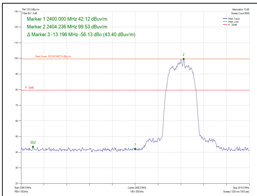
Figure 54 - GFSK/4DH5- 2404 MHz – Band Edge Frequency 2400.0 MHz (Plot should show P- 30dB limit in place of P- 20dB)
