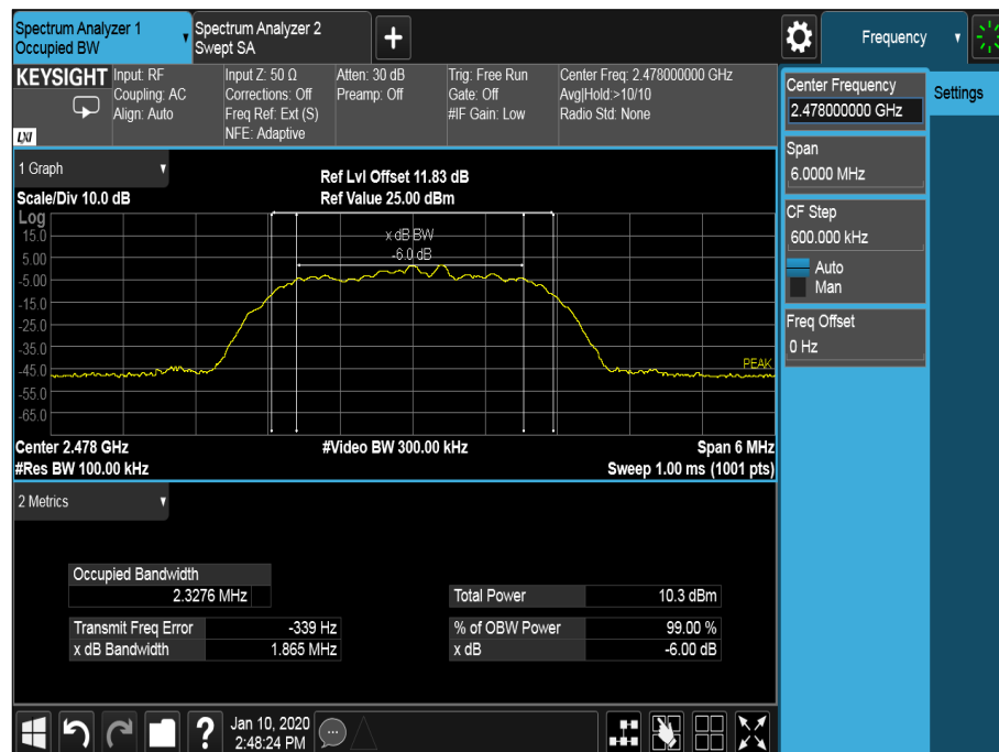
Figure 27 - 2478 MHz – Emission Bandwidth
