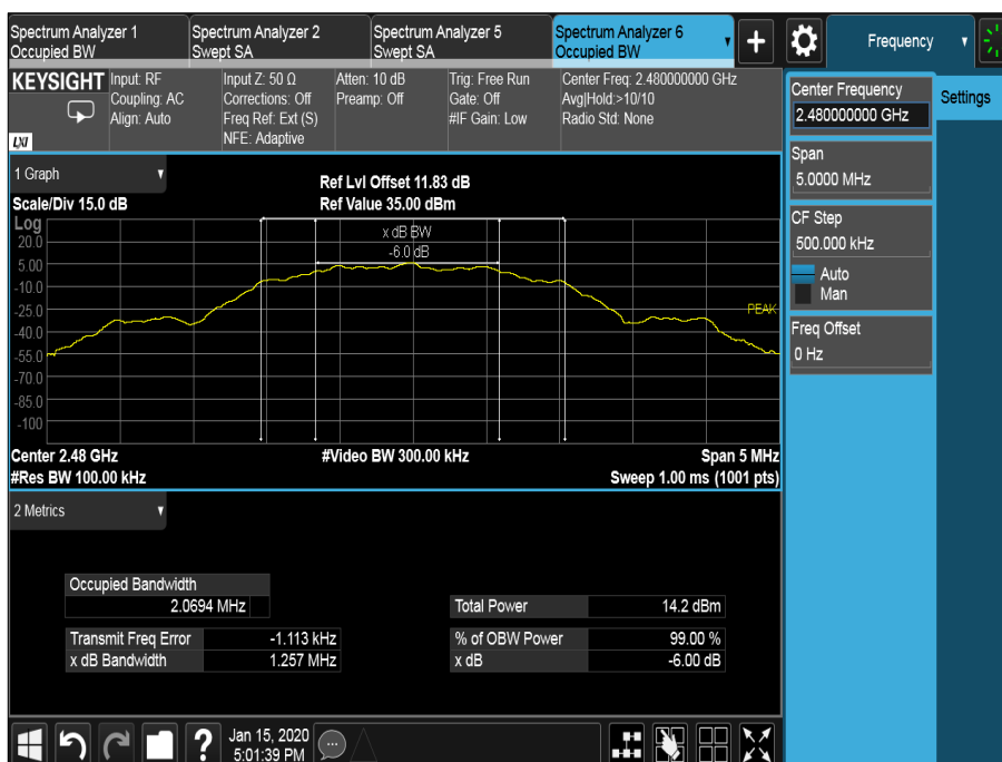
Figure 24 - 2480 MHz – Emission Bandwidth
