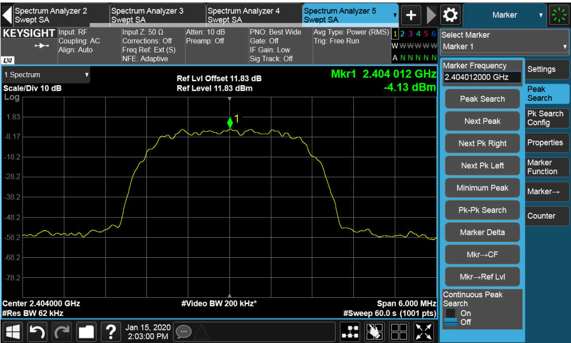
Figure 10 – 2404 MHz
