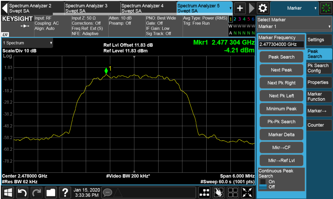
Figure 12 – 2478 MHz
