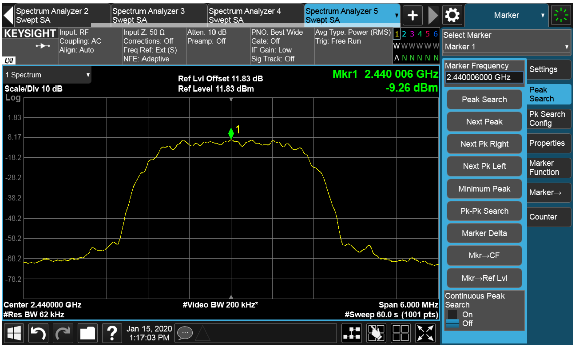
Figure 8 – 2440 MHz
