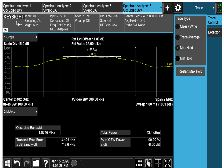
Figure 19 - 2402 MHz – Emission Bandwidth
