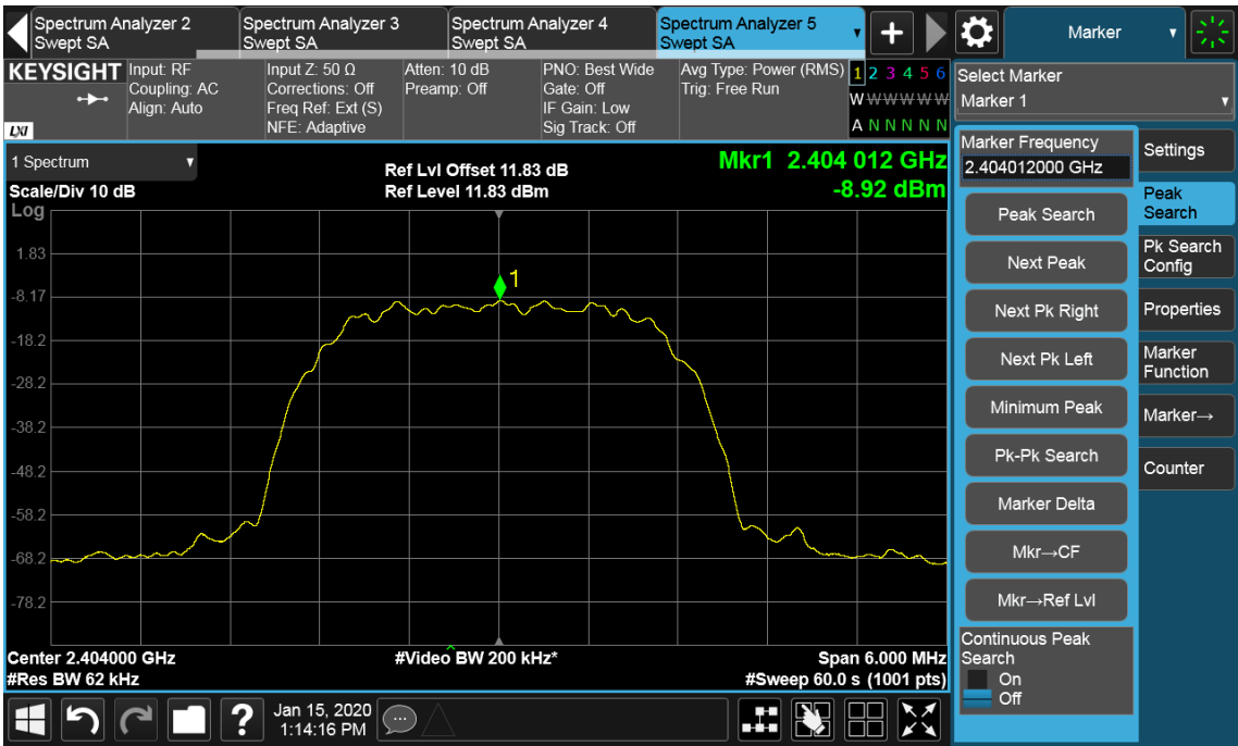
Figure 7 – 2404 MHz
