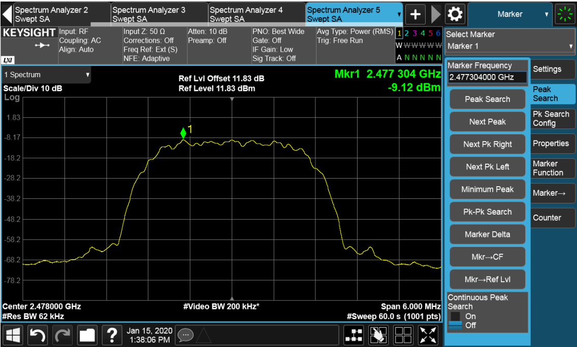
Figure 9 – 2478 MHz
