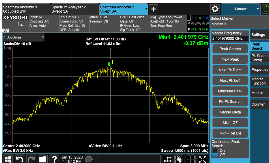
Figure 1 – 2402 MHz
