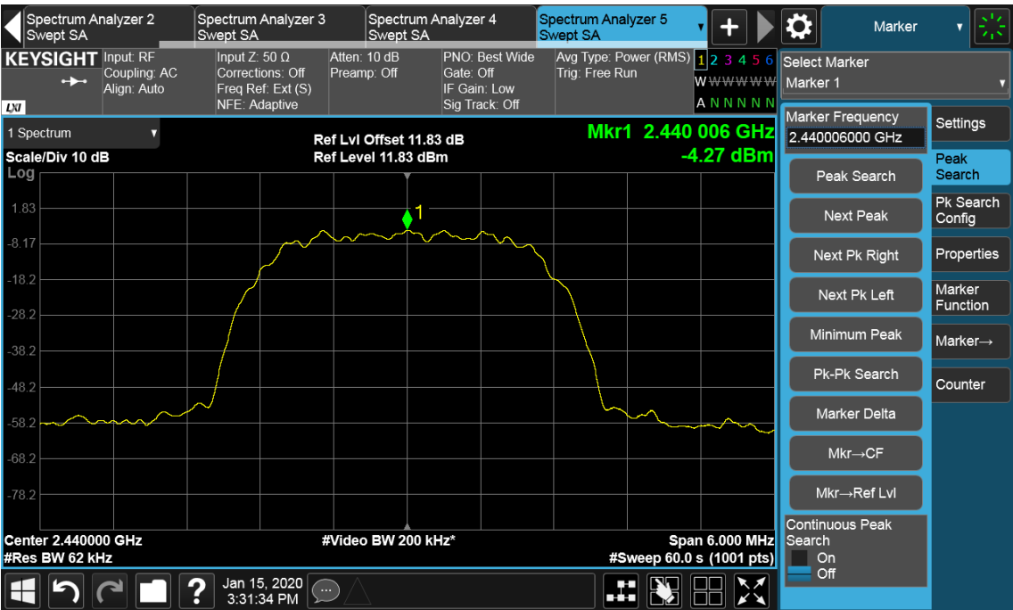
Figure 11 – 2440 MHz
