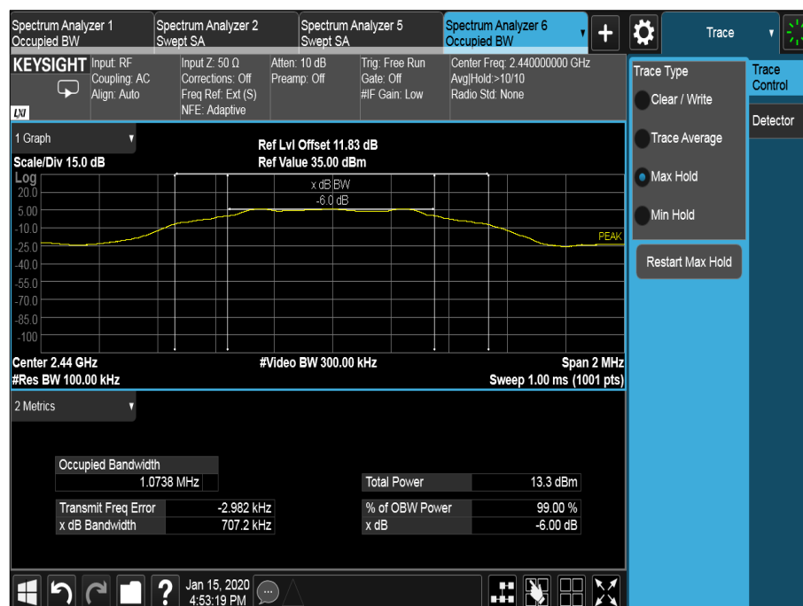
Figure 20 - 2440 MHz – Emission Bandwidth
