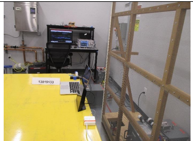
AC LINE CONDUCTED WITH AC ADAPTER (BACK)
