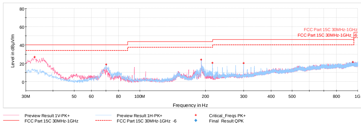
Plot 7-41. Radiated Spurious Plot Below 1GHz (GFSK ePA – Ch.39, with AC/DC Adapter)
