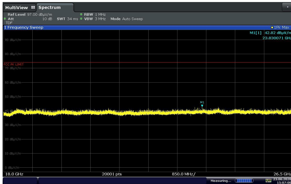
Plot 7-25. Radiated Spurious Emissions Above 18GHz (1Mbps ePA – Ch. 19, Ant. Pol. V)
