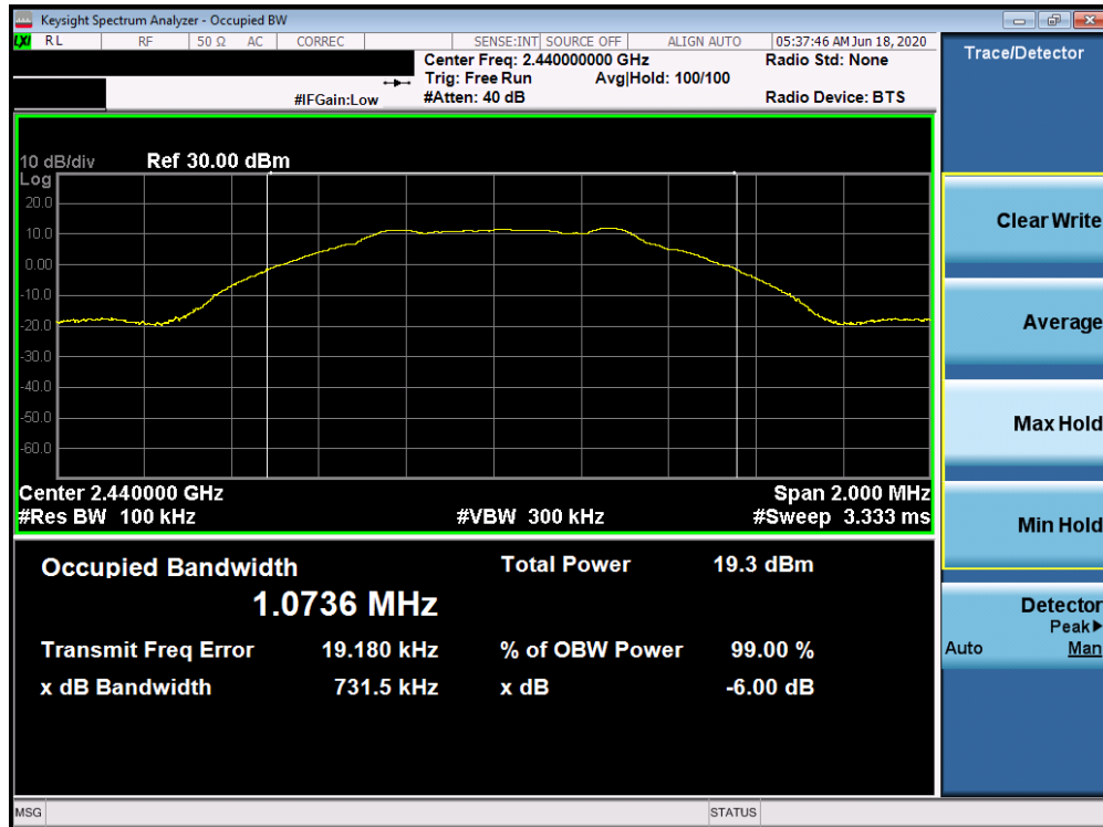
Plot 7-5. 6dB Bandwidth Plot (Bluetooth (LE), 1Mbps, iPA – Ch. 19)
