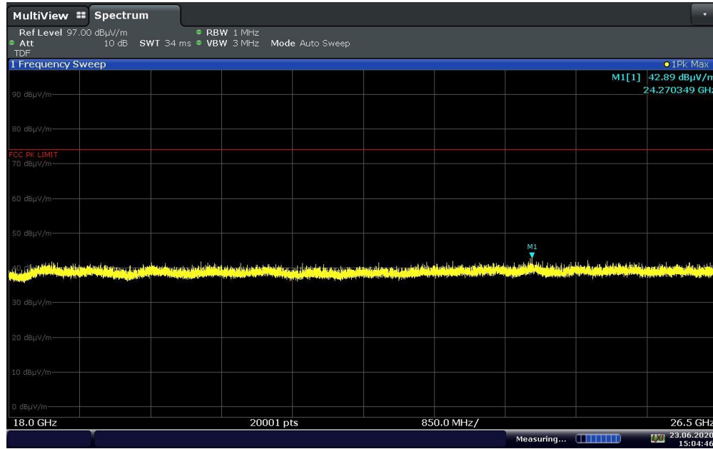
Plot 7-24. Radiated Spurious Emissions Above 18GHz (1Mbps ePA – Ch. 19, Ant. Pol. H)
