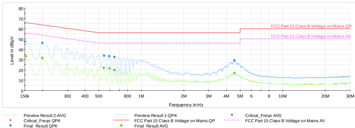
Plot 7-29. AC Line Conducted Plot with Bluetooth LE (L1, ePA - Ch.19, with AC/DC Adapter)
