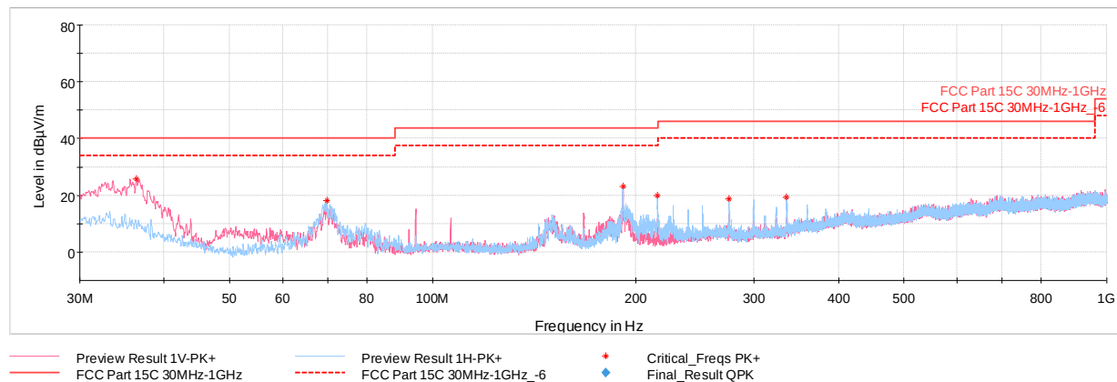
Plot 7-28. Radiated Spurious Emissions below 1GHz (1Mbps ePA - Ch.19, with AC/DC Adapter)
