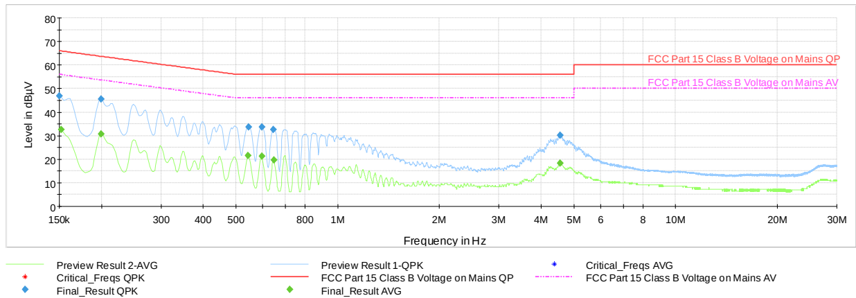
Plot 7-30. AC Line Conducted Plot with Bluetooth LE (N, ePA - Ch.19 with AC/DC Adapter)
