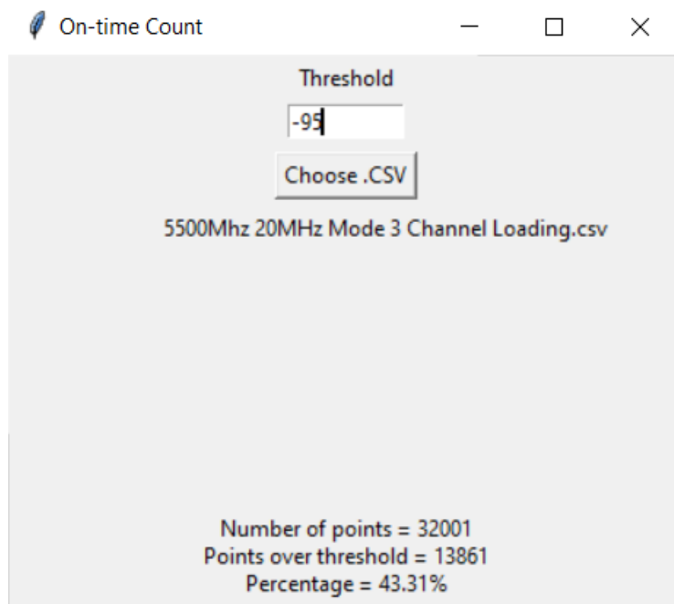
Figure 9-14. 5500MHz - Channel Loading Calculation - Mode 3 (20MHz)
