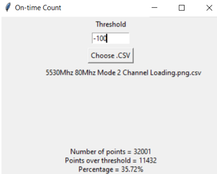
Figure 9-12. 5530MHz - Channel Loading Calculation - Mode 2 (80MHz)
