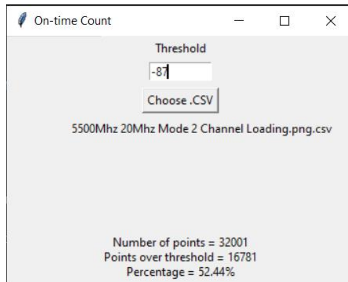
Figure 9-8. 5500MHz - Channel Loading Calculation - Mode 2 (20MHz)
