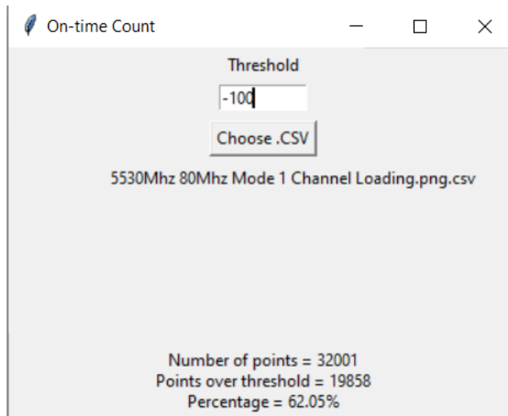
Figure 9-6. 5530MHz - Channel Loading Calculation - Mode 1 (80MHz)
