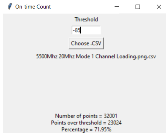
Figure 9-2. 5500MHz - Channel Loading Calculation - Mode 1 (20MHz)
