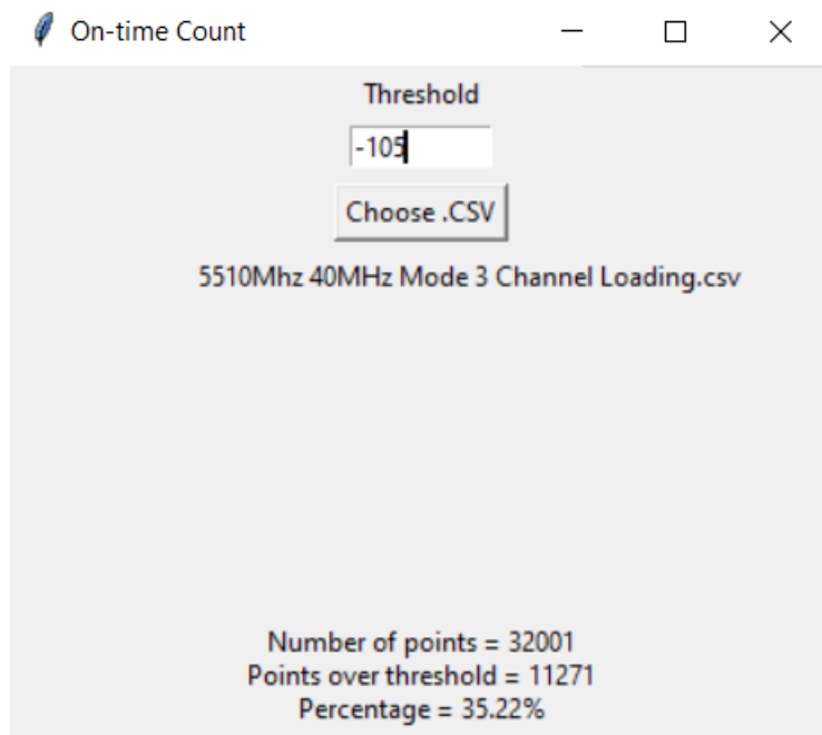
Figure 9-16 5510MHz - Channel Loading Calculation - Mode 3 (40MHz)
