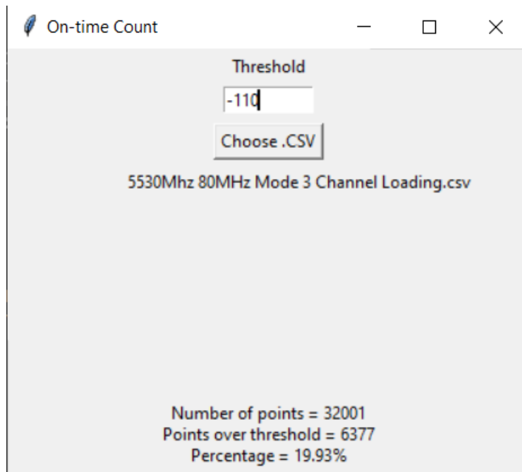
Figure 9-18. 5530MHz - Channel Loading Calculation - Mode 3 (80MHz)
