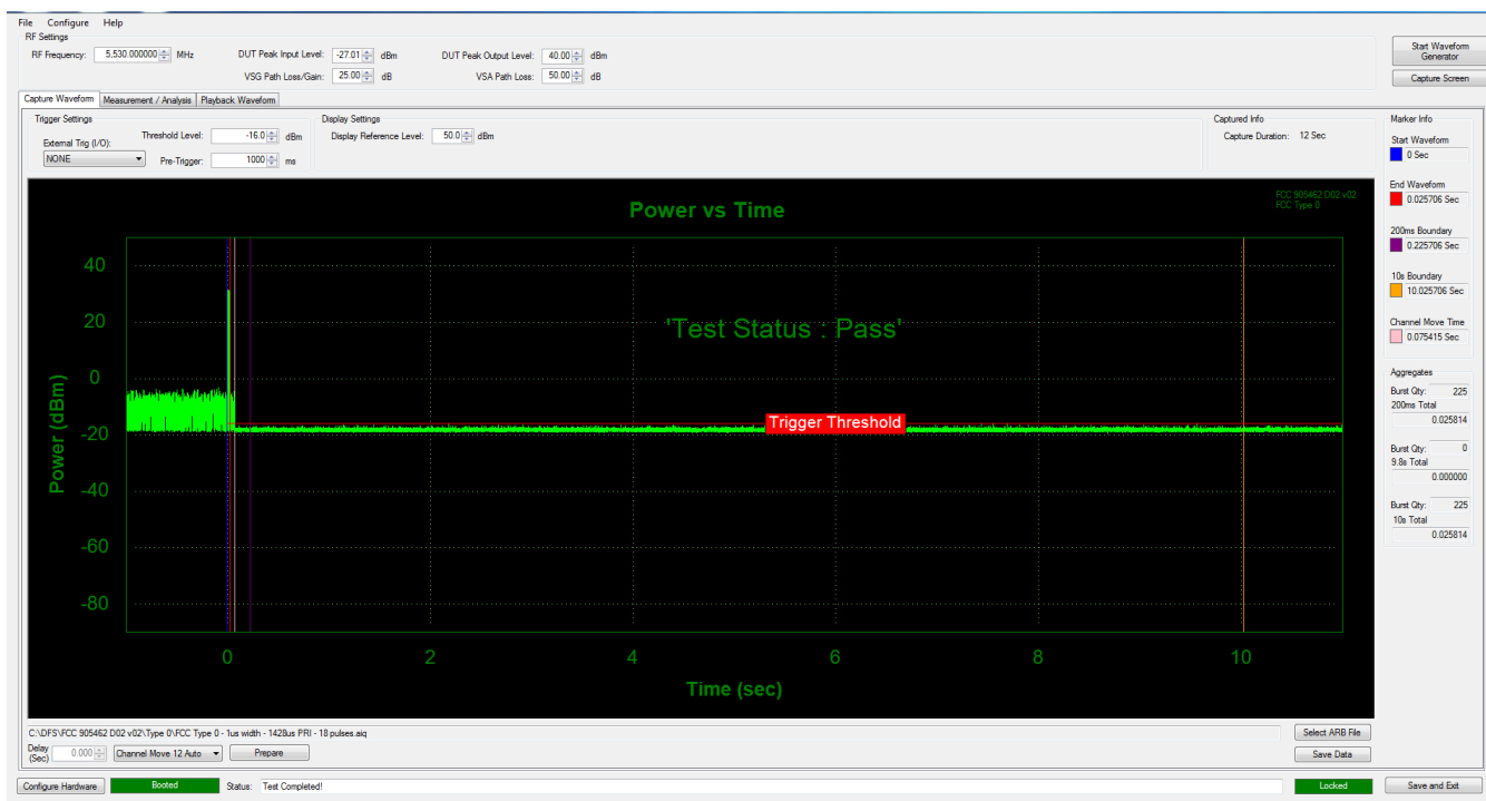
Figure 9-27. 5530MHz - Channel Move/ Closing Transmission Time - Mode 1 (80 MHz)
