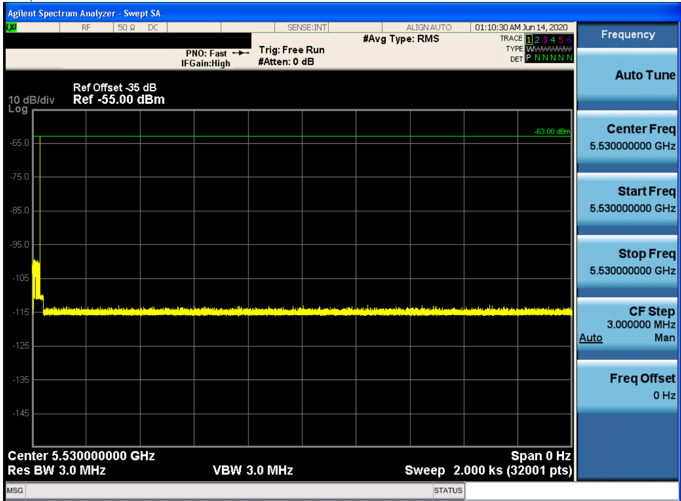
Figure 9-48. 5530MHz - Non-Occupancy Period (30 Minutes) - Mode 4 (80MHz)
