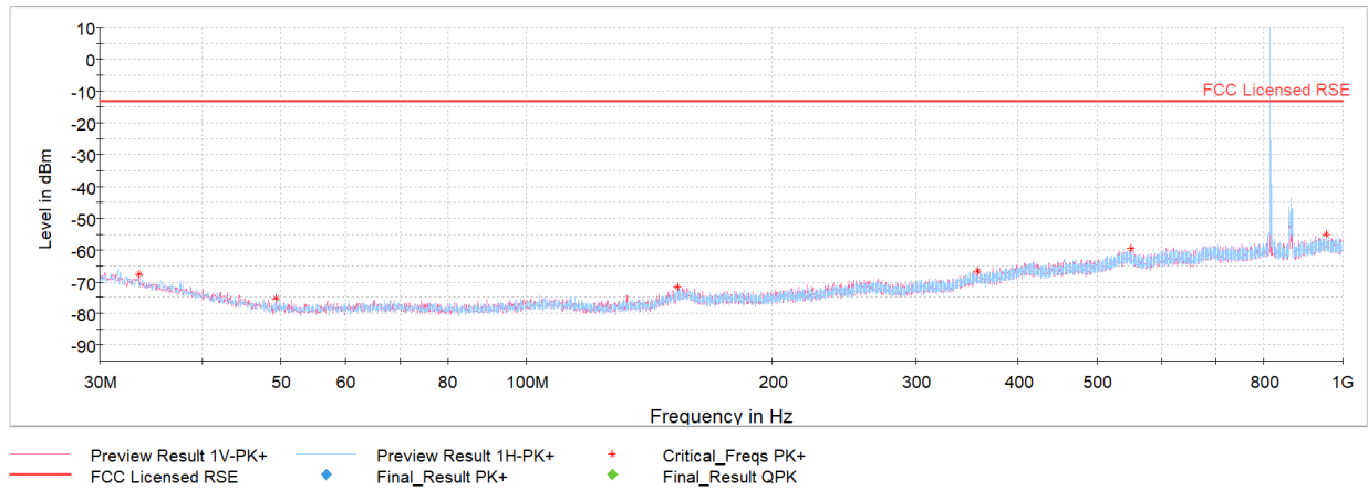
Plot 7-26. Radiated Spurious Plot Below 1GHz (Band 26)
