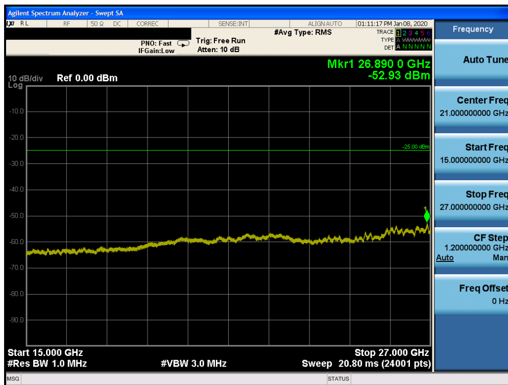
Plot 7-410. Conducted Spurious Plot (Band 7 – 20.0MHz QPSK – PCC 1/99 SCC 1/0 – Mid Channel)
