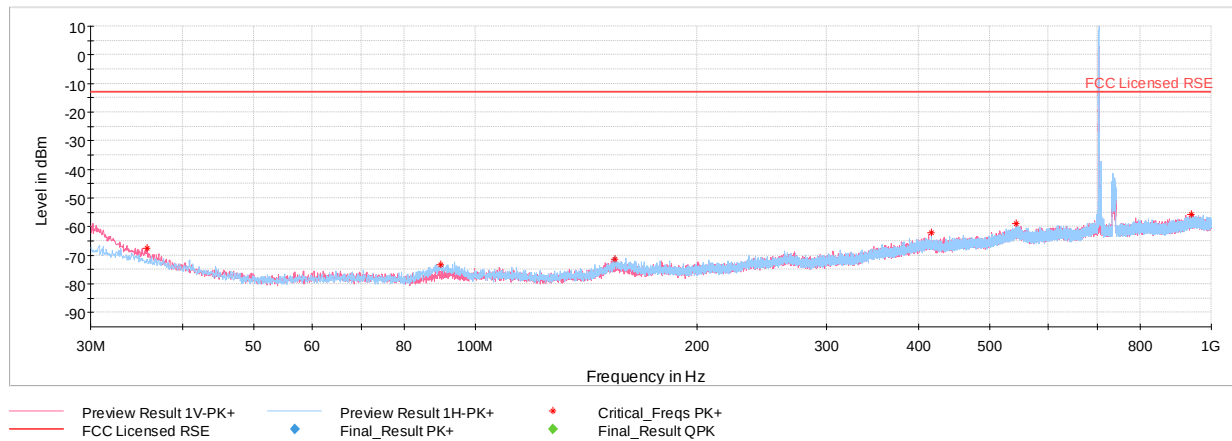
Plot 7-421. Radiated Spurious Plot below 1GHz (Band 13)
