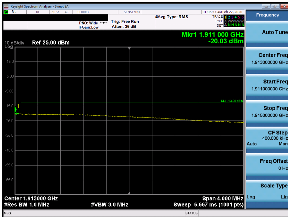
Plot 7-272. Upper Extended Band Edge Plot (Band 2 – 15.0MHz QPSK – RB Size 75)
