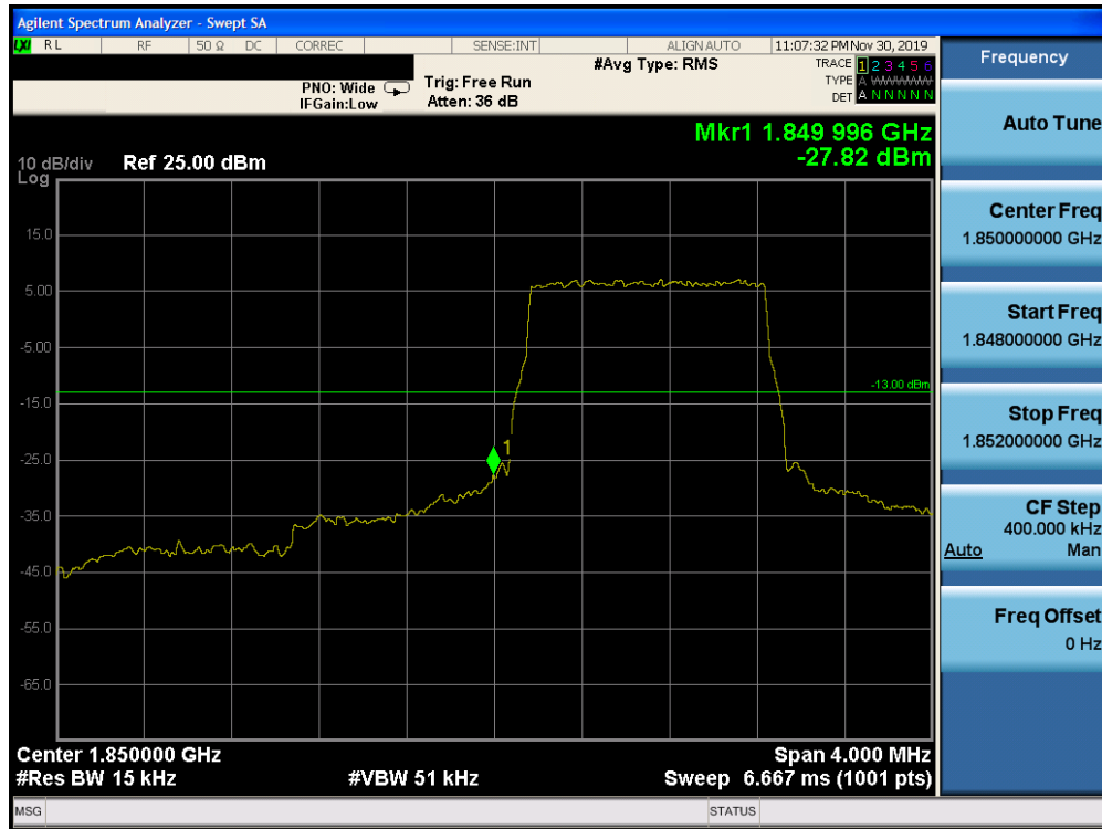
Plot 7-277. Lower Band Edge Plot (Band 25 – 1.4MHz QPSK – RB Size 6)
