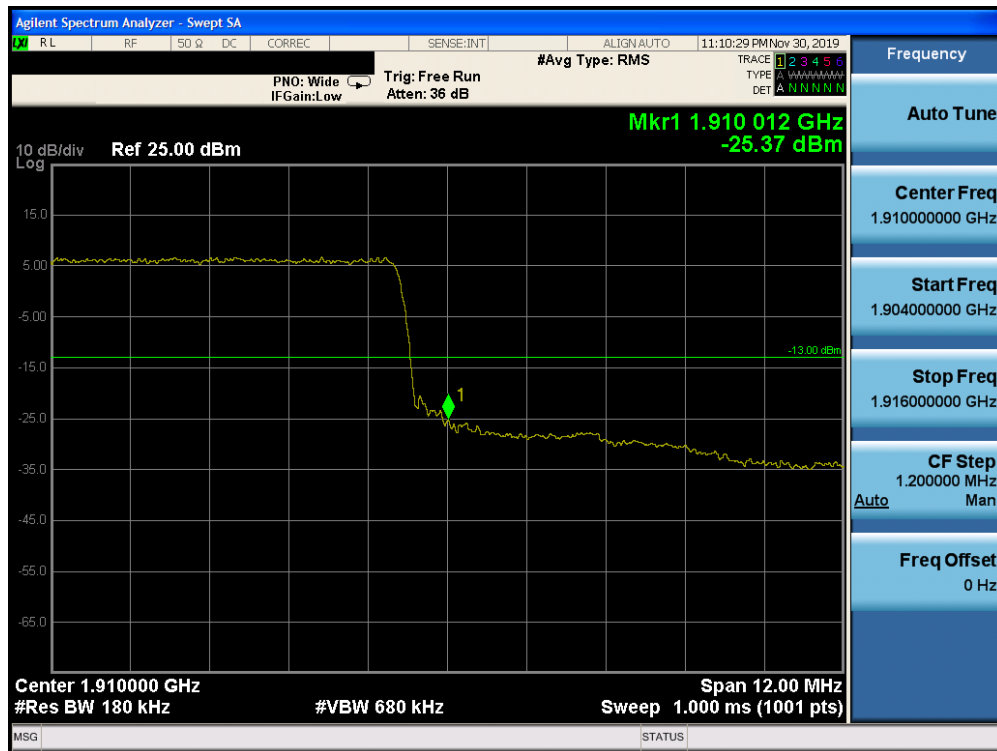
Plot 7-271. Upper Band Edge Plot (Band 2 – 15.0MHz QPSK – RB Size 75)
