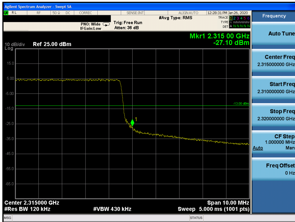
Plot 7-307. Upper Band Edge Plot (Band 30 - 10.0MHz QPSK - RB Size 50)
