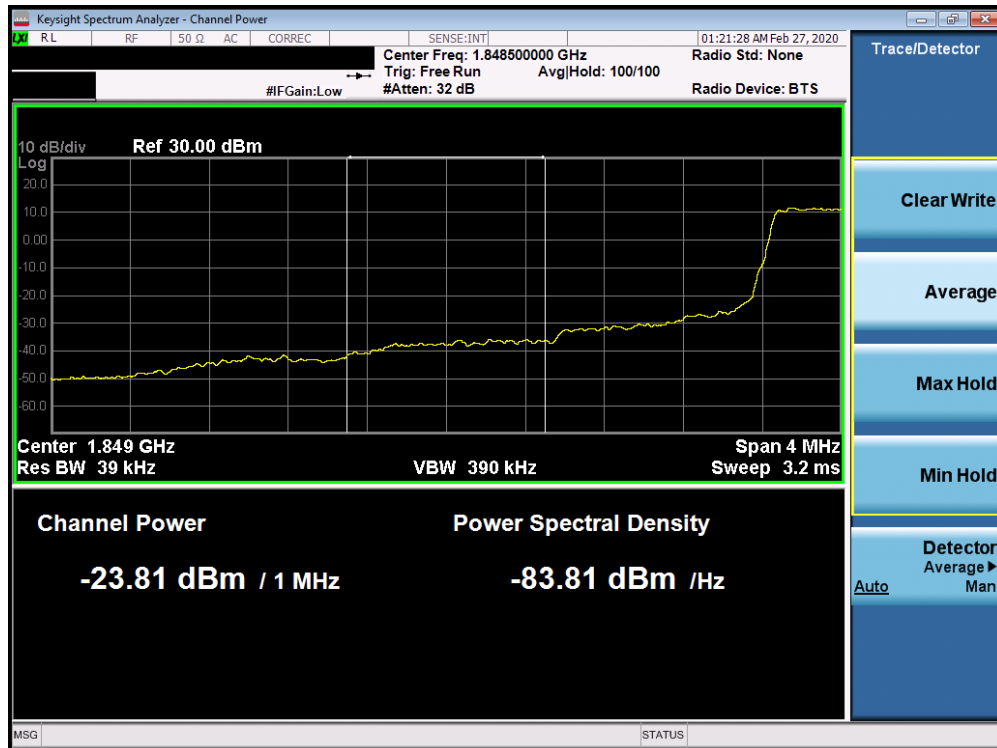
Plot 7-278. Lower Extended Band Edge Plot (Band 25 – 1.4MHz QPSK – RB Size 6)
