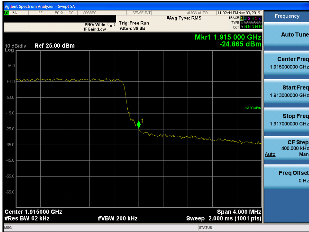
Plot 7-287. Upper Band Edge Plot (Band 25 – 5.0MHz QPSK – RB Size 25)
