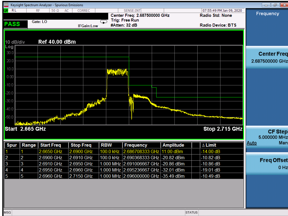
Plot 7-318. Upper ACP Plot (Band 41 – 5.0MHz QPSK – RB Size 25)
