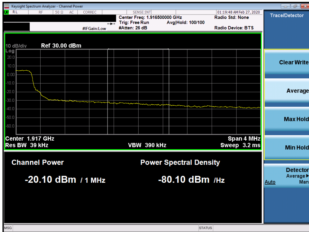
Plot 7-288. Upper Extended Band Edge Plot (Band 25 – 5.0MHz QPSK – RB Size 25)
