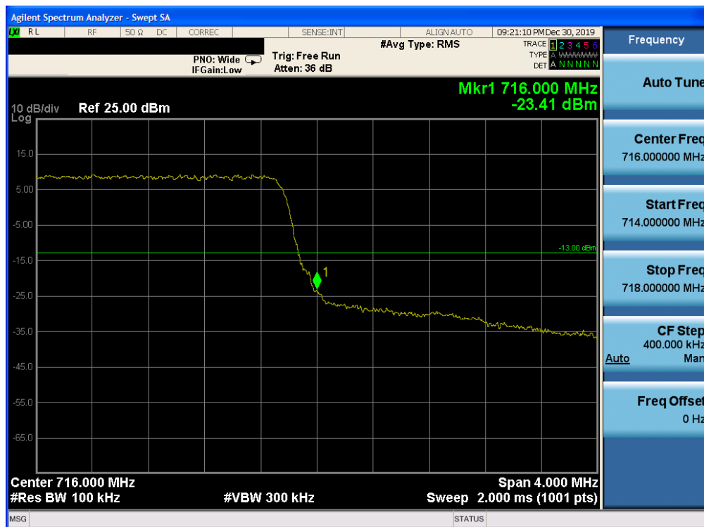
Plot 7-174. Upper Band Edge Plot (Band 12 – 5.0MHz QPSK – RB Size 25)
