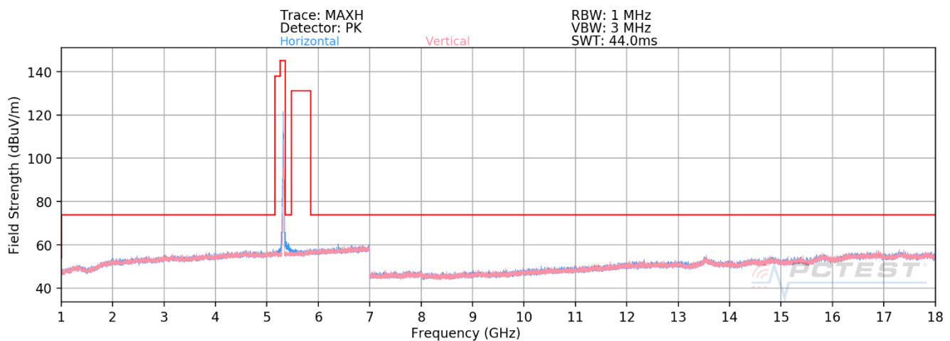
Plot 7-726. Radiated Spurious Plot above 1GHz SISO CORE 0 (802.11ax – U2A Ch. 64 – RU26)
