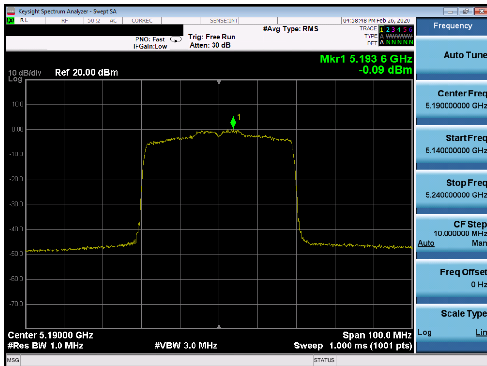
Plot 7-662. Power Spectral Density Plot ISCED CDD CORE 1 (40MHz BW 802.11ax – RU484 (UNII Band 1) – Ch. 38)
