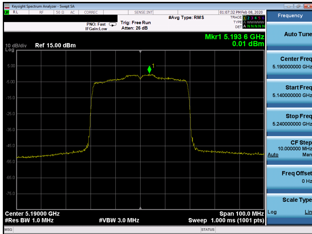
Plot 7-661. Power Spectral Density Plot ISCED CDD CORE 0 (40MHz BW 802.11ax – RU484 (UNII Band 1) – Ch. 38)
