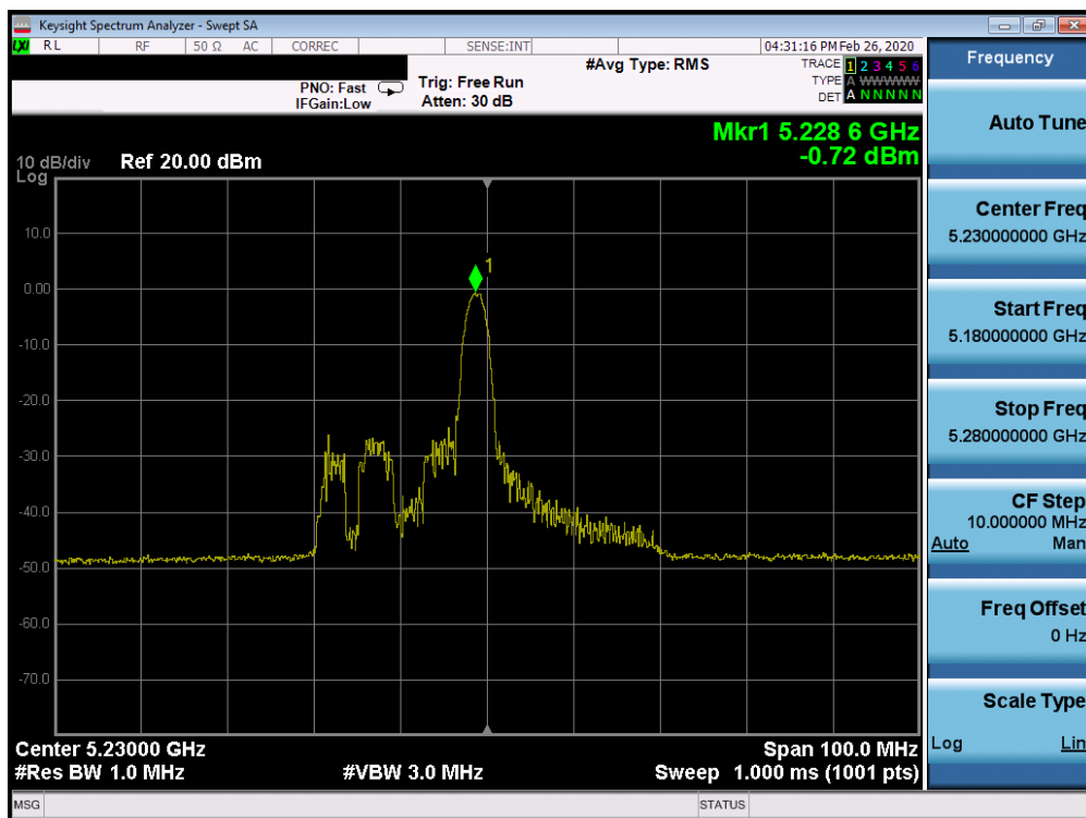
Plot 7-658. Power Spectral Density Plot ISD CDD CORE 1 (40MHz BW 802.11ax Index 8 – RU26 (UNII Band 1) – Ch. 46)
