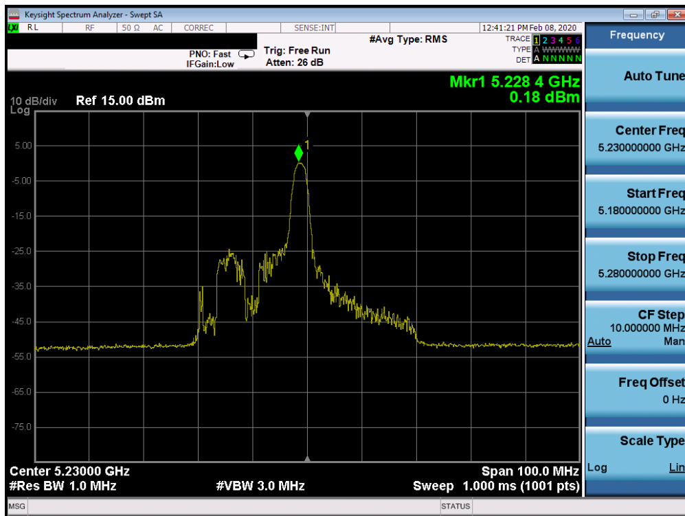
Plot 7-657. Power Spectral Density Plot ISD CDD CORE 0 (40MHz BW 802.11ax Index 8 – RU26 (UNII Band 1) – Ch. 46)
