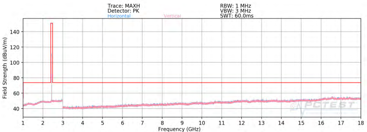
Plot 7-82. Radiated Spurious Plot Above 1GHz Ant 4a (4Mbps, HDR4 ePA – Ch. 38, Ant. Pol. H & V)
