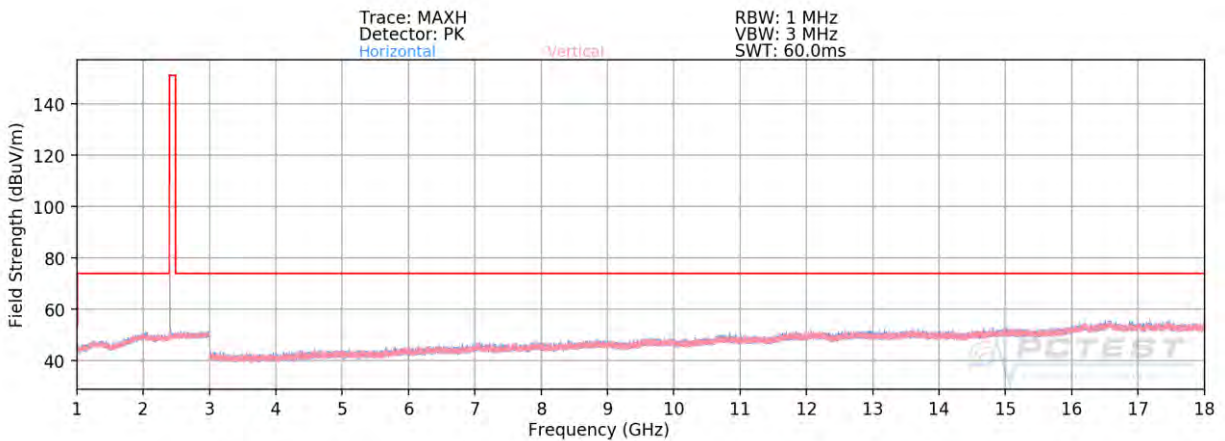
Plot 7-81. Radiated Spurious Plot Above 1GHz Ant 4a (4Mbps, HDR4 ePA – Ch. 1, Ant. Pol. H & V)
