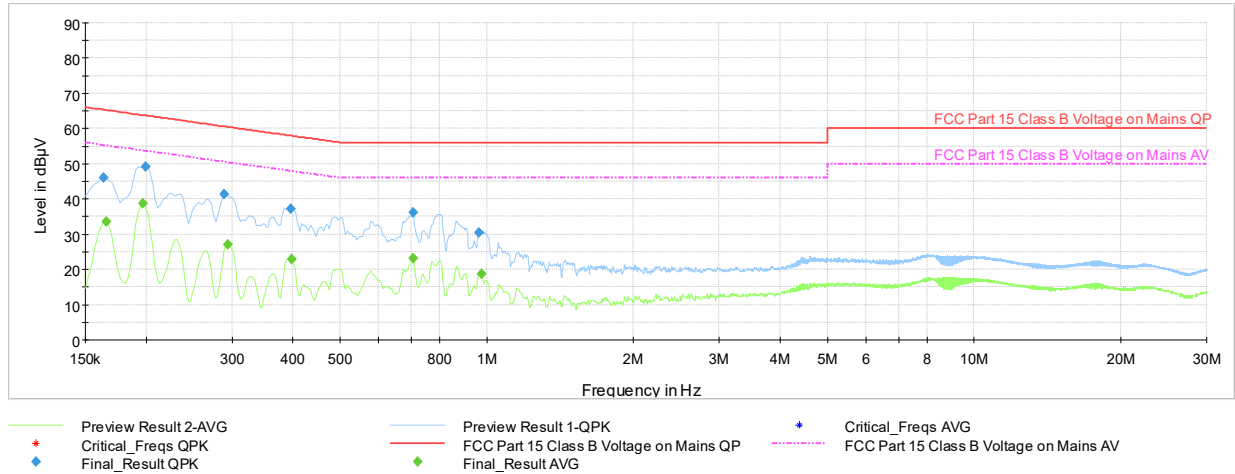
Plot 7-106. Line Conducted Plot with Bluetooth HDR (N, 4Mbps ePA – Ch.38 with AC/DC Adapter)
