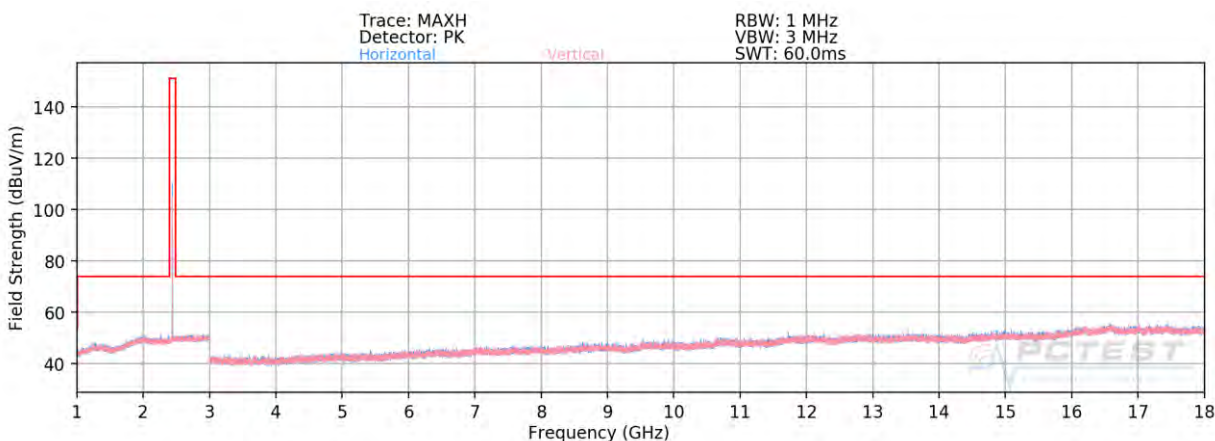
Plot 7-85. Radiated Spurious Plot Above 1GHz Ant 2a (4Mbps, HDR4 ePA – Ch. 38, Ant. Pol. H & V)
