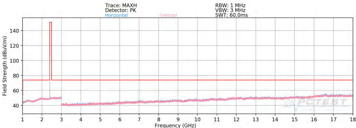
Plot 7-84. Radiated Spurious Plot Above 1GHz Ant 2a (4Mbps, HDR4 ePA – Ch. 1, Ant. Pol. H & V)
