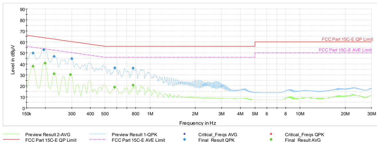
Plot 7-105. Line Conducted Plot with Bluetooth HDR (L1, 4Mbps ePA – Ch.38 with AC/DC Adapter)
