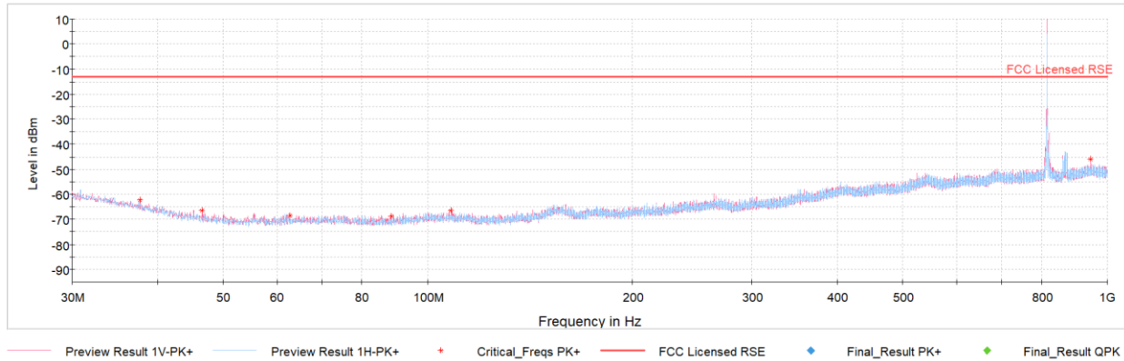
Plot 7-26. Radiated Spurious Plot Below 1GHz (Band 26)
