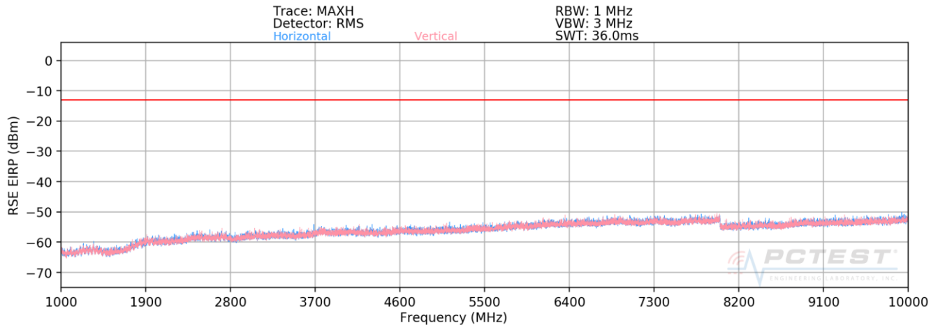
Plot 7-27. Radiated Spurious Plot Above 1GHz (Band 26)
