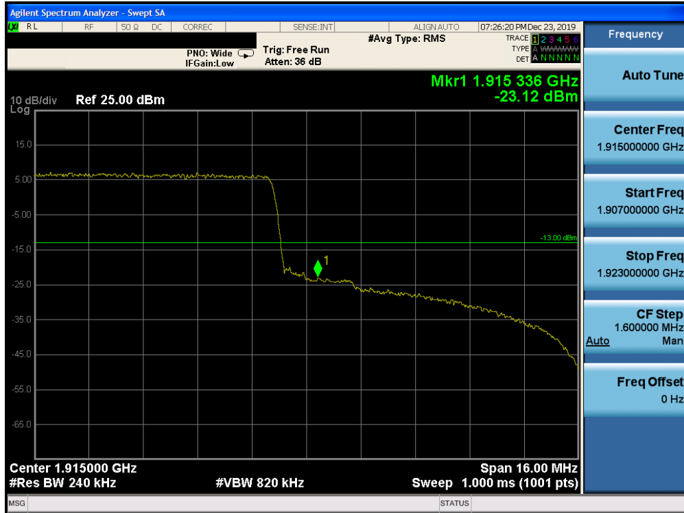
Plot 7-299. Upper Band Edge Plot (Band 25 – 20.0MHz QPSK – RB Size 100)
