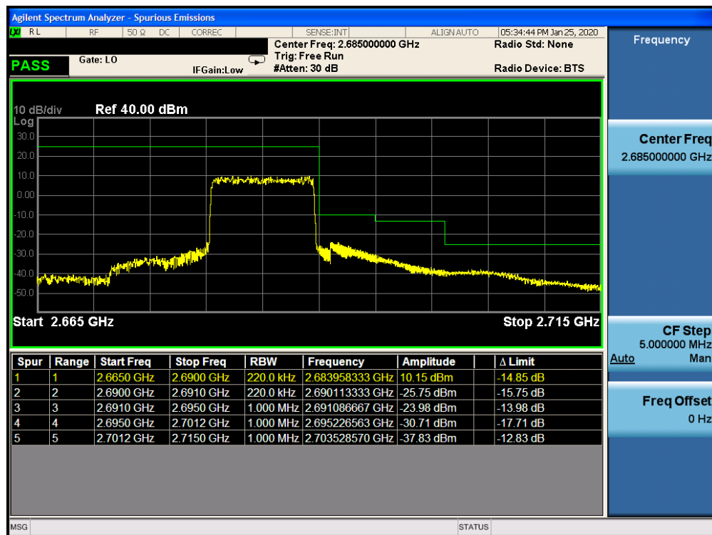
Plot 7-320. Upper ACP Plot (Band 41 – 10.0MHz QPSK – RB Size 50)
