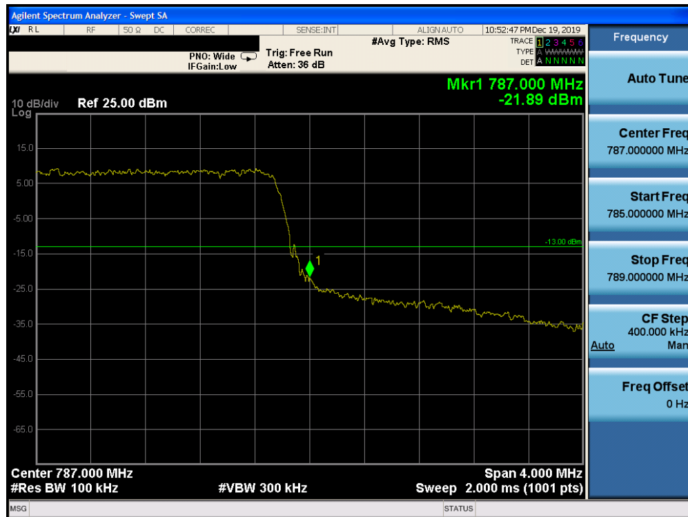
Plot 7-183. Upper Band Edge Plot (Band 13 – 5.0MHz QPSK – RB Size 25)
