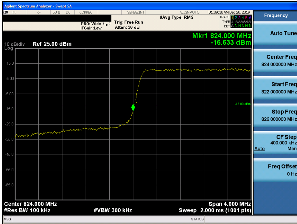
Plot 7-199. Lower Band Edge Plot (Band 5 – 3.0MHz QPSK – RB Size 15)
