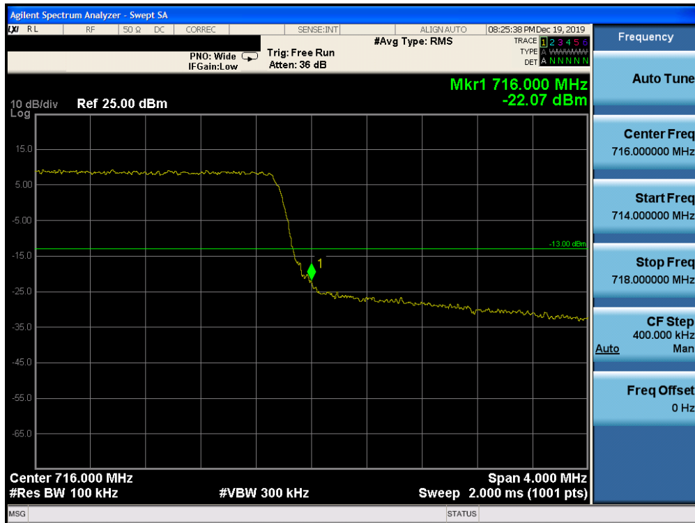
Plot 7-178. Upper Band Edge Plot (Band 17 – 5.0MHz QPSK – RB Size 25)
