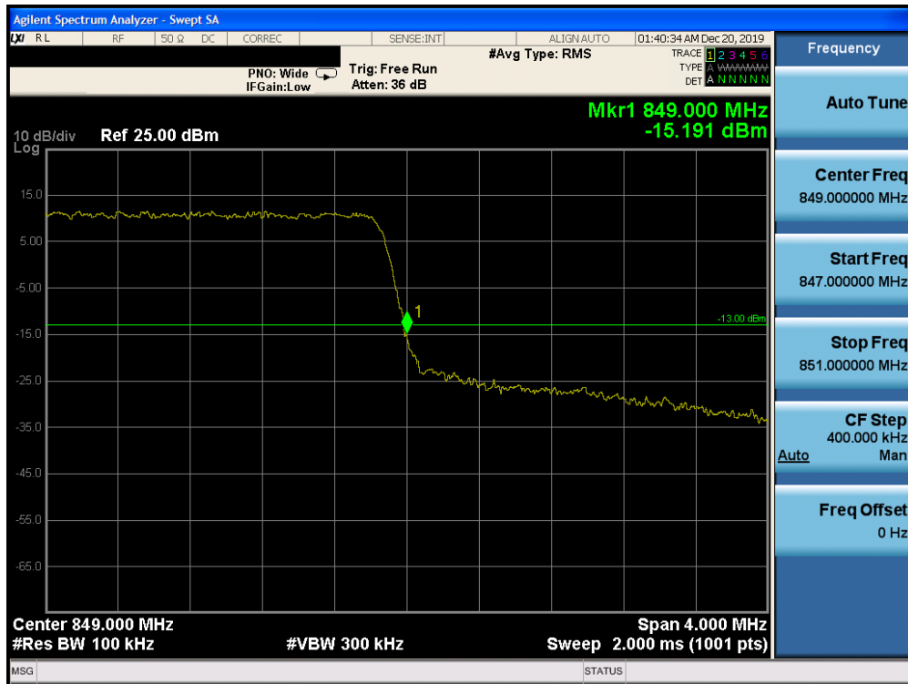
Plot 7-200. Upper Band Edge Plot (Band 5 – 3.0MHz QPSK – RB Size 15)
