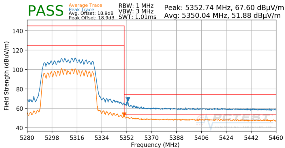
Plot 7-901. Radiated Upper Band Edge Plot CDD (Peak & Average – UNII Band 2A – RU484)
