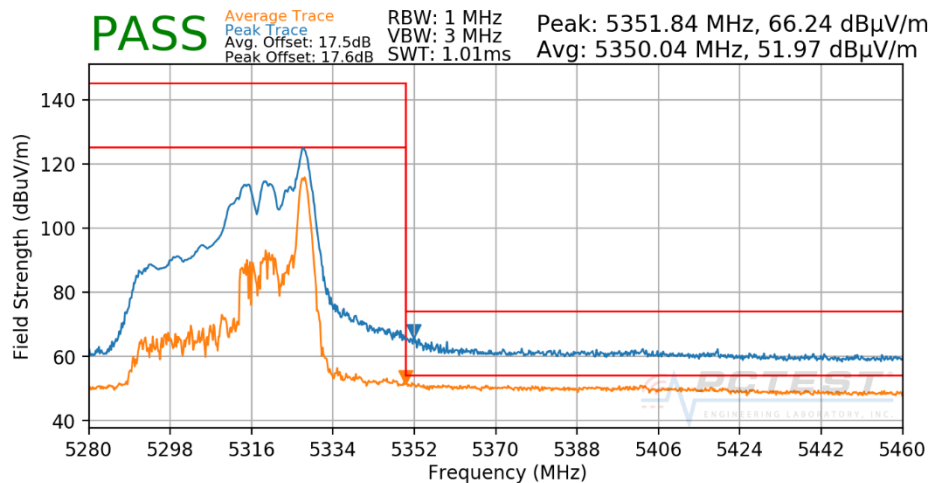
Plot 7-893. Radiated Upper Band Edge Plot CDD (Peak & Average – UNII Band 2A – RU26)
