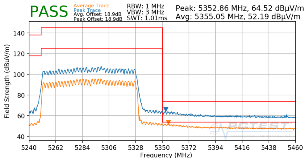
Plot 7-913. Radiated Upper Band Edge Plot CDD (Peak & Average – UNII Band 2A – RU996)
