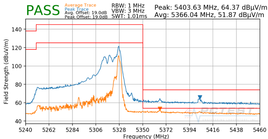
Plot 7-908. Radiated Upper Band Edge Plot CDD (Peak & Average – UNII Band 2A – RU26)
