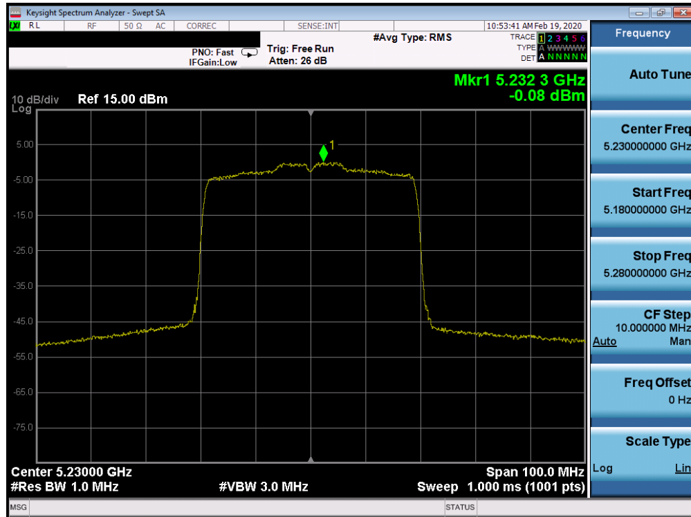
Plot 7-663. Power Spectral Density Plot ISCED CDD CORE 0 (40MHz BW 802.11ax – RU484 (UNII Band 1) – Ch. 46)
