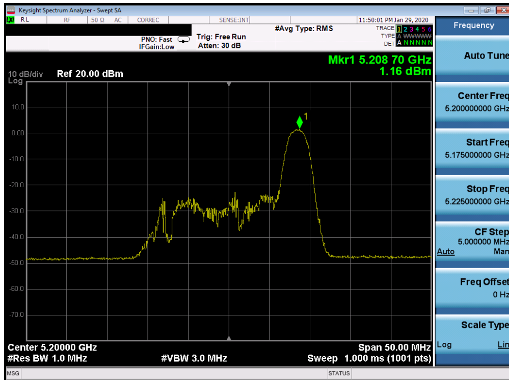
Plot 7-636. Power Spectral Density Plot ISD CDD CORE 1 (20MHz BW 802.11ax Index 8- RU26 (UNII Band 1) – Ch. 40)
