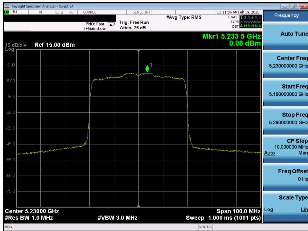
Plot 7-664. Power Spectral Density Plot ISCED CDD CORE 1 (40MHz BW 802.11ax – RU484 (UNII Band 1) – Ch. 46)
