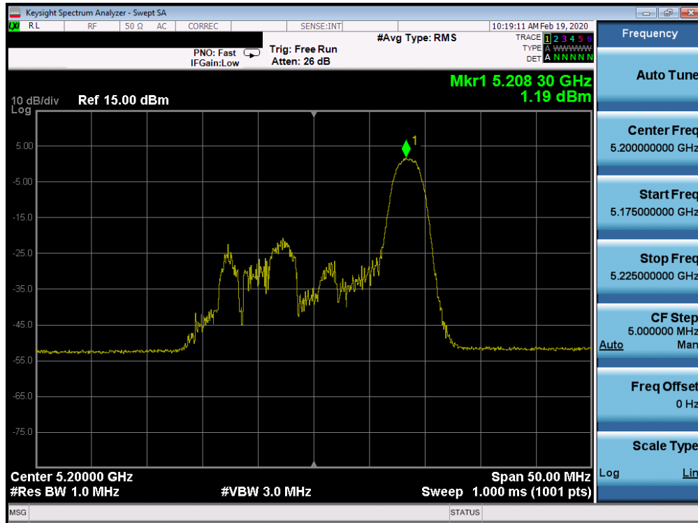
Plot 7-635. Power Spectral Density Plot ISD CDD CORE 0 (20MHz BW 802.11ax Index 8- RU26 (UNII Band 1) – Ch. 40)
