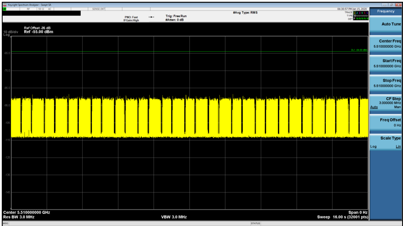
Figure 9-21. 5510MHz - Channel Loading - Mode 4 (40MHz)
