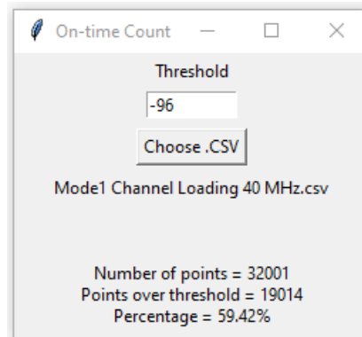
Figure 9-4 5510MHz - Channel Loading Calculation - Mode 1 (40MHz)
