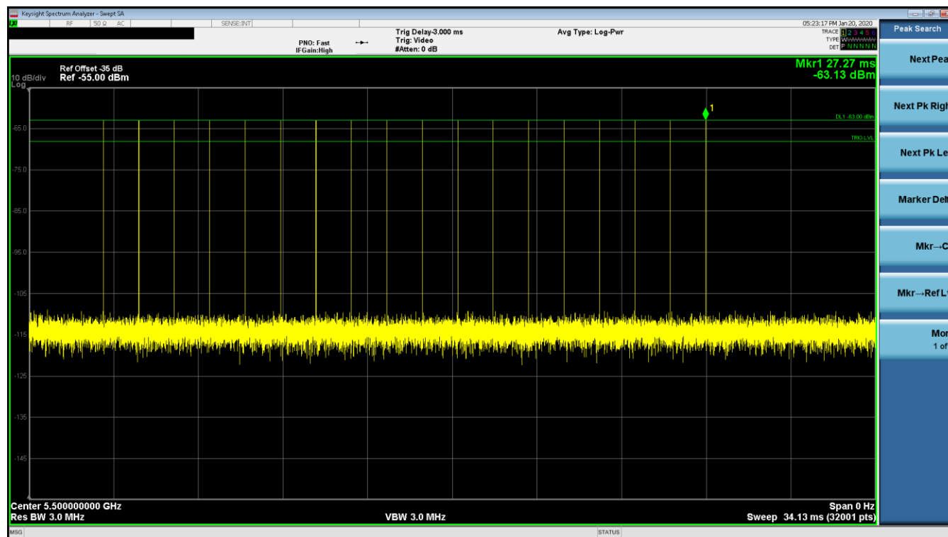
Figure 7-3. 5500MHz – Radar Pulse Type 0 (20MHz)
