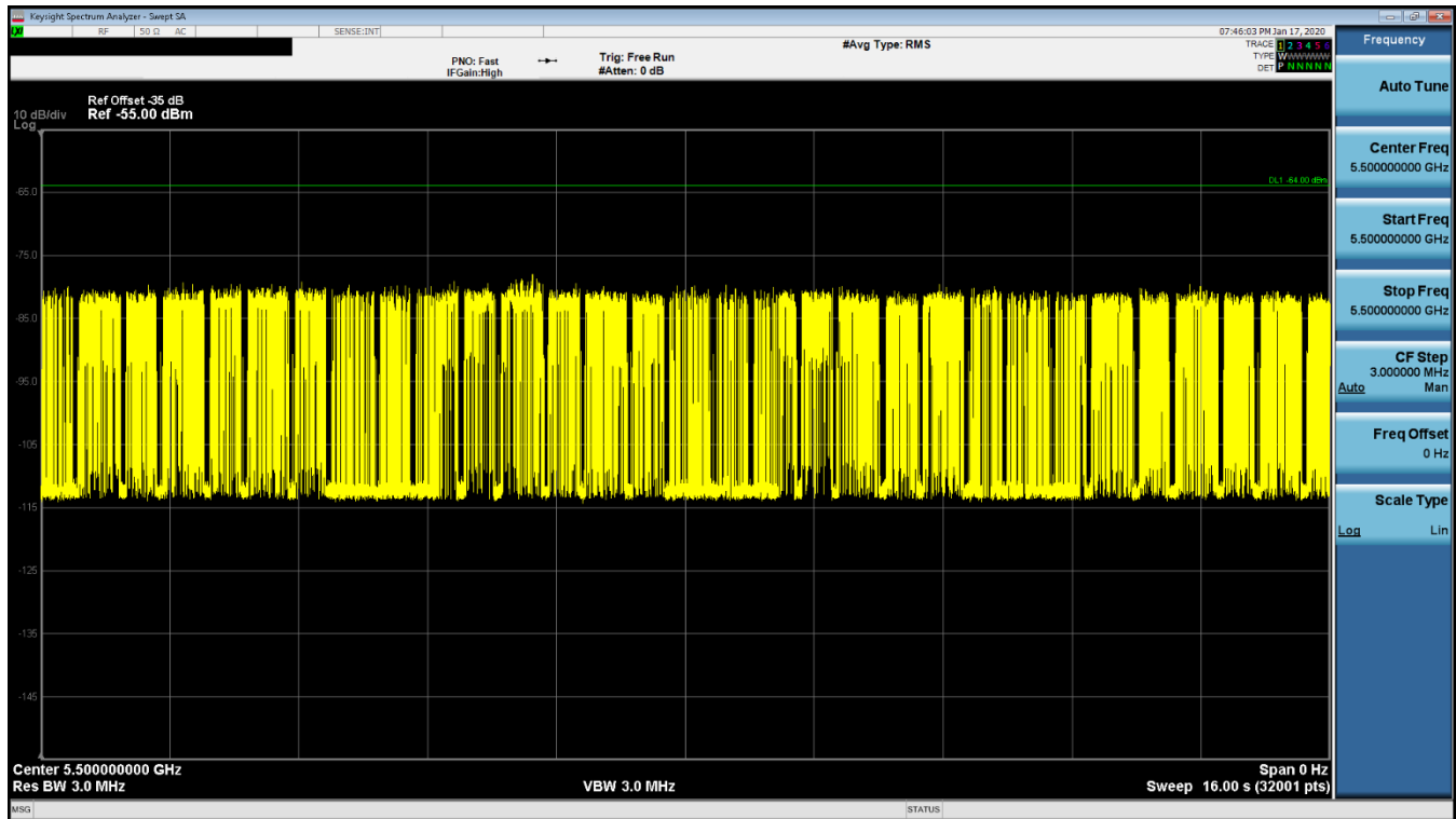
Figure 9-7. 5500MHz - Channel Loading - Mode 2 (20MHz)
