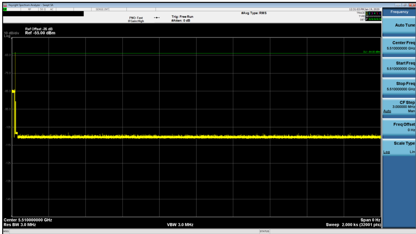
Figure 9-38. 5510MHz - Non-Occupancy Period (30 Minutes) - Mode 1 (40MHz)
