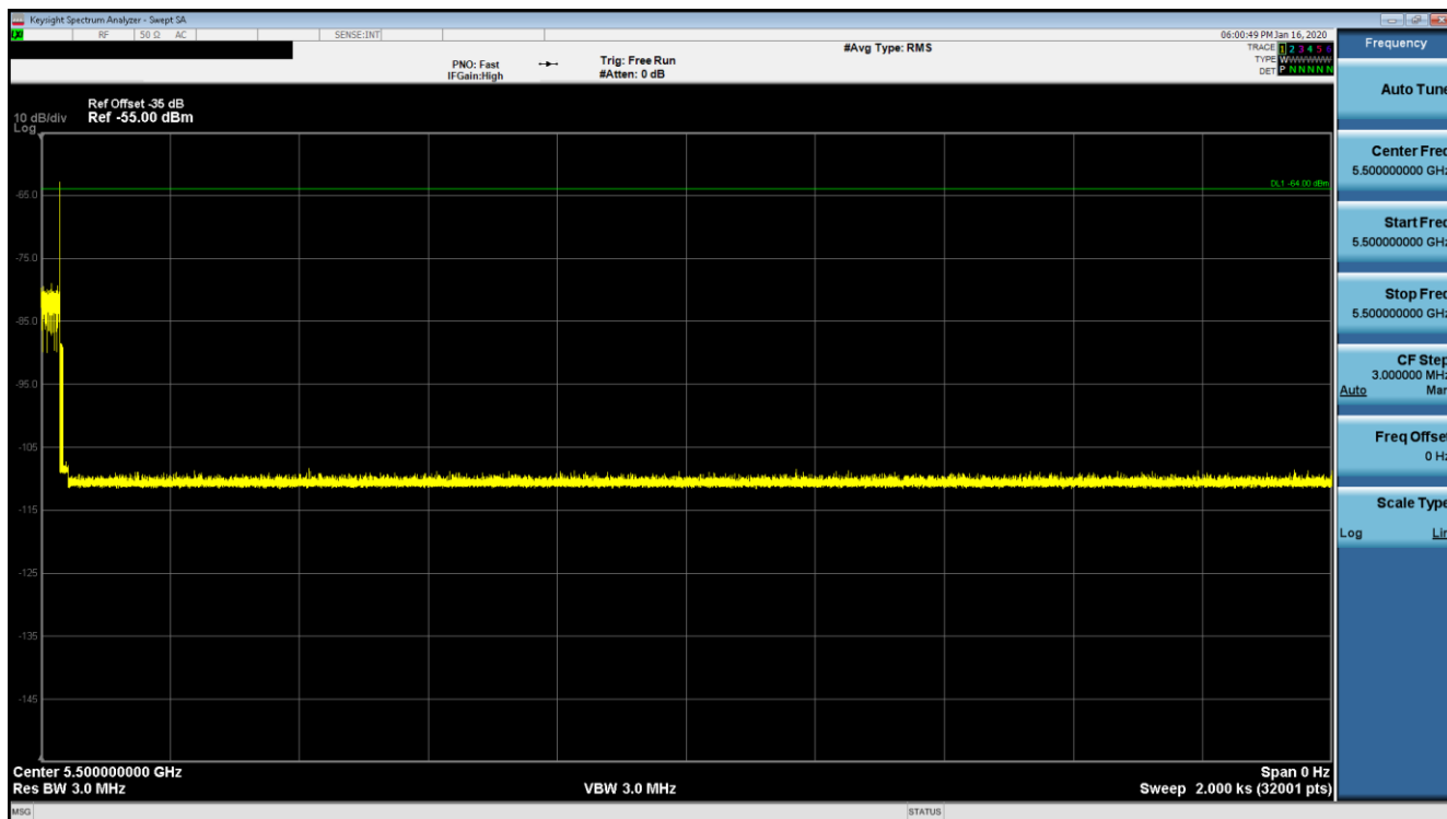
Figure 9-43. 5500MHz - Non-Occupancy Period (30 Minutes) - Mode 3 (20MHz)
