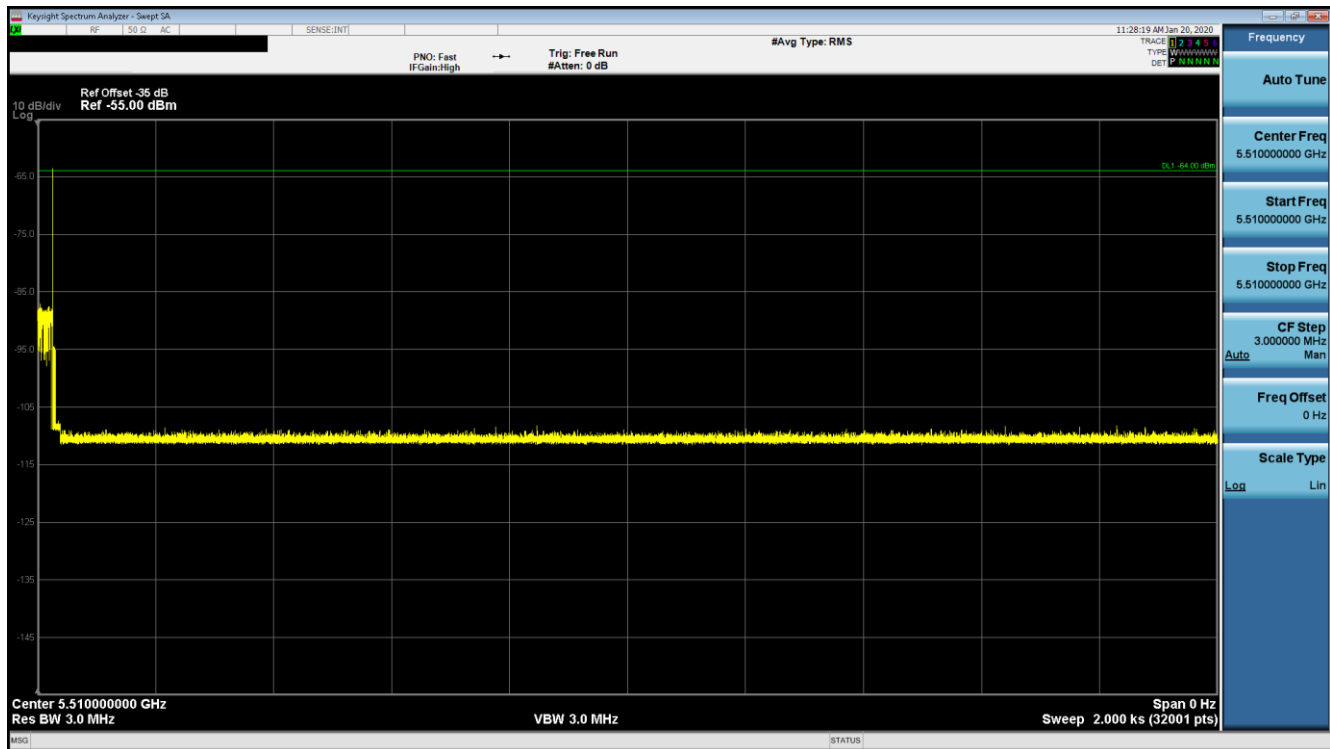
Figure 9-44. 5510MHz - Non-Occupancy Period (30 Minutes) - Mode 3 (40MHz)
