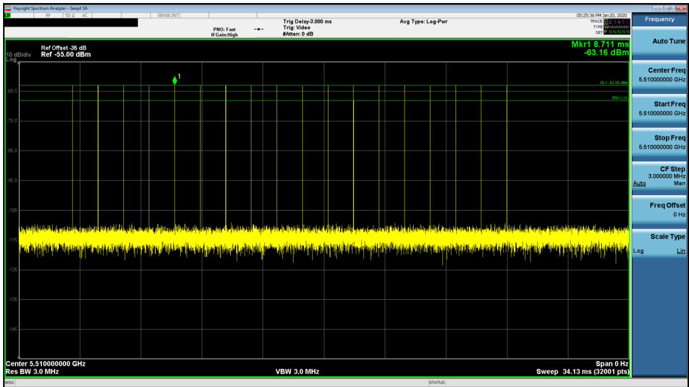
Figure 7-4. 5510MHz – Radar Pulse Type 0 (40MHz)
