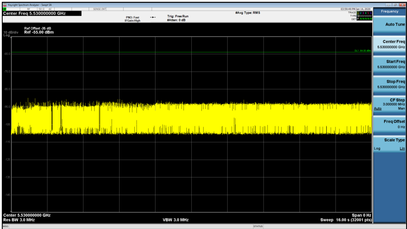
Figure 9-5. 5530MHz - Channel Loading - Mode 1 (80MHz)
