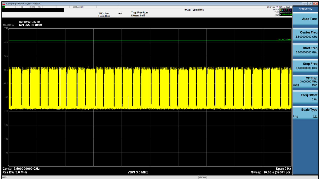
Figure 9-19. 5500 MHz - Channel Loading - Mode 4 (20MHz)
