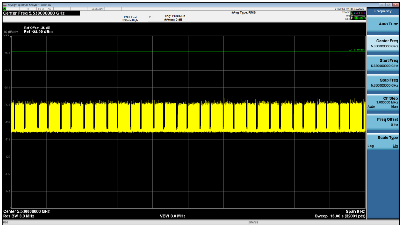
Figure 9-17. 5530MHz - Channel Loading - Mode 3 (80MHz)
