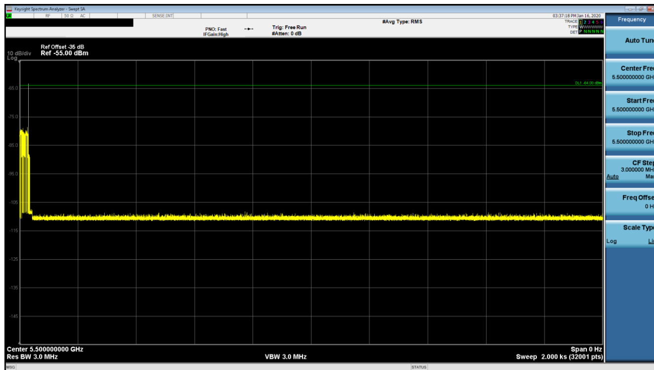
Figure 9-37. 5500MHz - Non-Occupancy Period (30 Minutes) - Mode 1 (20MHz)
