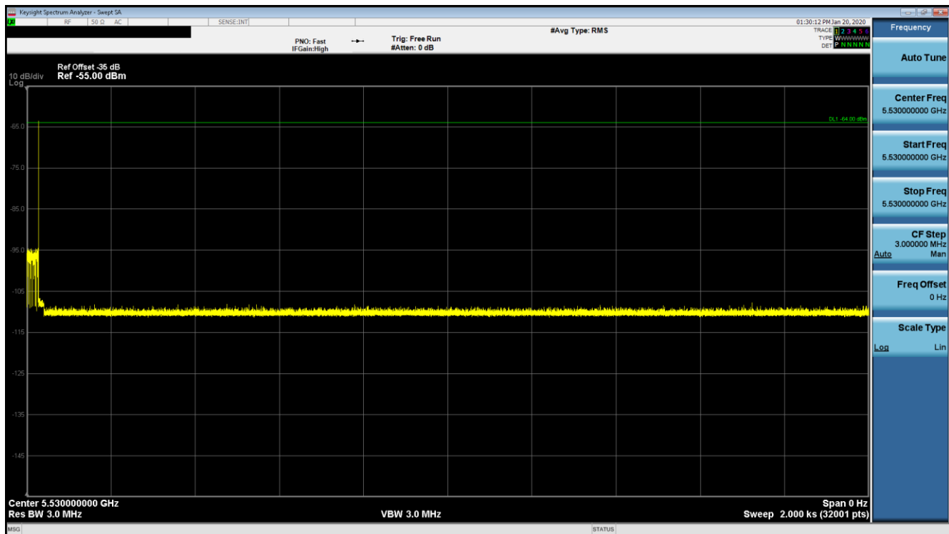
Figure 9-48. 5530MHz - Non-Occupancy Period (30 Minutes) - Mode 4 (80MHz)
