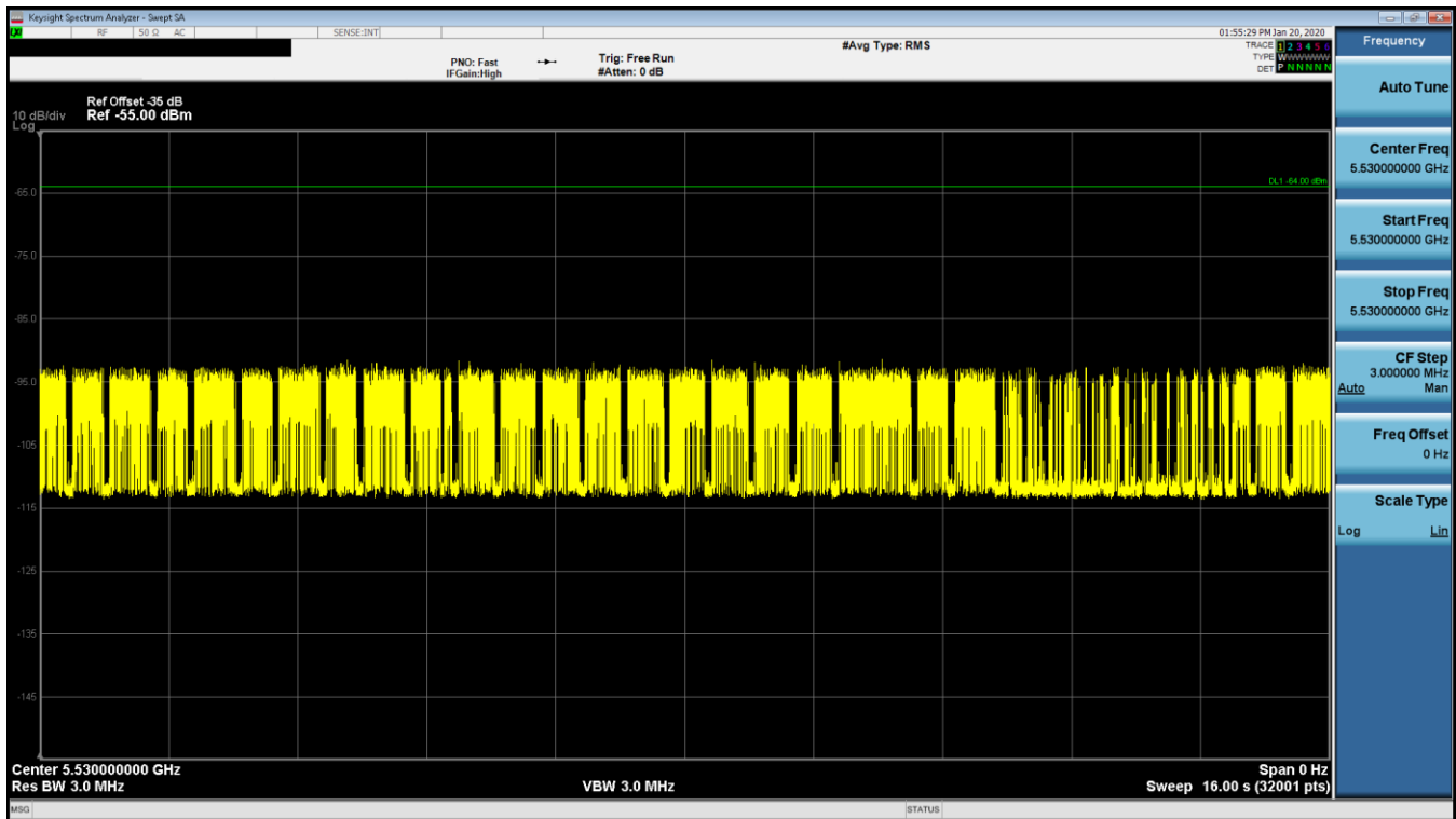
Figure 9-11. 5530MHz - Channel Loading - Mode 2 (80MHz)
