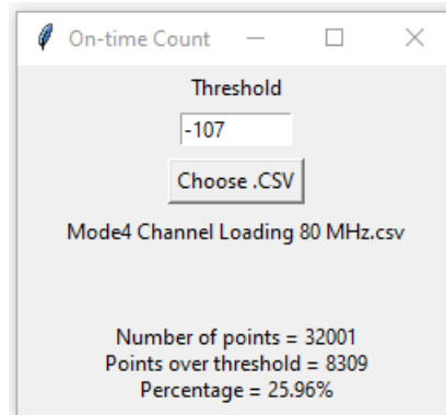
Figure 9-24. 5530MHz - Channel Loading Calculation - Mode 4 (80MHz)
