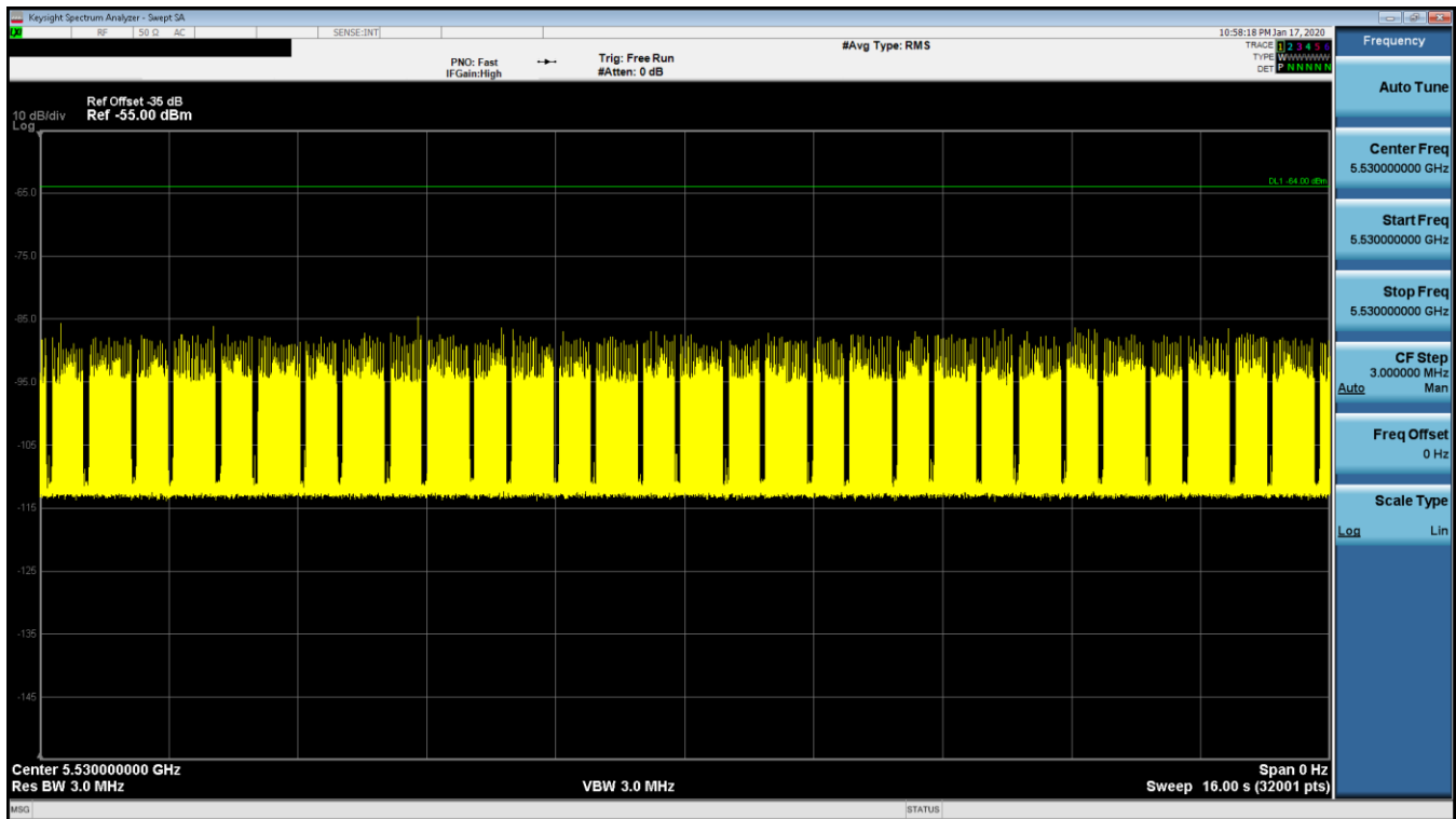
Figure 9-23. 5530MHz - Channel Loading - Mode 4 (80MHz)
