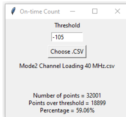
Figure 9-10 5510MHz - Channel Loading Calculation - Mode 2 (40MHz)
