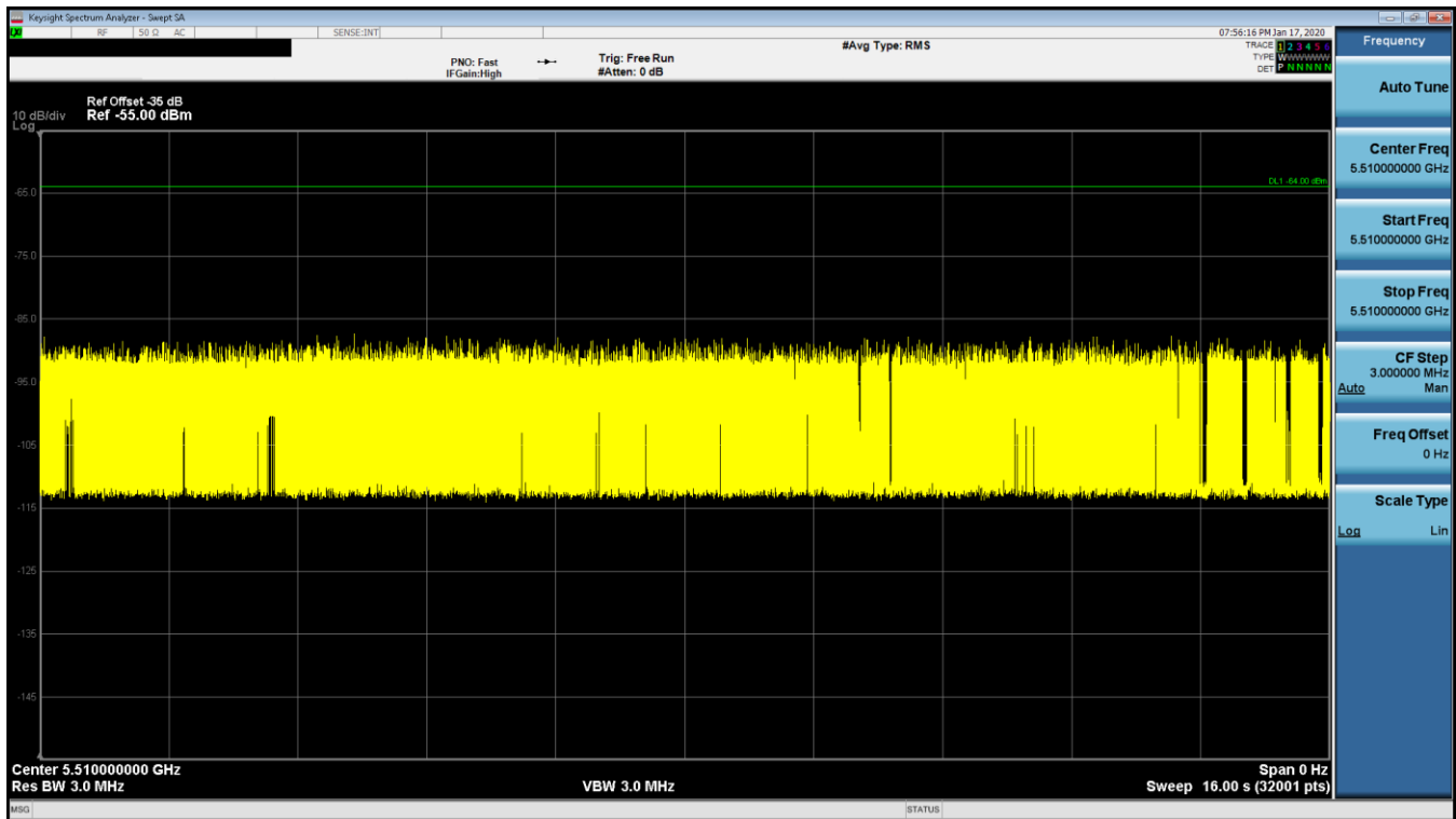
Figure 9-3. 5510MHz - Channel Loading - Mode 1 (40MHz)
