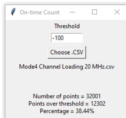
Figure 9-20. 5500MHz - Channel Loading Calculation - Mode 4 (20MHz)
