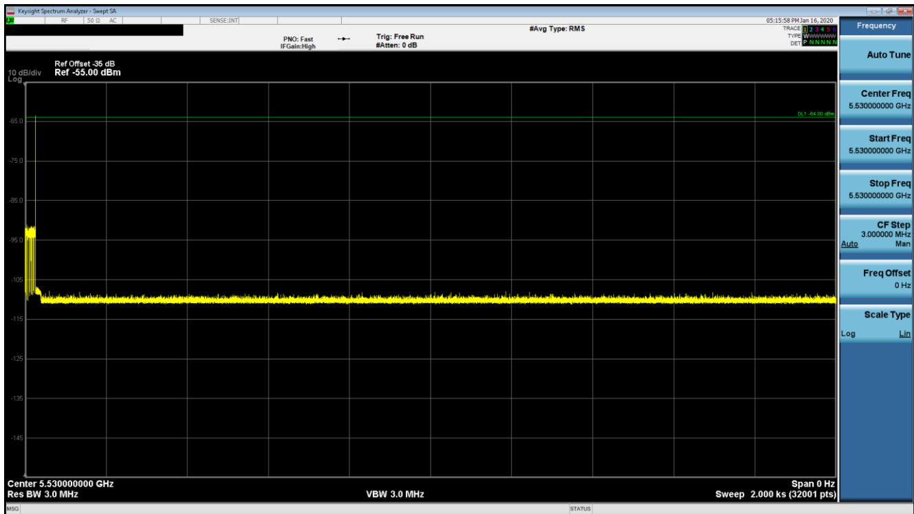
Figure 9-45. 5530MHz - Non-Occupancy Period (30 Minutes) - Mode 3 (80MHz)
