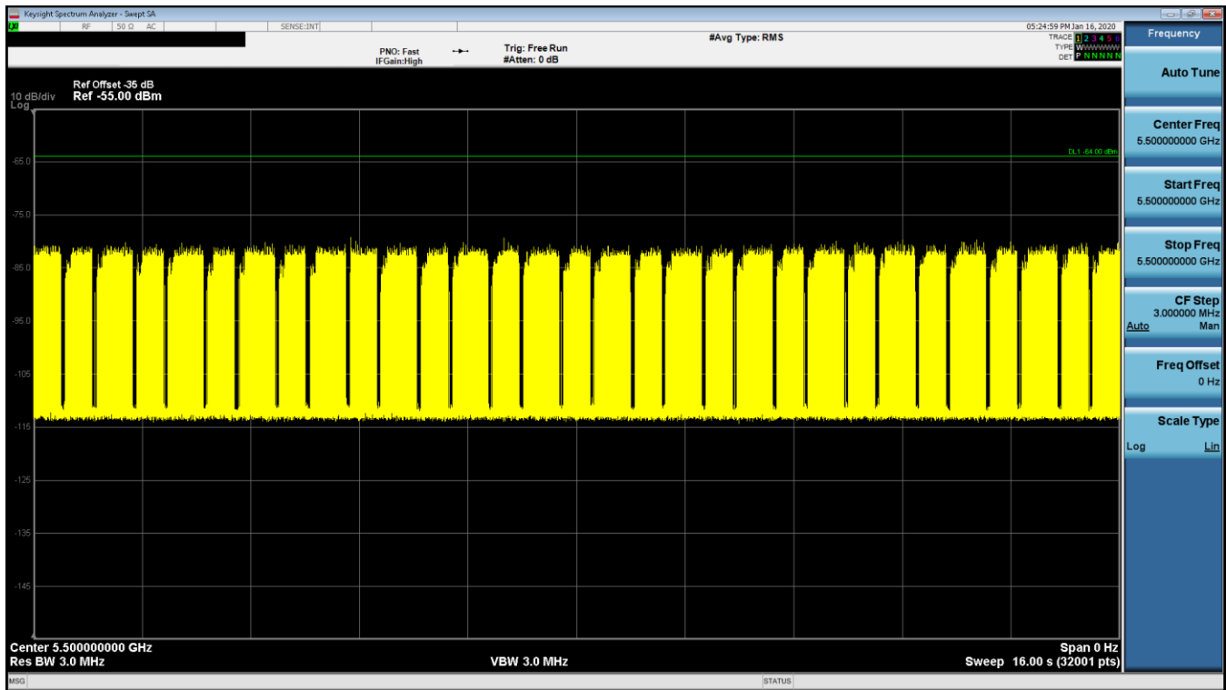
Figure 9-13. 5500MHz - Channel Loading - Mode 3 (20MHz)
