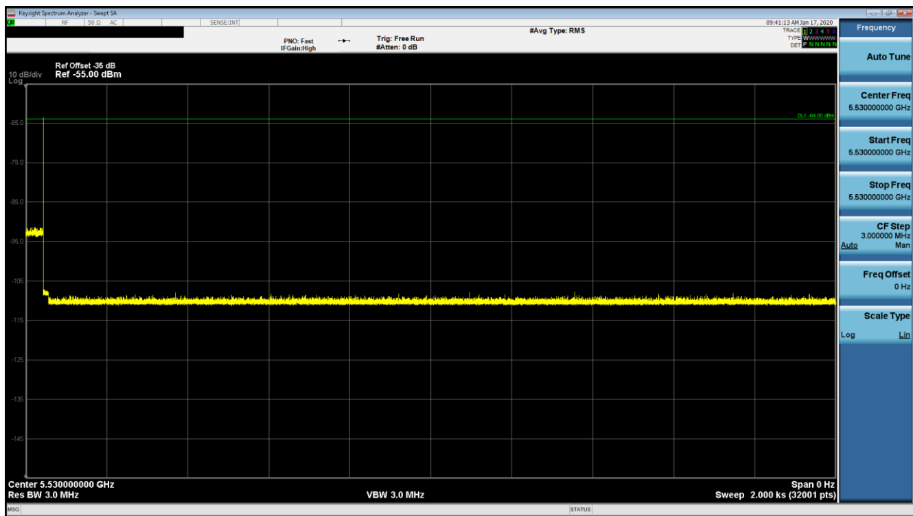
Figure 9-39. 5530MHz - Non-Occupancy Period (30 Minutes) - Mode 1 (80MHz)
