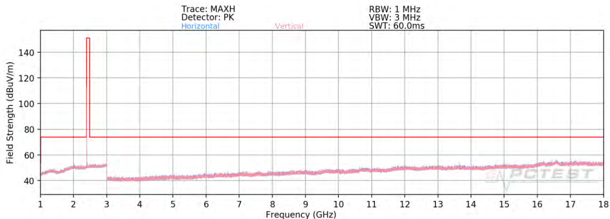
Plot 7-84. Radiated Spurious Plot Above 1GHz Ant 2a (1Mbps, ePA – Ch. 0)
