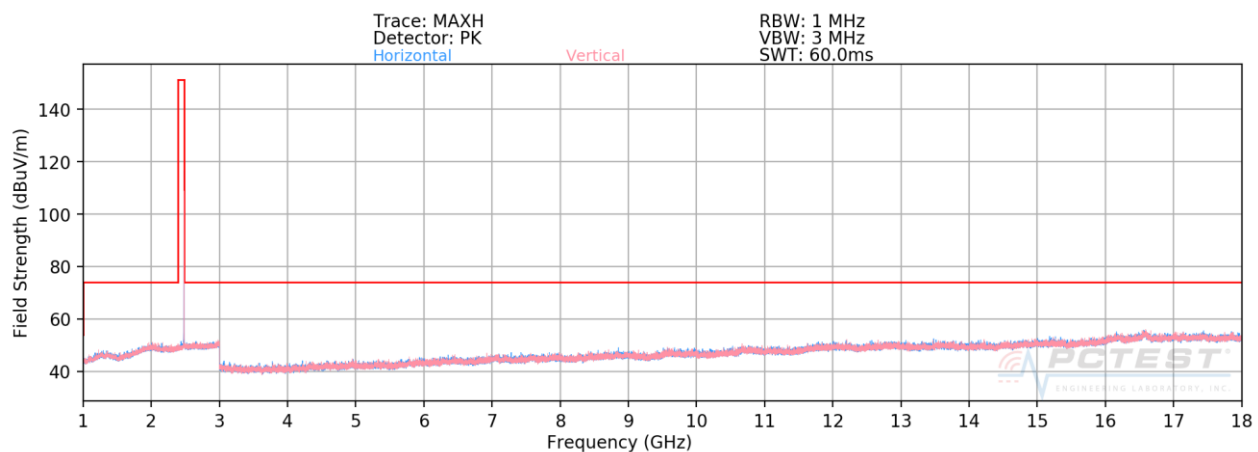
Plot 7-59. Radiated Spurious Plot above 1GHz Ant WF8 (BT GFSK ePA – Ch. 78)
