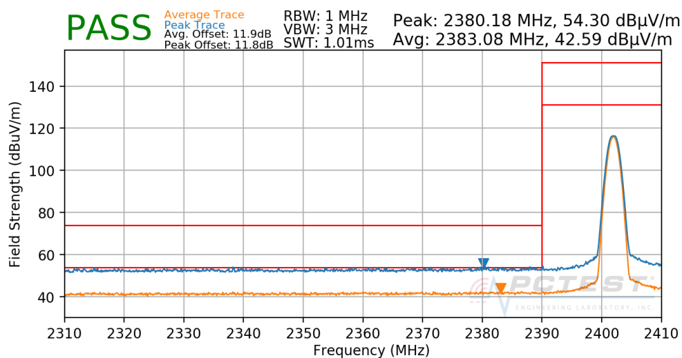
Plot 7-68. Radiated Restricted Lower Band Edge Measurement Ant WF8 (Average & Peak)
