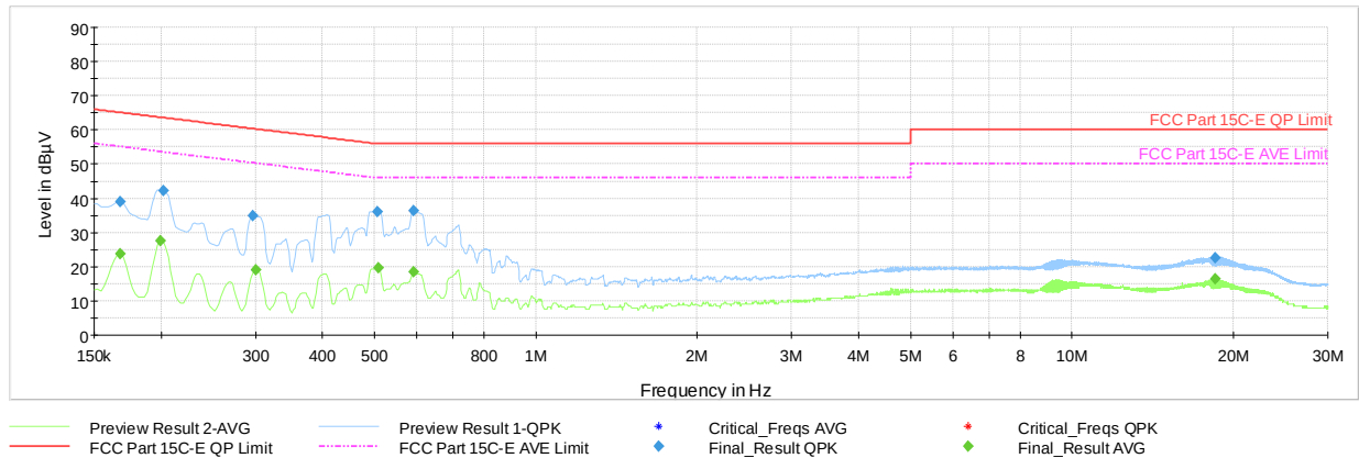
Plot 7-81. Line-Conducted Test Plot- Ch.39 TxBF (L1, with AC/DC Adapter)
