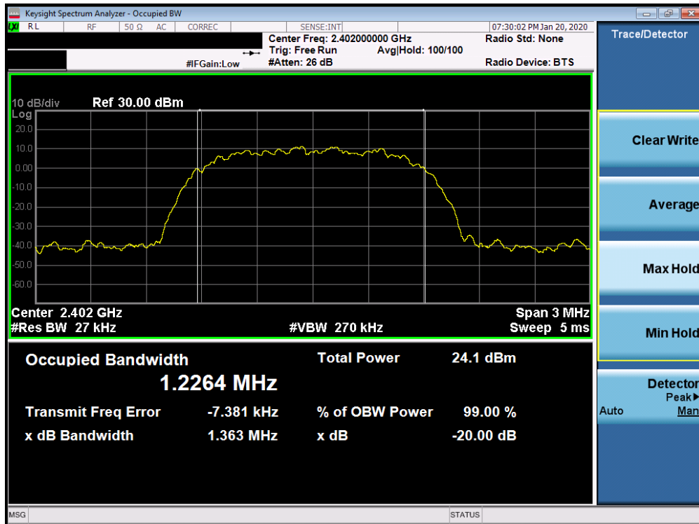
Plot 7-4. 20dB Bandwidth Plot Ant WF8 (Bluetooth, 8DPSK, ePA – Ch. 0)
