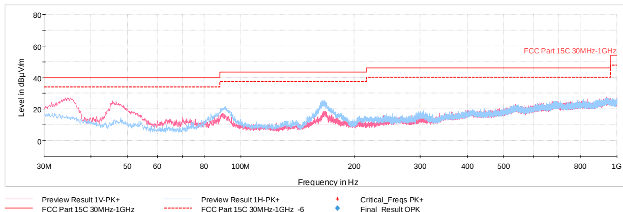
Plot 7-80. Radiated Spurious Plot below 1GHz GFSK ePA TxBF – Ch.39, with AC/DC Adapter)
