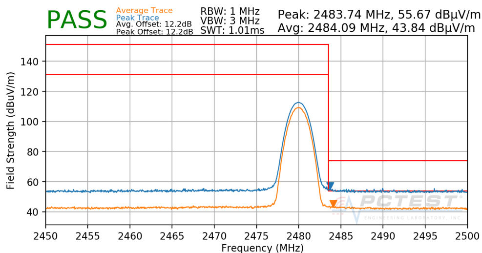
Plot 7-75. Radiated Restricted Upper Band Edge Measurement Ant WF7 (Average & Peak)
