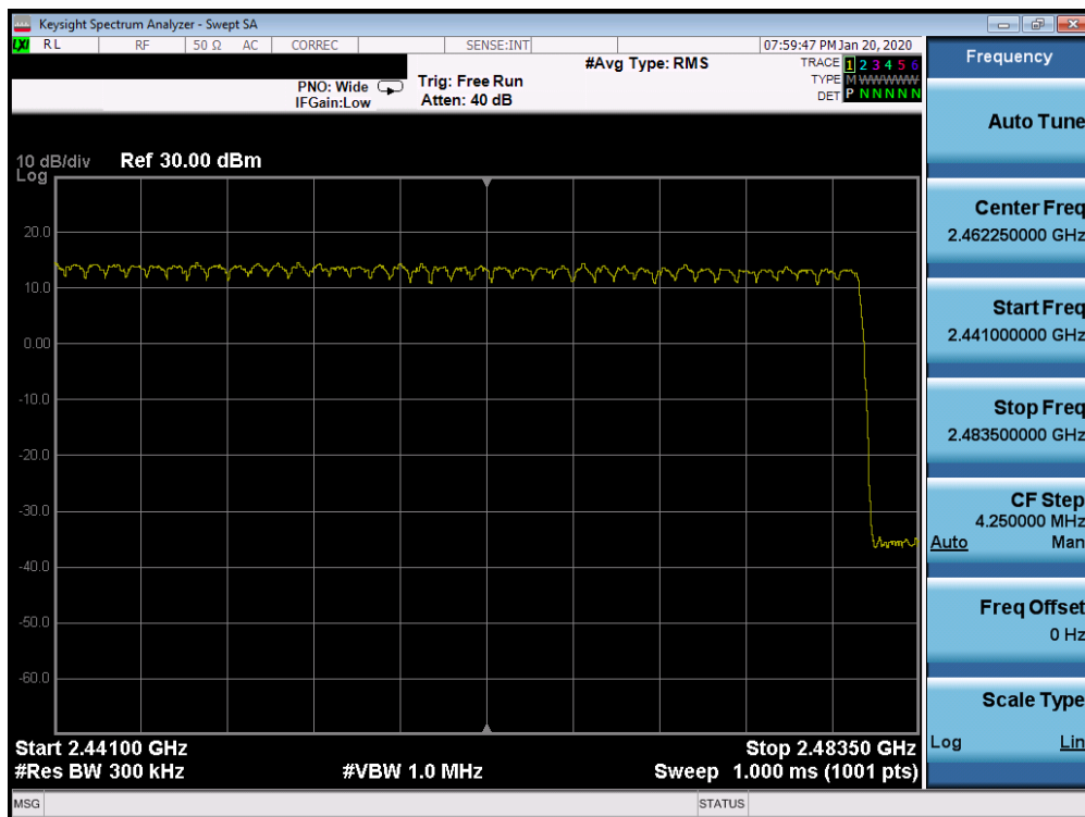
Plot 7-40. High End Spectrum Channel Hopping Plot Ant WF8 (Bluetooth, 8DPSK, ePA)
