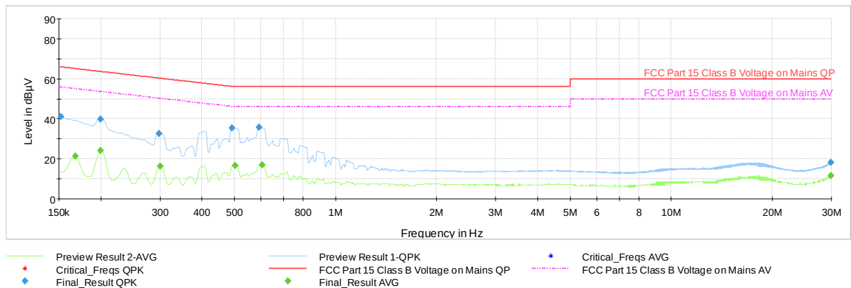
Plot 7-82. Line-Conducted Test Plot- Ch.39 TxBF (N, with AC/DC Adapter)
