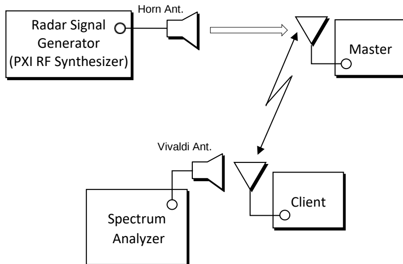
Figure 8-1. Test Setup (Mode 1)
