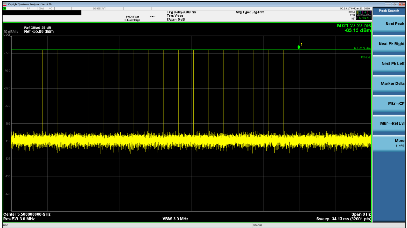
Figure 7-3. 5500MHz – Radar Pulse Type 0 (20MHz)
