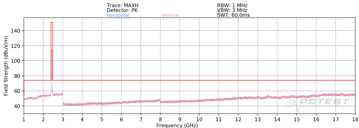
Plot 7-127. Radiated Spurious Plot above 1GHz SISO CORE 0 (802.11ax OFDMA – RU242 – Ch. 6)
