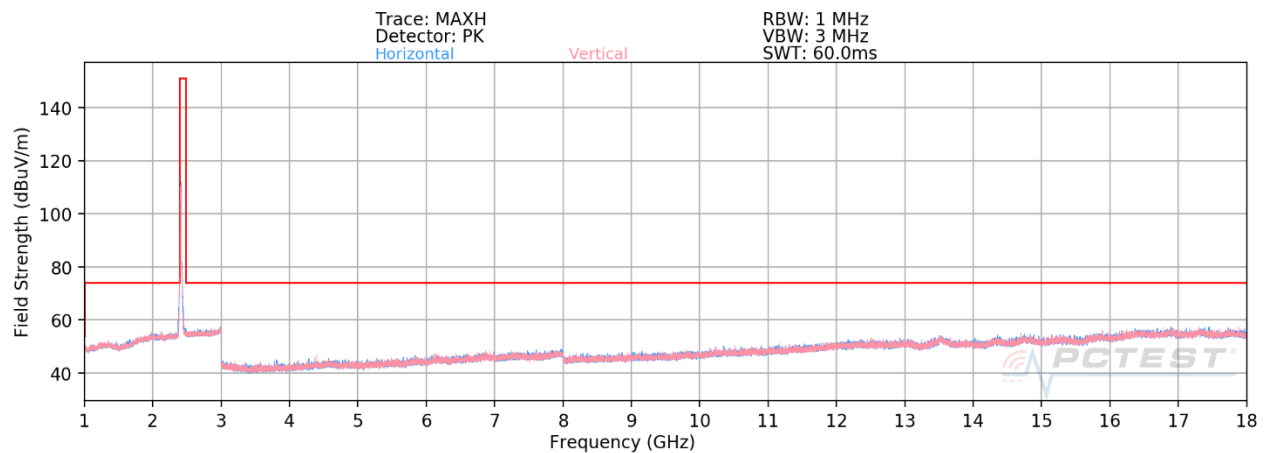
Plot 7-132. Radiated Spurious Plot above 1GHz SISO CORE 1 (802.11ax OFDMA – RU242 – Ch. 1)
