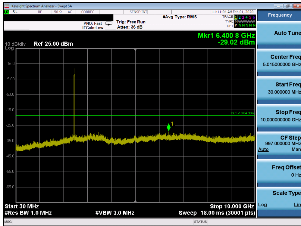
Plot 7-109. Conducted Spurious Plot SISO CORE 0 (802.11ax OFDMA – RU242 – Ch. 11)
