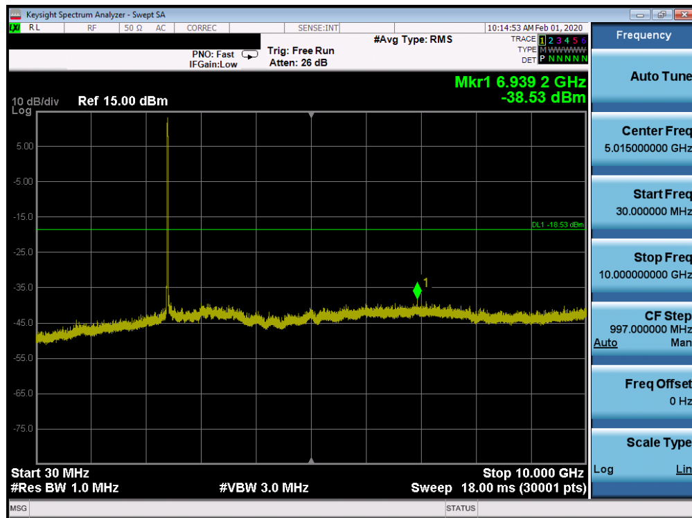
Plot 7-105. Conducted Spurious Plot SISO CORE 0 (802.11ax OFDMA – RU242 – Ch. 1)
