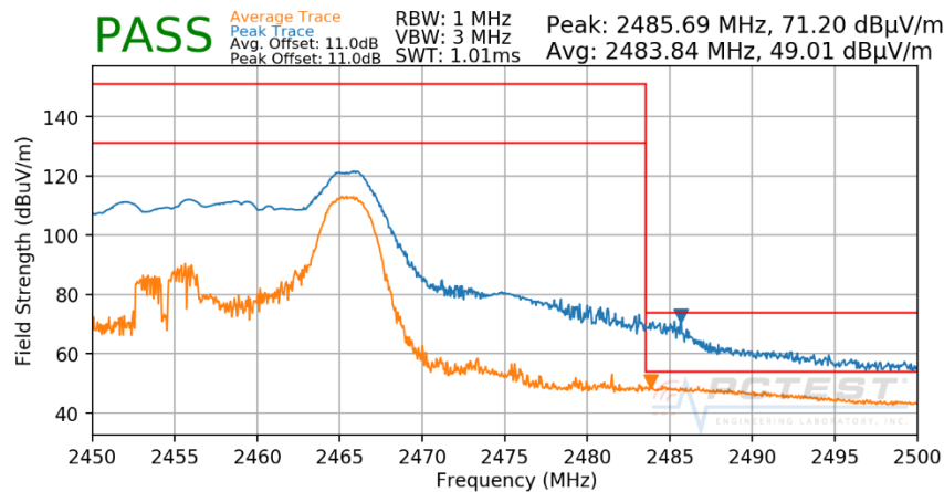
Plot 7-149. Radiated Restricted Upper Band Edge Measurement SISO CORE 0 (Peak & Average – RU26)
