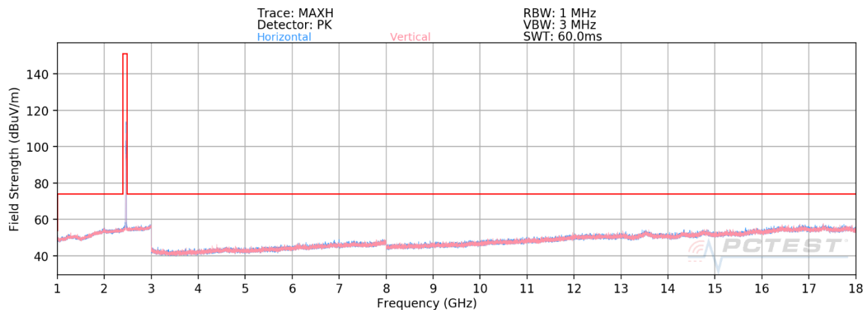
Plot 7-125. Radiated Spurious Plot above 1GHz SISO CORE 0 (802.11ax OFDMA – RU26 – Ch. 11)
