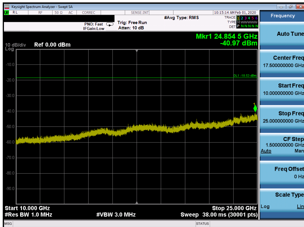
Plot 7-106. Conducted Spurious Plot SISO CORE 0 (802.11ax OFDMA – RU242 – Ch. 1)
