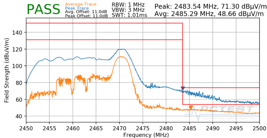
Plot 7-150. Radiated Restricted Upper Band Edge Measurement SISO CORE 0 (Peak & Average – RU26)
