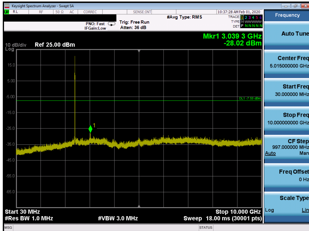
Plot 7-99. Conducted Spurious Plot SISO CORE 0 (802.11ax OFDMA – RU26 – Ch. 1)
