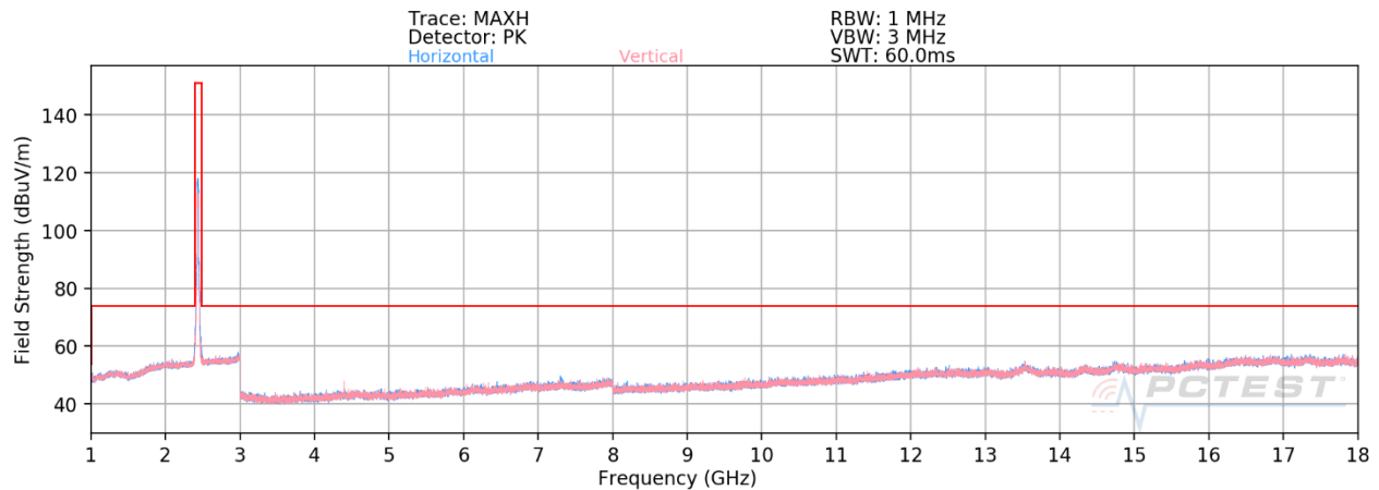
Plot 7-139. Radiated Spurious Plot above 1GHz CDD (802.11ax OFDMA – RU242 – Ch. 6)
