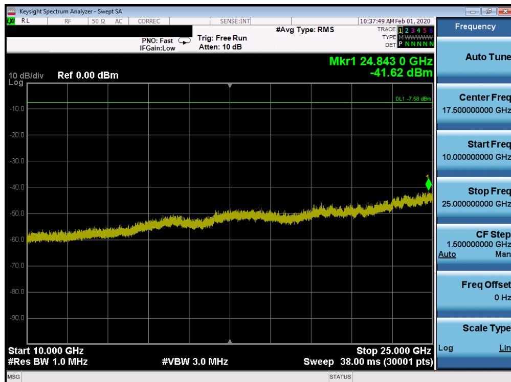
Plot 7-100. Conducted Spurious Plot SISO CORE 0 (802.11ax OFDMA – RU26 – Ch. 1)
