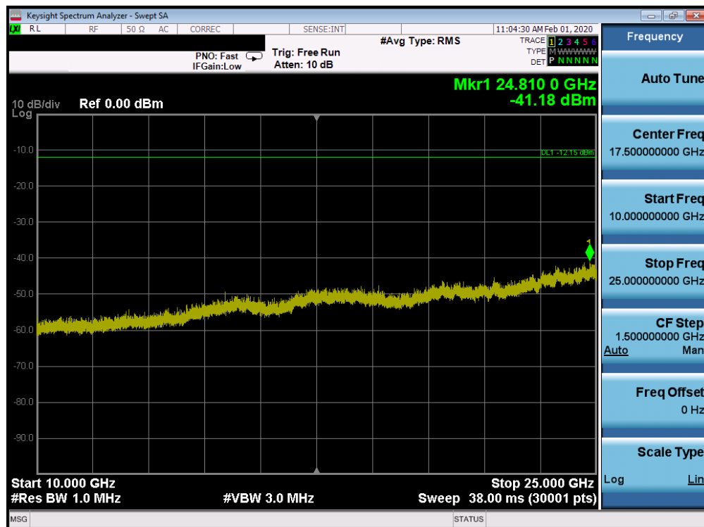
Plot 7-104. Conducted Spurious Plot SISO CORE 0 (802.11ax OFDMA – RU26 – Ch. 11)
