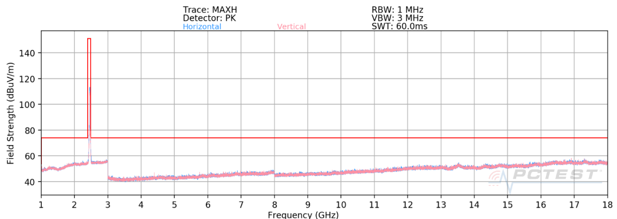
Plot 7-134. Radiated Spurious Plot above 1GHz SISO CORE 1 (802.11ax OFDMA – RU242 – Ch. 11)
