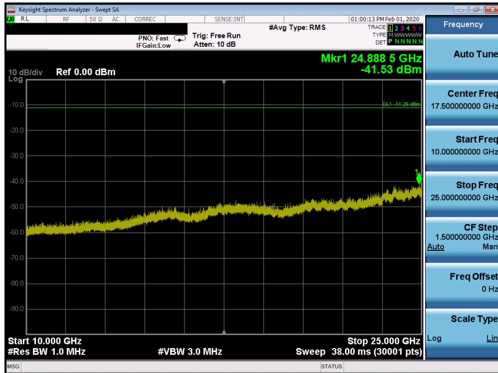
Plot 7-112. Conducted Spurious Plot SISO CORE 1 (802.11ax OFDMA – RU26 – Ch. 1)
