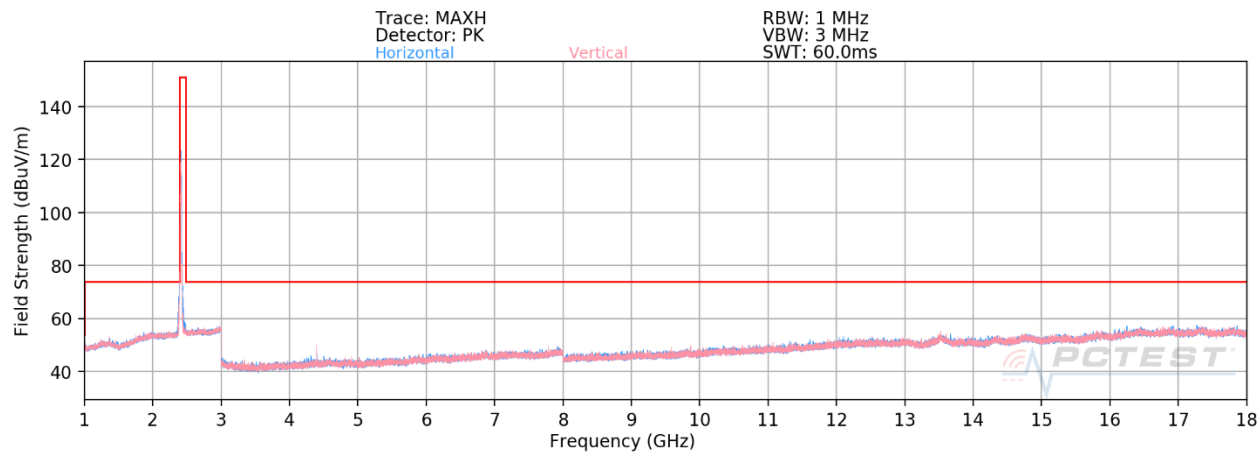
Plot 7-135. Radiated Spurious Plot above 1GHz CDD (802.11ax OFDMA – RU26 – Ch. 1)
