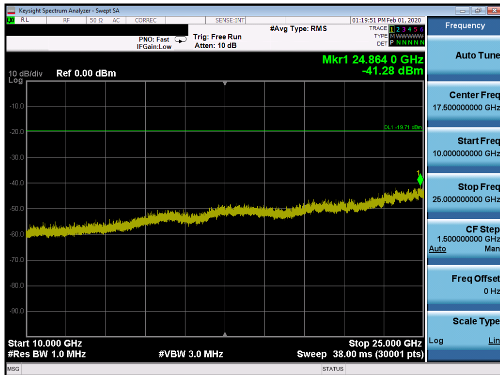
Plot 7-122. Conducted Spurious Plot SISO CORE 1 (802.11ax OFDMA – RU242 – Ch. 11)
