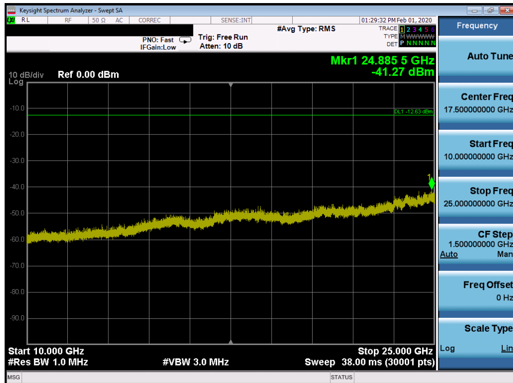
Plot 7-116. Conducted Spurious Plot SISO CORE 1 (802.11ax OFDMA – RU26 – Ch. 11)
