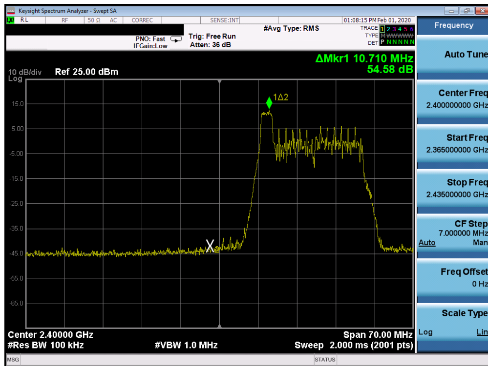
Plot 7-88. Band Edge SISO CORE 1 (802.11ax OFDMA – RU26 Index 0 – Ch. 2)
