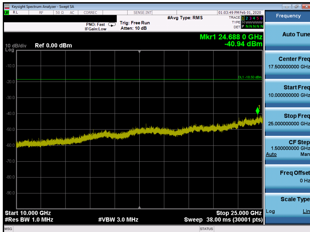
Plot 7-118. Conducted Spurious Plot SISO CORE 1 (802.11ax OFDMA – RU242 – Ch. 1)
