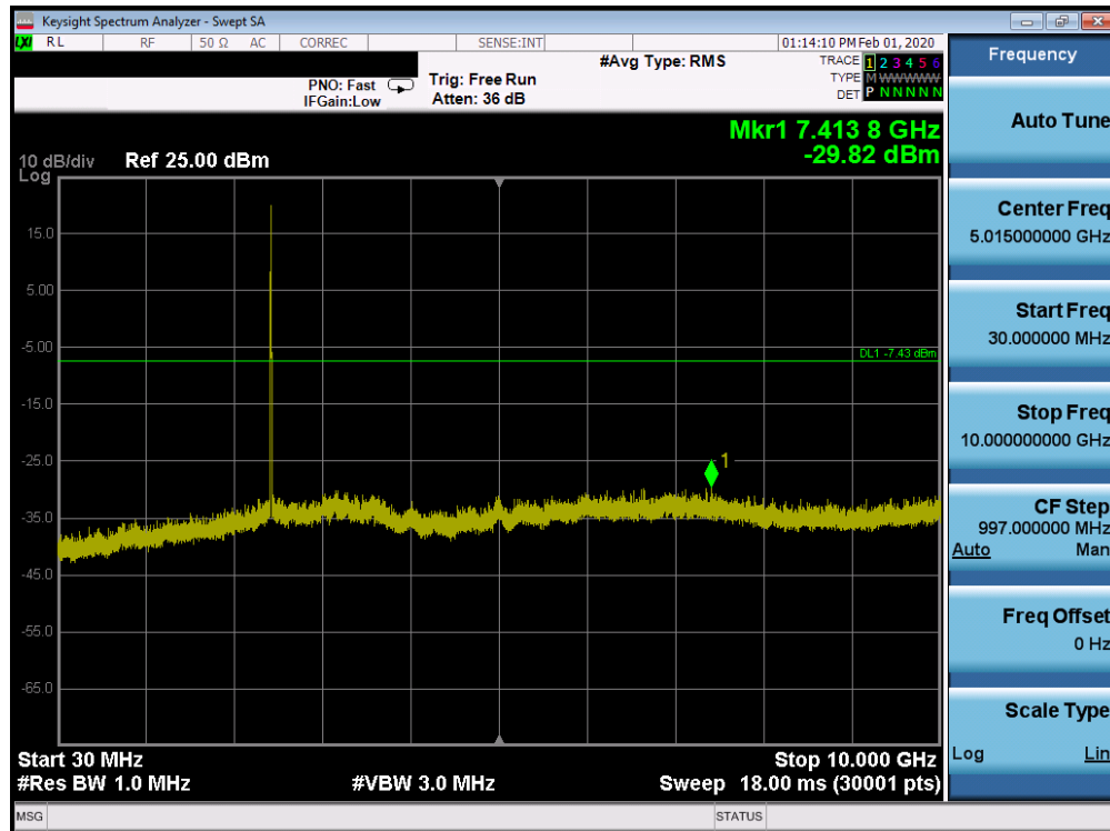
Plot 7-113. Conducted Spurious Plot SISO CORE 1 (802.11ax OFDMA – RU26 – Ch. 6)
