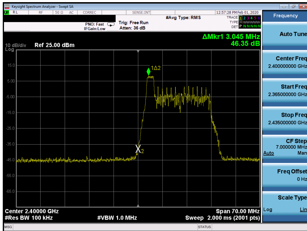
Plot 7-87. Band Edge SISO CORE 1 (802.11ax OFDMA – RU26 Index 0 – Ch. 1)
