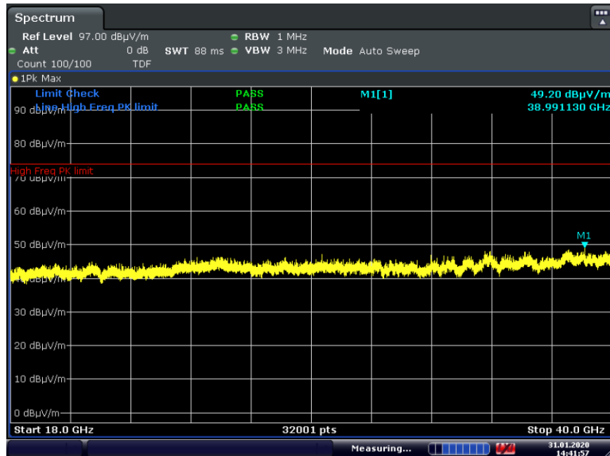
Plot 7-143. Radiated Spurious Plot above 18GHz CDD (802.11ax OFDMA – RU242, Pol. H)
