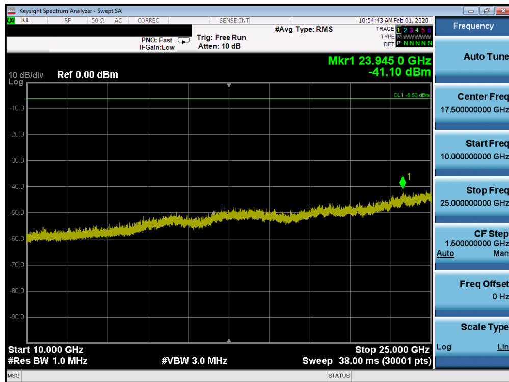
Plot 7-102. Conducted Spurious Plot SISO CORE 0 (802.11ax OFDMA – RU26 – Ch. 6)
