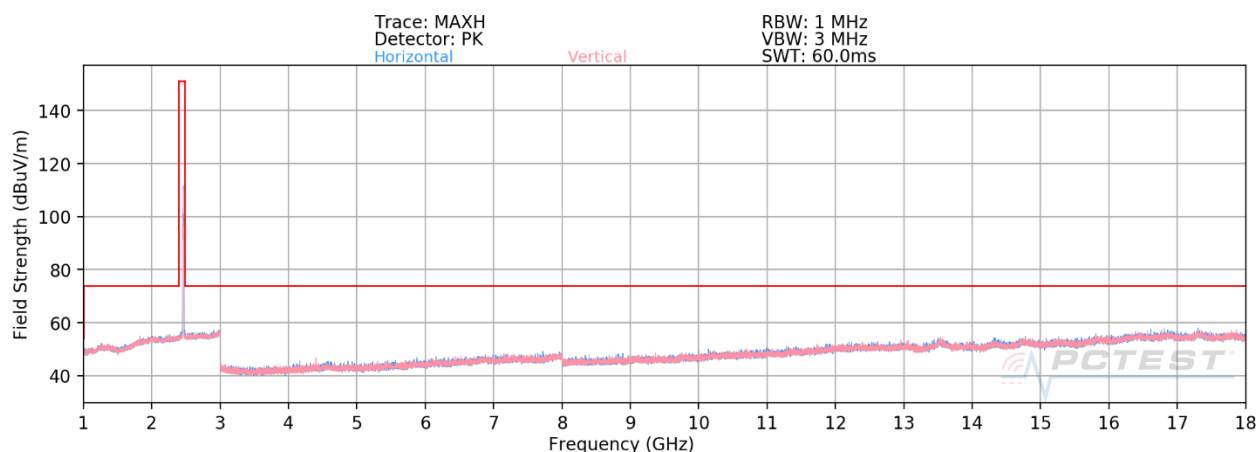
Plot 7-131. Radiated Spurious Plot above 1GHz SISO CORE 1 (802.11ax OFDMA – RU26 – Ch. 11)
