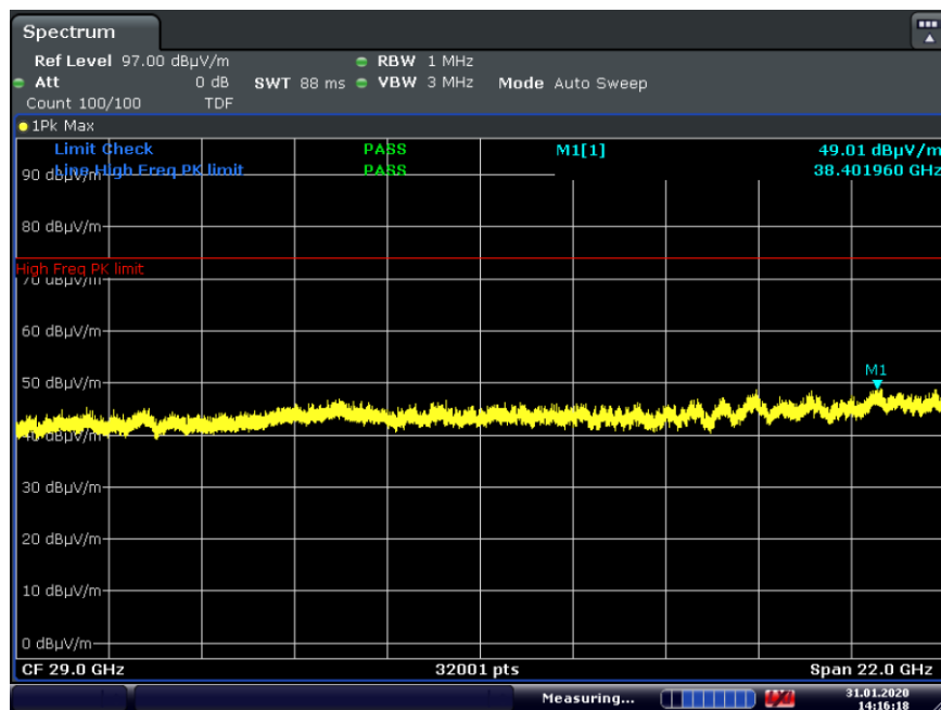
Plot 7-142. Radiated Spurious Plot above 18GHz CDD (802.11ax OFDMA – RU26, Pol. V)
