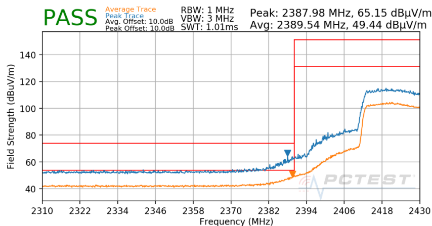
Plot 7-154. Radiated Restricted Lower Band Edge Measurement SISO CORE 0 (Peak & Average – RU242)
