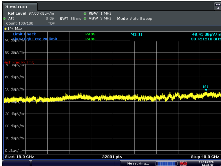
Plot 7-144. Radiated Spurious Plot above 18GHz CDD (802.11ax OFDMA – RU242, Pol. V)
