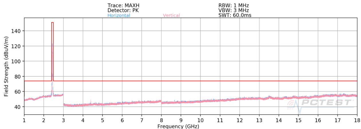
Plot 7-136. Radiated Spurious Plot above 1GHz CDD (802.11ax OFDMA – RU26 – Ch. 6)
