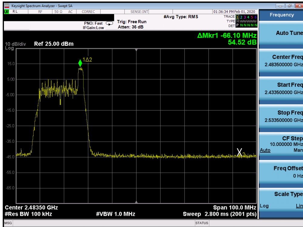
Plot 7-89. Band Edge SISO CORE 1 (802.11ax OFDMA – RU26 Index 8 – Ch. 9)
