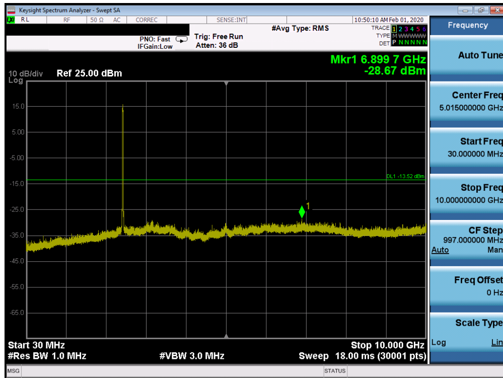
Plot 7-107. Conducted Spurious Plot SISO CORE 0 (802.11ax OFDMA – RU242 – Ch. 6)
