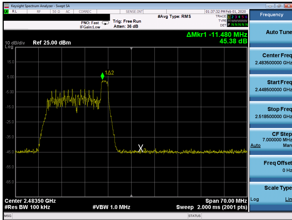
Plot 7-91. Band Edge SISO CORE 1 (802.11ax OFDMA – RU26 Index 8 – Ch. 11)
