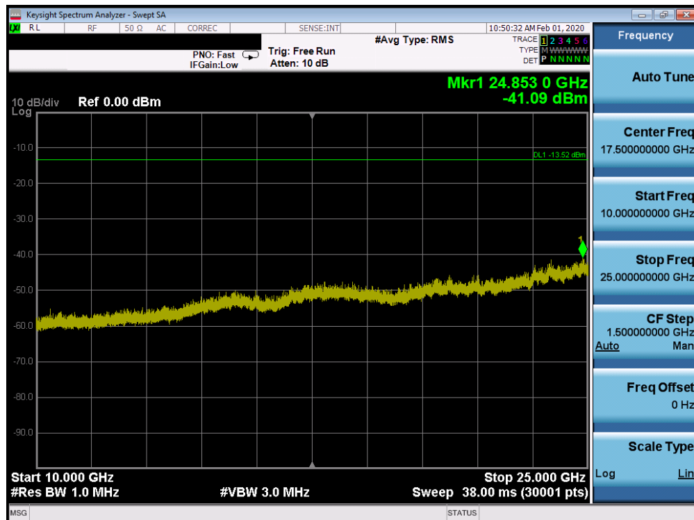
Plot 7-108. Conducted Spurious Plot SISO CORE 0 (802.11ax OFDMA – RU242 – Ch. 6)
