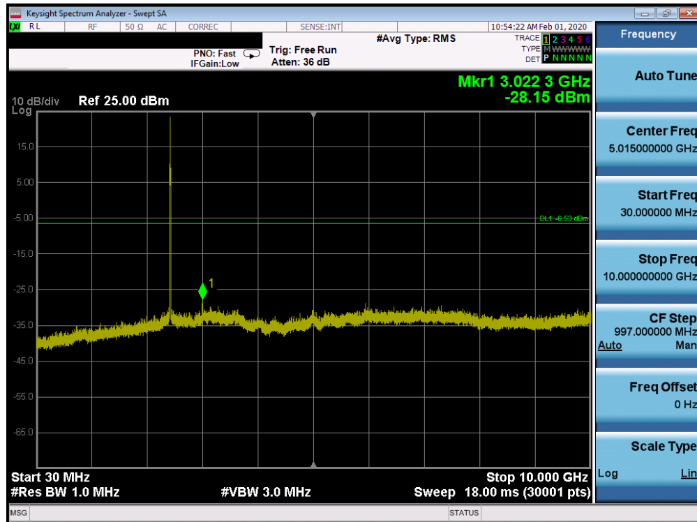
Plot 7-101. Conducted Spurious Plot SISO CORE 0 (802.11ax OFDMA – RU26 – Ch. 6)
