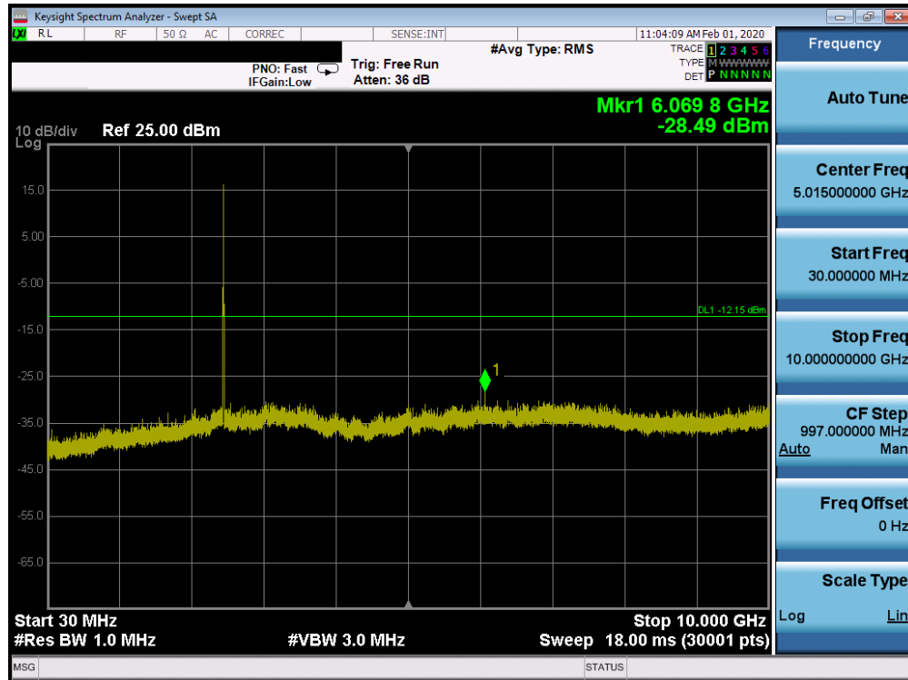
Plot 7-103. Conducted Spurious Plot SISO CORE 0 (802.11ax OFDMA – RU26 – Ch. 11)
