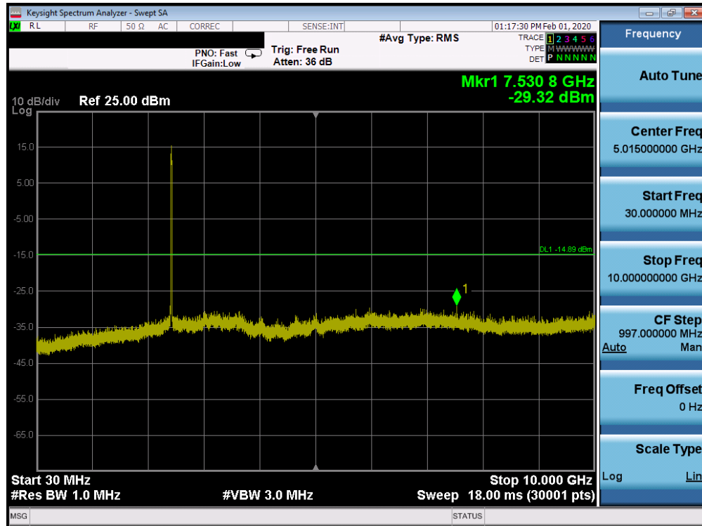
Plot 7-119. Conducted Spurious Plot SISO CORE 1 (802.11ax OFDMA – RU242 – Ch. 6)
