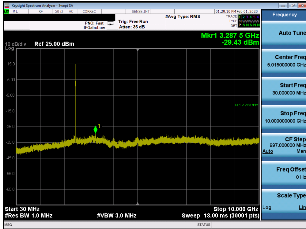
Plot 7-115. Conducted Spurious Plot SISO CORE 1 (802.11ax OFDMA – RU26 – Ch. 11)
