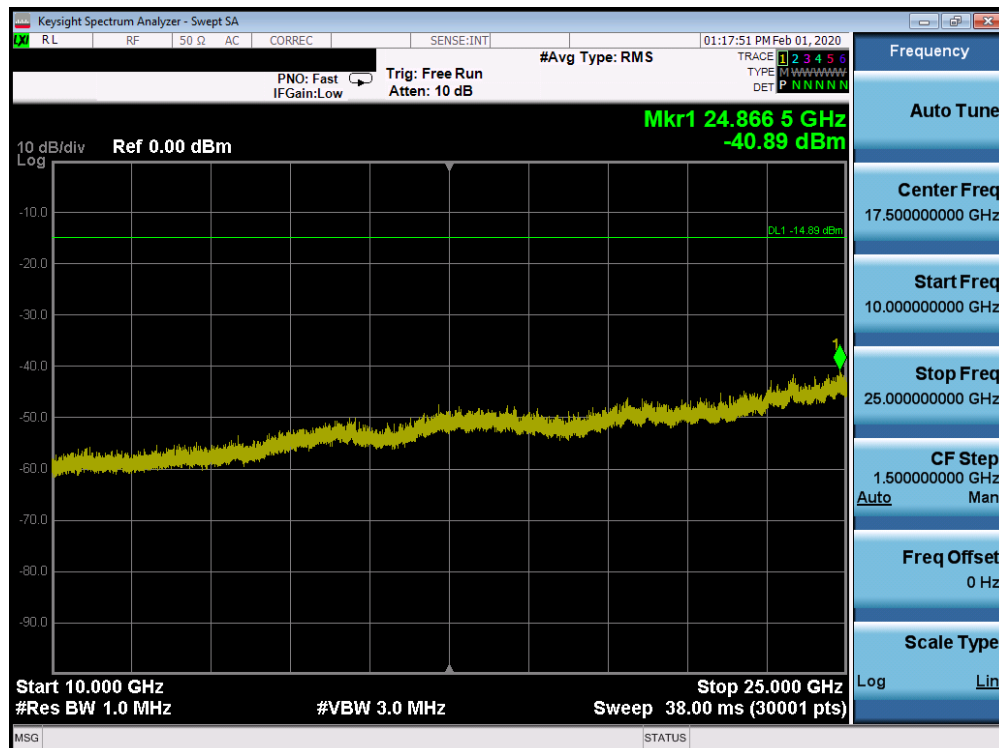
Plot 7-120. Conducted Spurious Plot SISO CORE 1 (802.11ax OFDMA – RU242 – Ch. 6)
