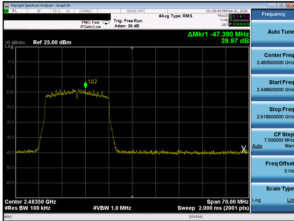
Plot 7-97. Band Edge SISO CORE 1 (802.11ax OFDMA – RU242 – Ch. 11)
