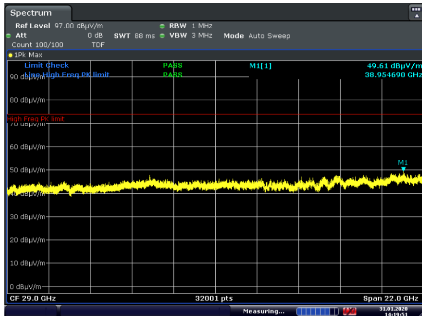
Plot 7-141. Radiated Spurious Plot above 18GHz CDD (802.11ax OFDMA – RU26, Pol. H)
