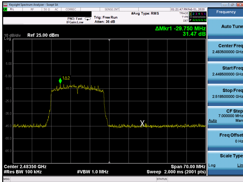
Plot 7-98. Band Edge SISO CORE 1 (802.11ax OFDMA – RU242 – Ch. 12)
