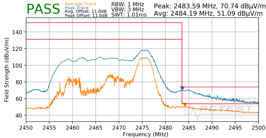
Plot 7-151. Radiated Restricted Upper Band Edge Measurement SISO CORE 0 (Peak & Average – RU26)
