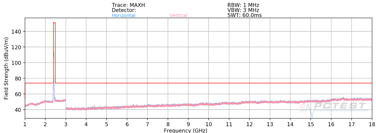
Plot 7-126. Radiated Spurious Plot above 1GHz SISO CORE 0 (802.11ax OFDMA – RU242 – Ch. 1)
