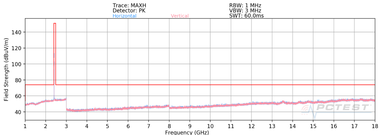
Plot 7-123. Radiated Spurious Plot above 1GHz SISO CORE 0 (802.11ax OFDMA – RU26 – Ch. 1)
