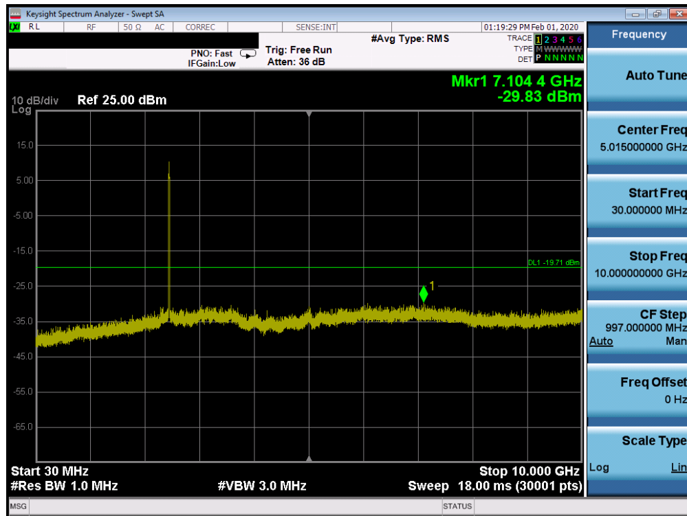
Plot 7-121. Conducted Spurious Plot SISO CORE 1 (802.11ax OFDMA – RU242 – Ch. 11)
