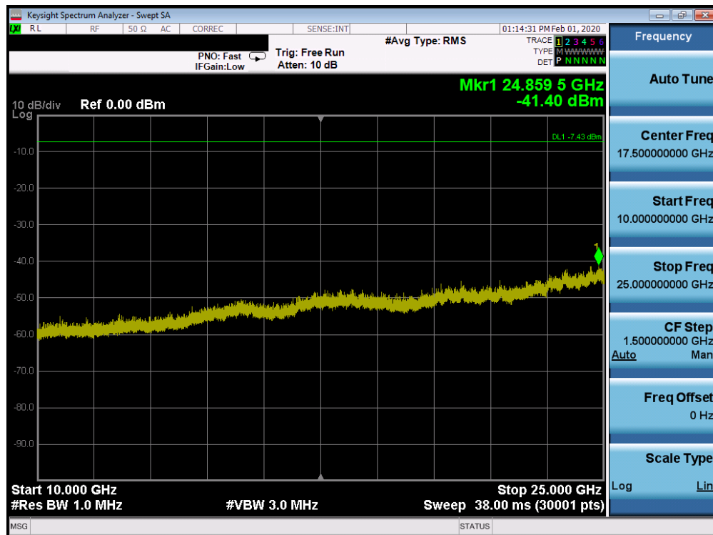
Plot 7-114. Conducted Spurious Plot SISO CORE 1 (802.11ax OFDMA – RU26 – Ch. 6)
