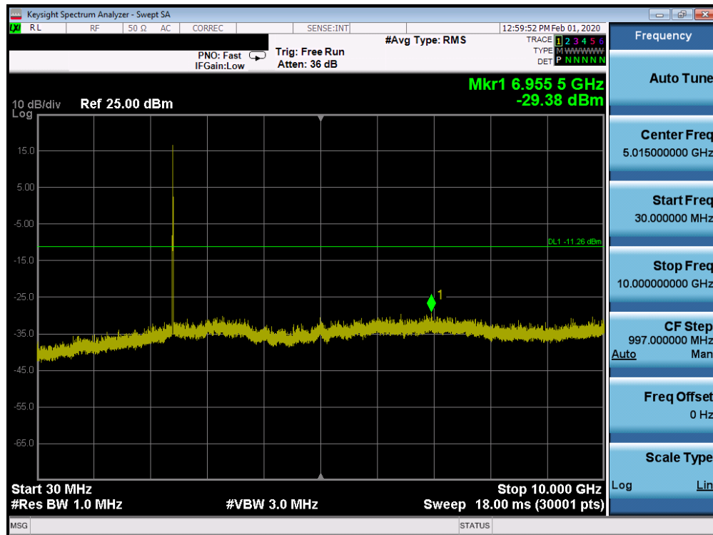
Plot 7-111. Conducted Spurious Plot SISO CORE 1 (802.11ax OFDMA – RU26 – Ch. 1)
