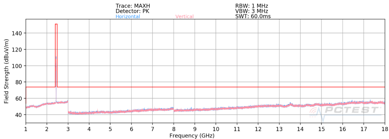
Plot 7-130. Radiated Spurious Plot above 1GHz SISO CORE 1 (802.11ax OFDMA – RU26 – Ch. 6)
