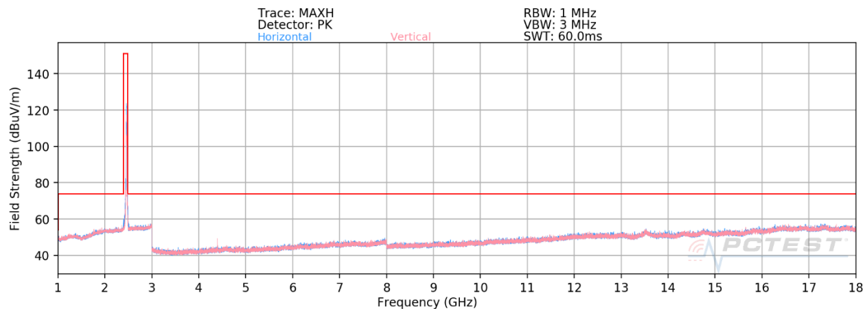
Plot 7-137. Radiated Spurious Plot above 1GHz CDD (802.11ax OFDMA – RU26 – Ch. 11)
