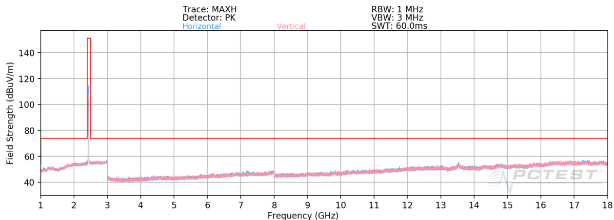
Plot 7-124. Radiated Spurious Plot above 1GHz SISO CORE 0 (802.11ax OFDMA – RU26 – Ch. 6)
