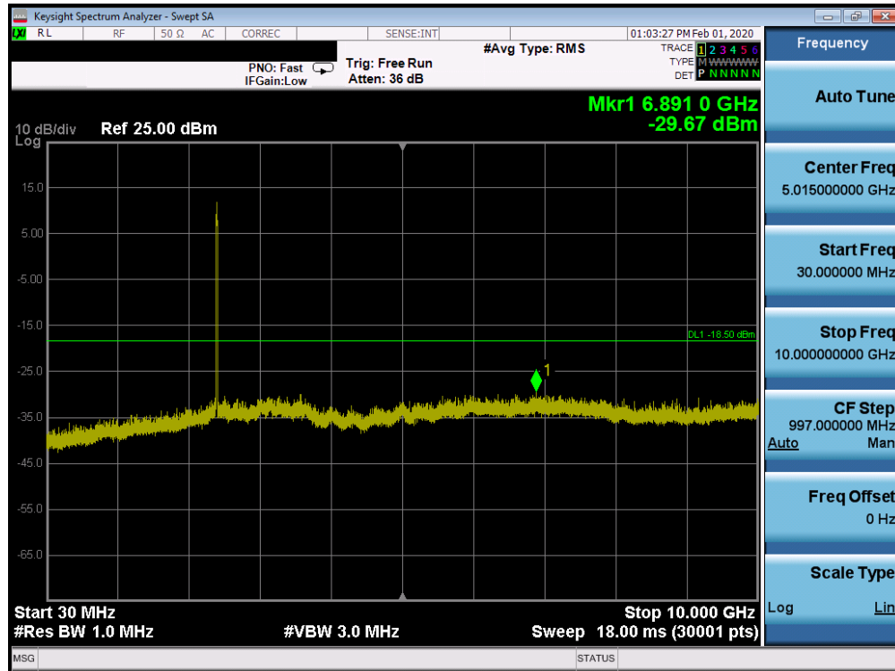
Plot 7-117. Conducted Spurious Plot SISO CORE 1 (802.11ax OFDMA – RU242 – Ch. 1)
