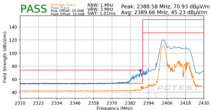
Plot 7-145. Radiated Restricted Lower Band Edge Measurement SISO CORE 0 (Peak & Average – RU26)
