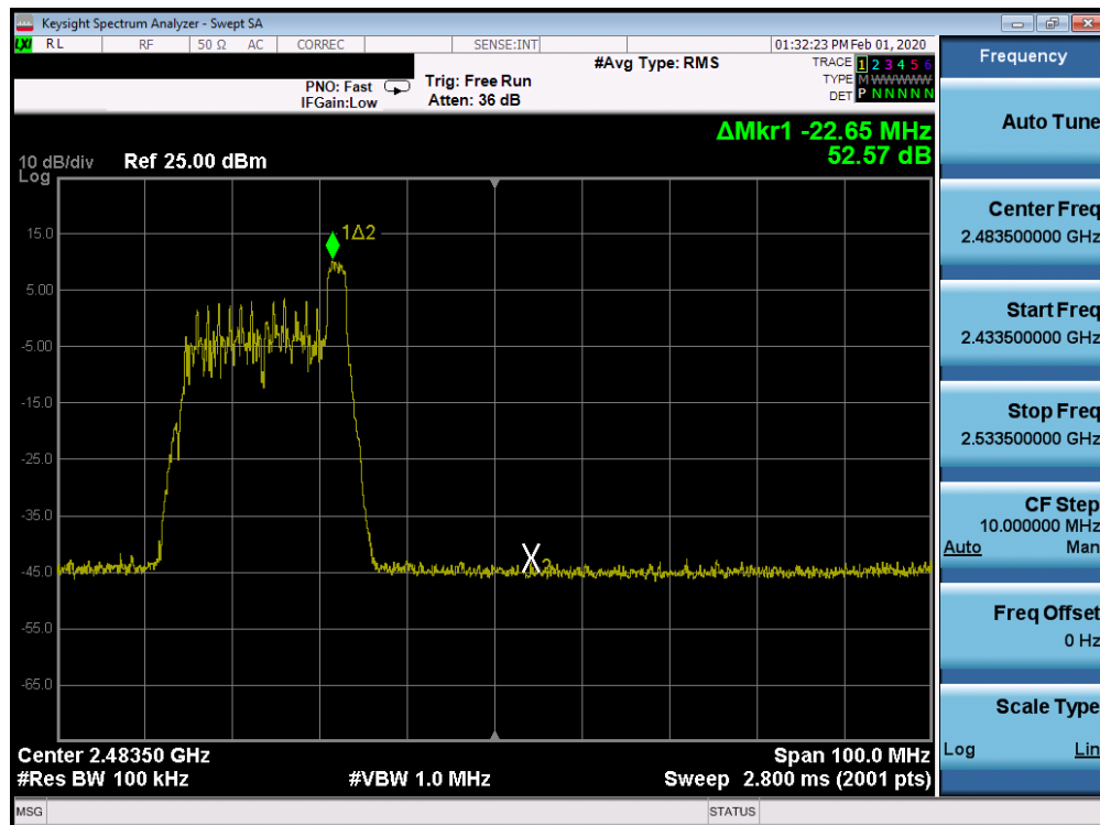
Plot 7-90. Band Edge SISO CORE 1 (802.11ax OFDMA – RU26 Index 8 – Ch. 10)
