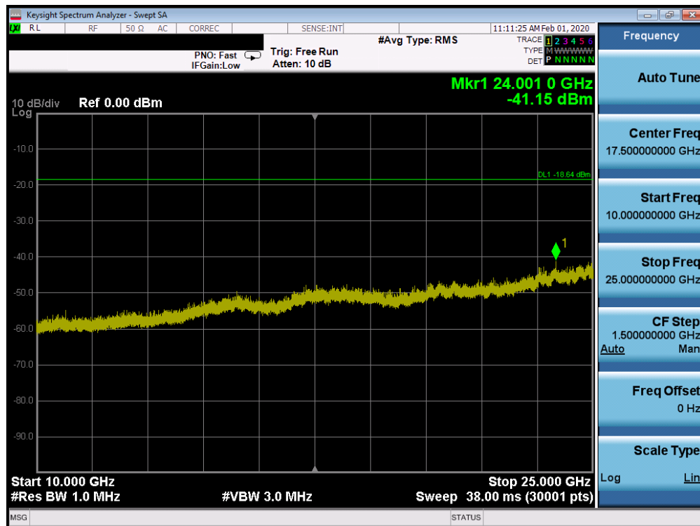
Plot 7-110. Conducted Spurious Plot SISO CORE 0 (802.11ax OFDMA – RU242 – Ch. 11)
