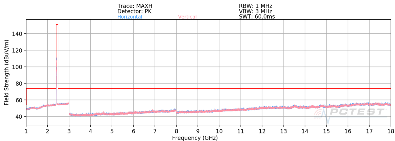
Plot 7-129. Radiated Spurious Plot above 1GHz SISO CORE 1 (802.11ax OFDMA – RU26 – Ch. 1)
