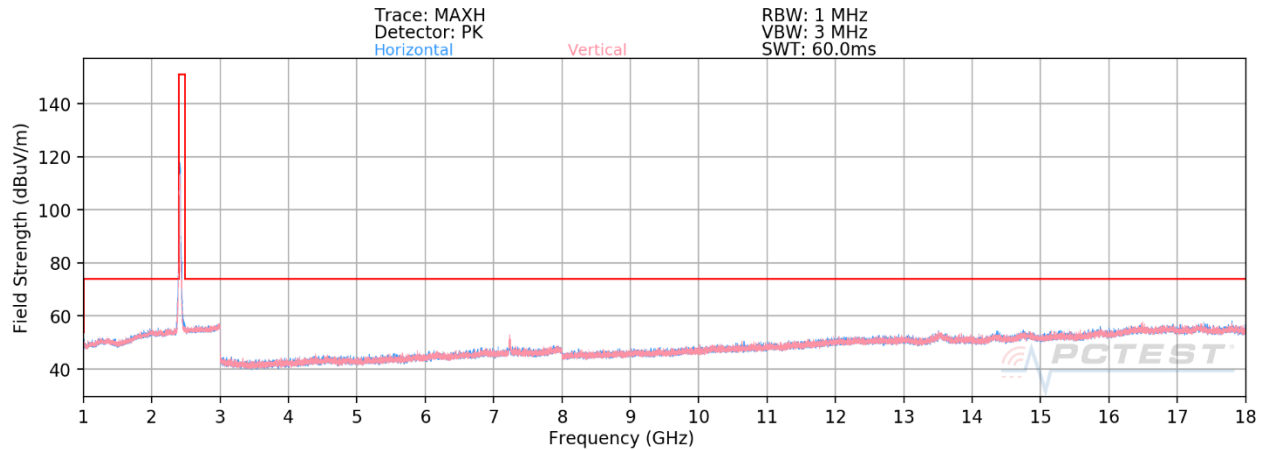
Plot 7-138. Radiated Spurious Plot above 1GHz CDD (802.11ax OFDMA – RU242 – Ch. 1)
