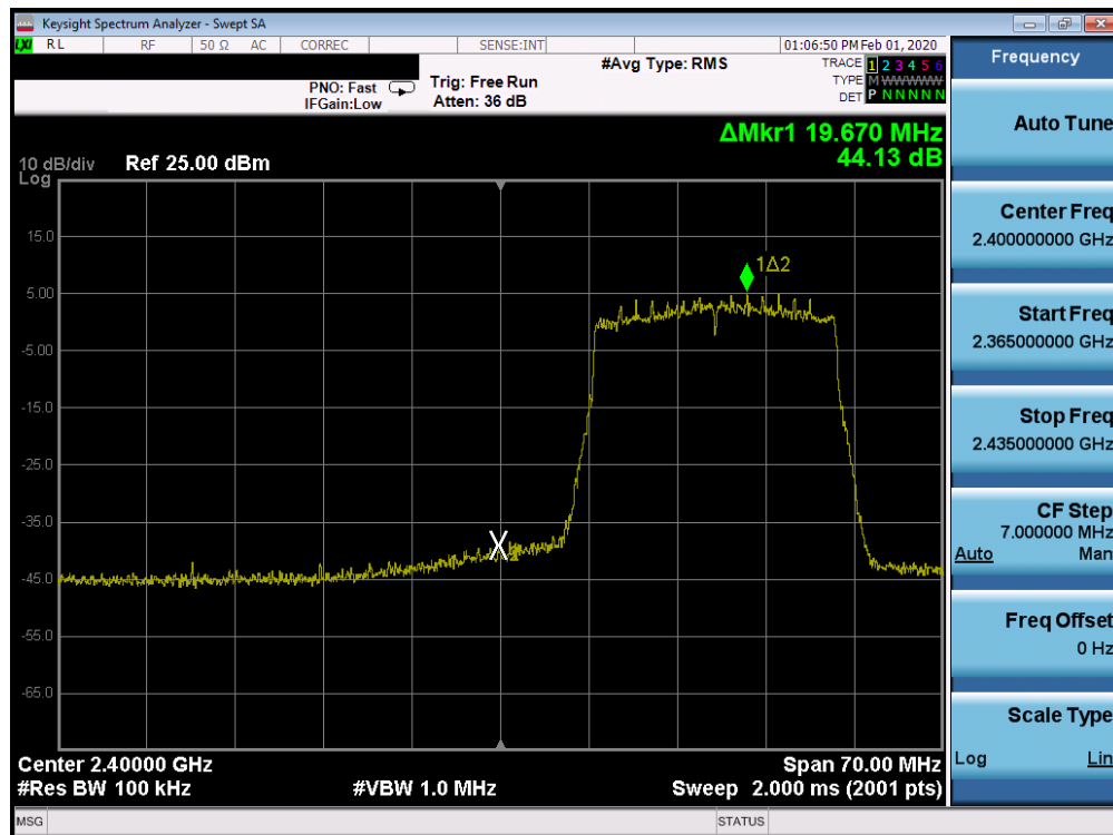
Plot 7-94. Band Edge SISO CORE 1 (802.11ax OFDMA – RU242 – Ch. 2)
