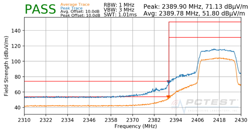
Plot 7-153. Radiated Restricted Lower Band Edge Measurement SISO CORE 0 (Peak & Average – RU242)
