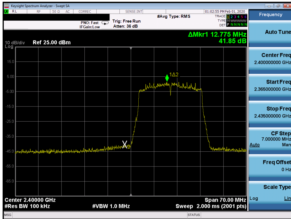
Plot 7-93. Band Edge SISO CORE 1 (802.11ax OFDMA – RU242 – Ch. 1)
