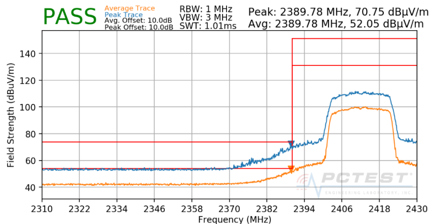
Plot 7-152. Radiated Restricted Lower Band Edge Measurement SISO CORE 0 (Peak & Average – RU242)
