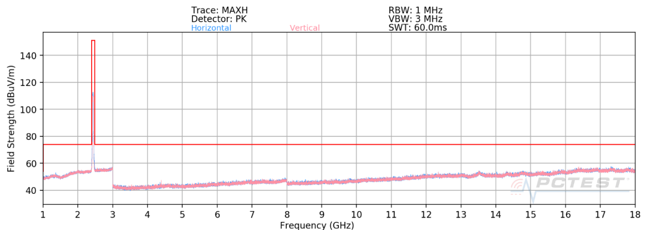
Plot 7-133. Radiated Spurious Plot above 1GHz SISO CORE 1 (802.11ax OFDMA – RU242 – Ch. 6)
