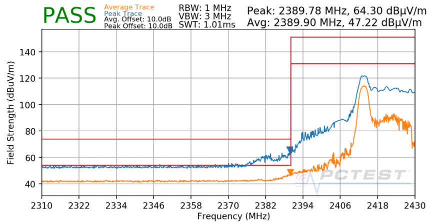
Plot 7-147. Radiated Restricted Lower Band Edge Measurement SISO CORE 0 (Peak & Average – RU26)
