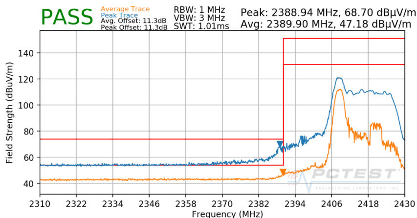
Plot 7-146. Radiated Restricted Lower Band Edge Measurement SISO CORE 0 (Peak & Average – RU26)
