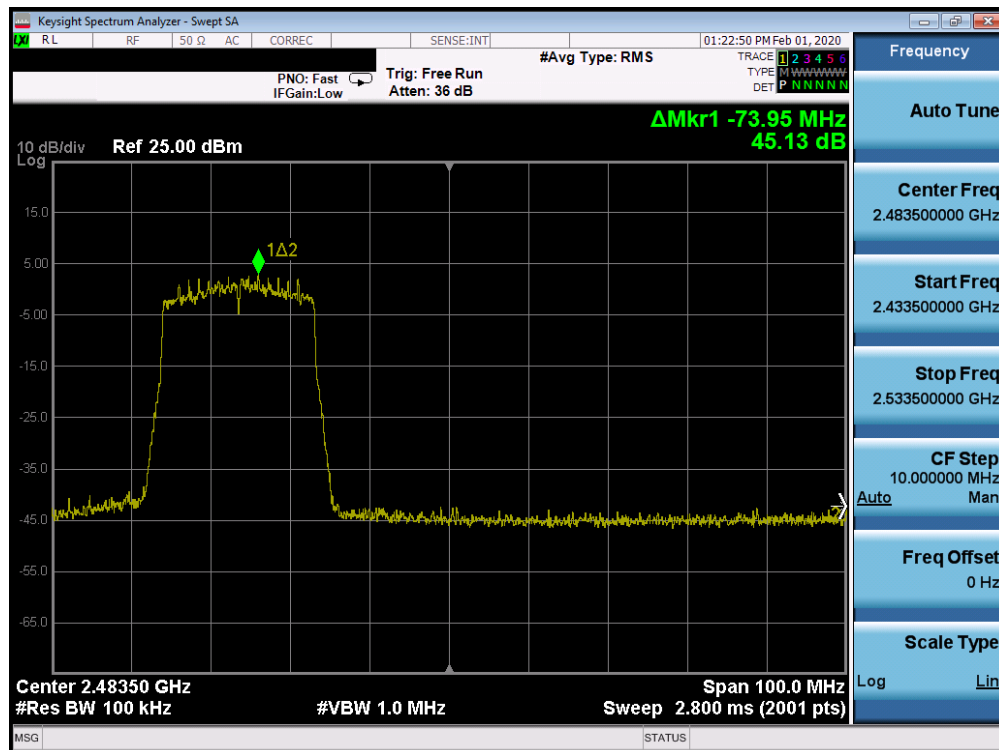
Plot 7-96. Band Edge SISO CORE 1 (802.11ax OFDMA – RU242 – Ch. 10)
