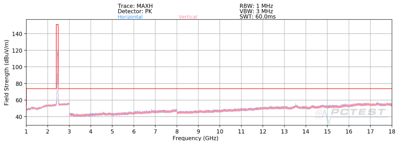
Plot 7-140. Radiated Spurious Plot above 1GHz CDD (802.11ax OFDMA – RU242 – Ch. 11)
