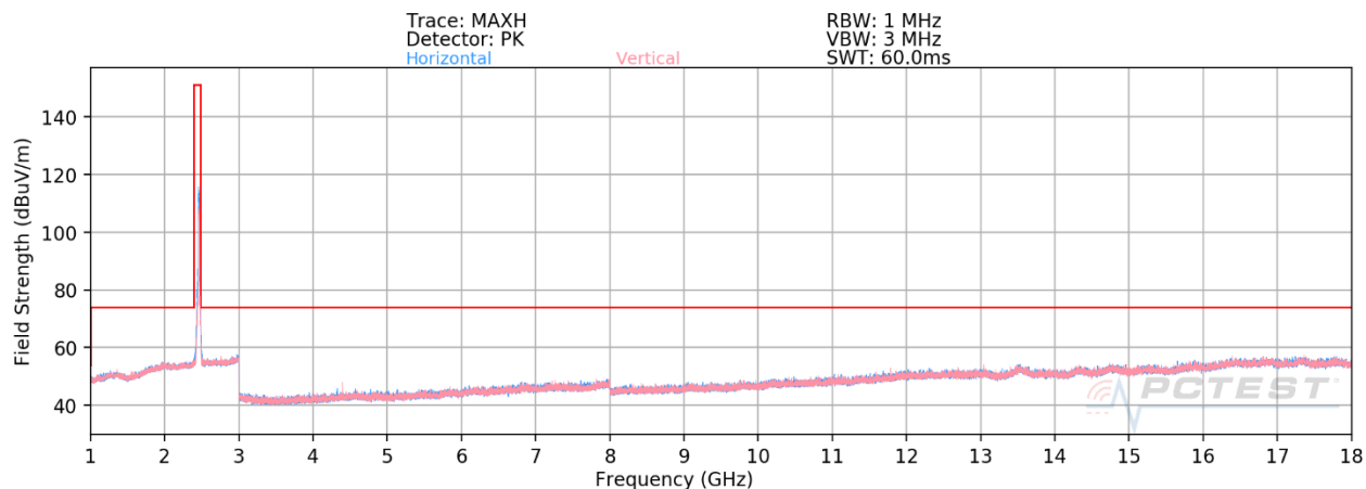
Plot 7-128. Radiated Spurious Plot above 1GHz SISO CORE 0 (802.11ax OFDMA – RU242 – Ch. 11)
