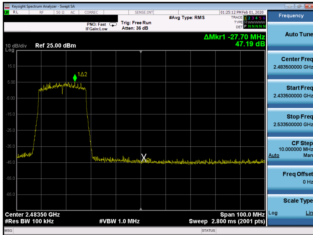
Plot 7-95. Band Edge SISO CORE 1 (802.11ax OFDMA – RU242 – Ch. 9)
