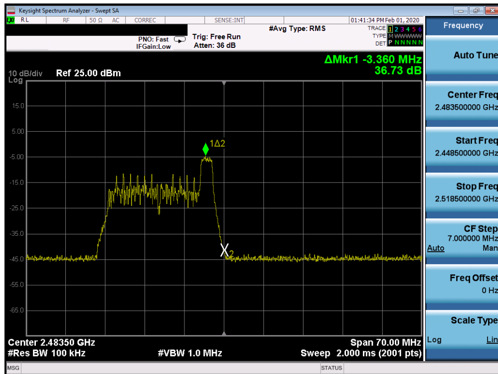
Plot 7-92. Band Edge SISO CORE 1 (802.11ax OFDMA – RU26 Index 8 – Ch. 12)
