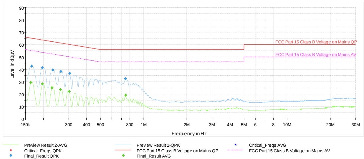
Plot 7-139. Line Conducted Plot with 802.11n CDD Ch.6 (N, with AC/DC Adapter)
