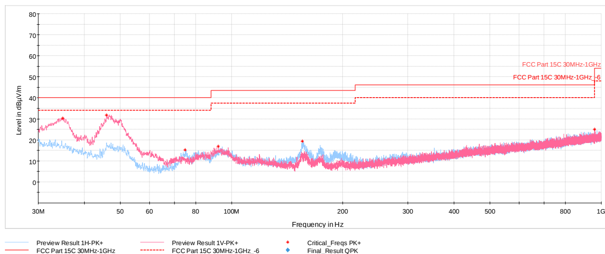
Plot 7-137. Radiated Spurious Plot below 1GHz CDD Ch.6, with AC/DC Adapter
