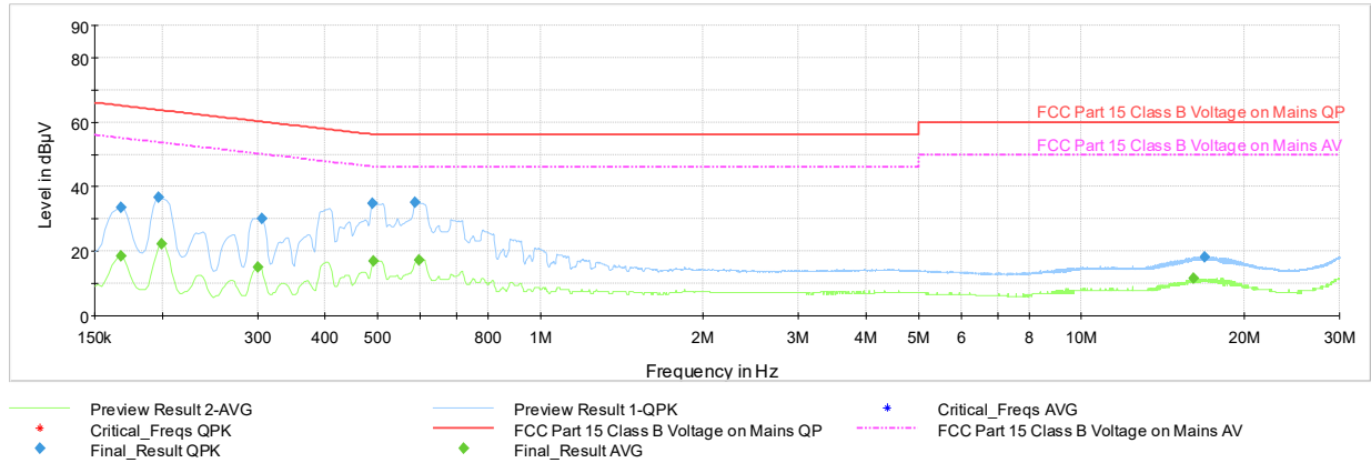
Plot 7-106. Line Conducted Plot with Bluetooth LE (N – 1Mbps, ePA, Ch.19 with AC/DC Adapter)
