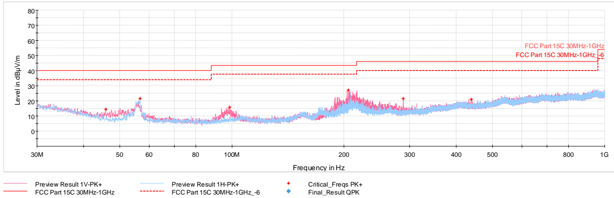
Plot 7-891. Radiated Spurious Plot below 1GHz CDD (802.11ax – RU26 – U3 Ch. 157) with Laptop
