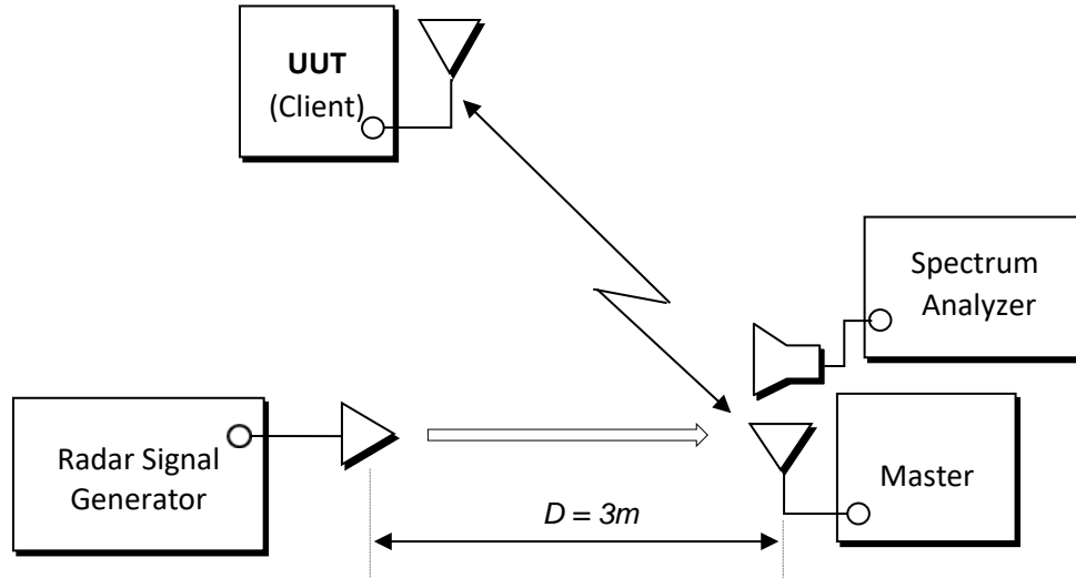
Figure 7-1. Radiated Test Setup for DFS
