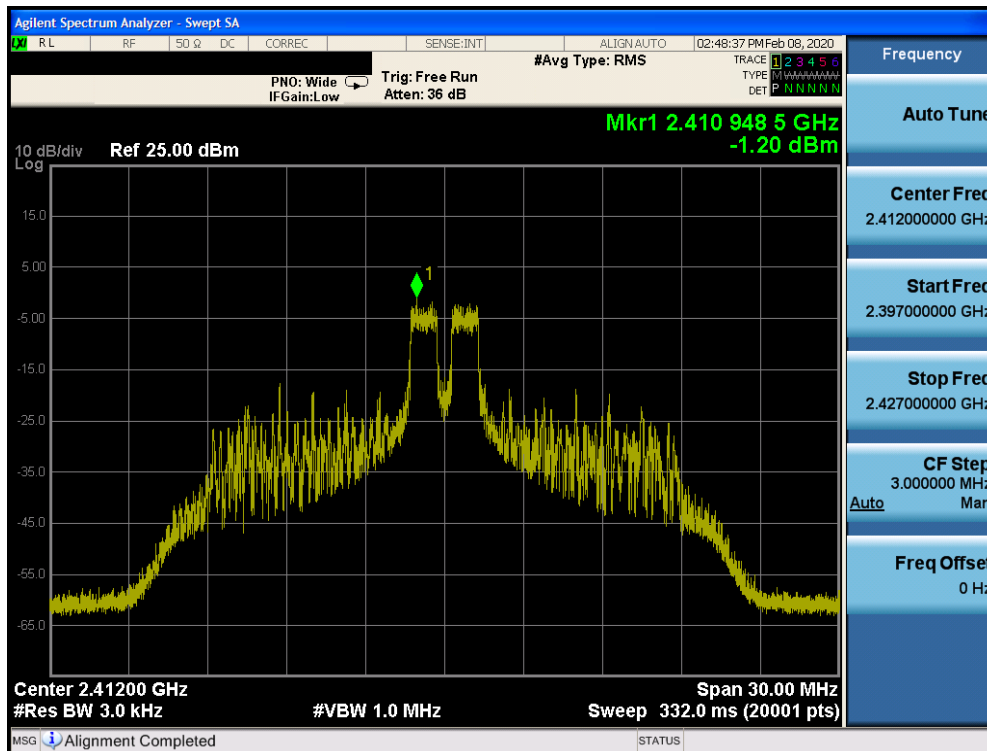
Plot 7-51. Power Spectral Density Plot CDD CORE 0 (802.11ax OFDMA – RU26 Index 4 – Ch. 1)
