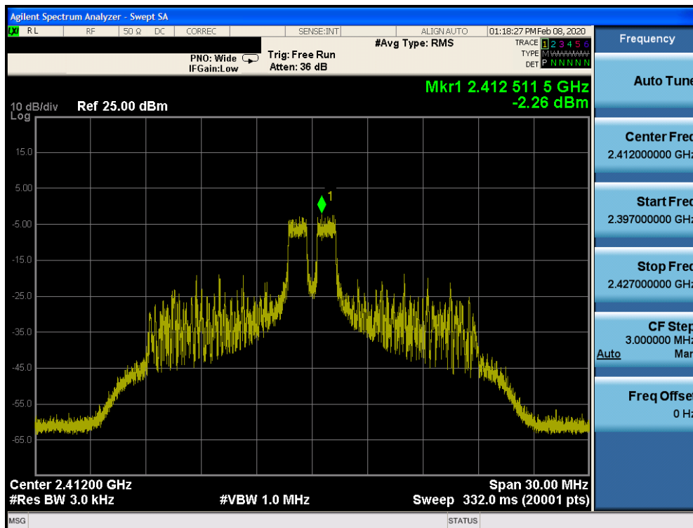
Plot 7-52. Power Spectral Density Plot CDD CORE 1 (802.11ax OFDMA – RU26 Index 4 – Ch. 1)
