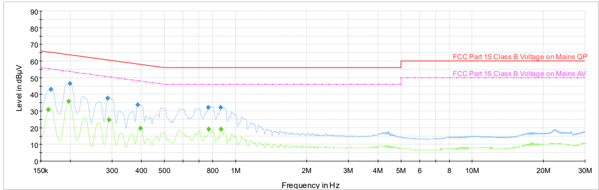
Plot 7-133. Line Conducted Plot with 802.11n CDD Ch.6 (N, with AC/DC Adapter)
