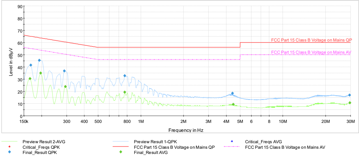
Plot 7-106. Line Conducted Plot with Bluetooth HDR (N, 4Mbps ePA – Ch.38 with AC/DC Adapter)
