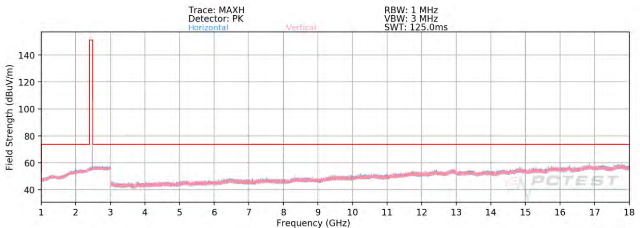
Plot 7-83. Radiated Spurious Plot Above 1GHz Ant WF8 (4Mbps, HDR4 ePA – Ch. 75, Ant. Pol. H & V)
