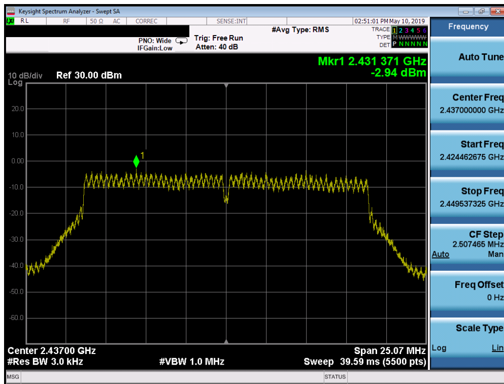
Plot 7-35. Power Spectral Density Plot SISO CORE 1 (802.11n (2.4GHz) – Ch. 6)
