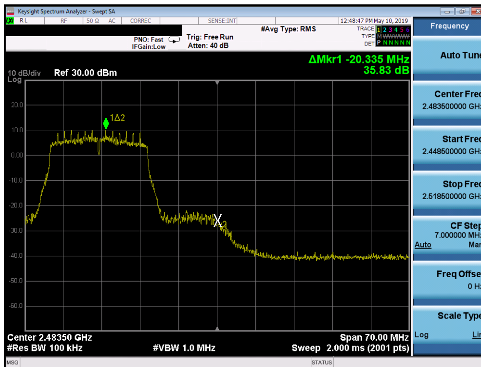
Plot 7-58. Band Edge Plot SISO CORE 0 (802.11n (2.4GHz) – Ch. 11)
