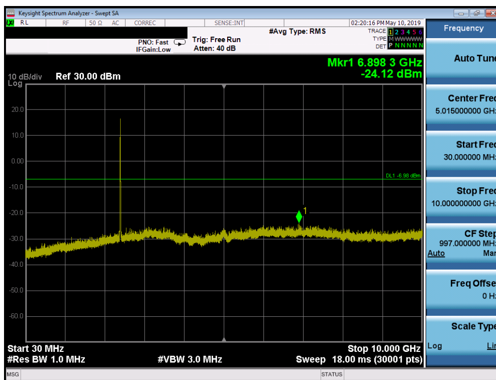
Plot 7-79. Conducted Spurious Plot SISO CORE 1 (802.11b – Ch. 1)
