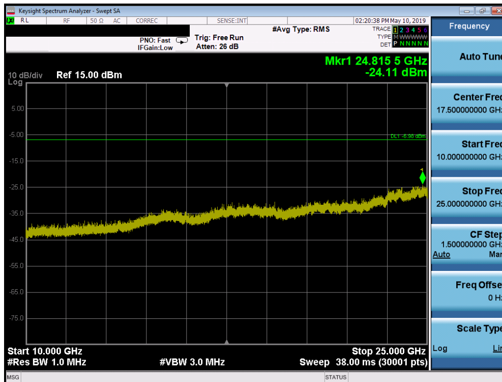
Plot 7-80. Conducted Spurious Plot SISO CORE 1 (802.11b – Ch. 1)
