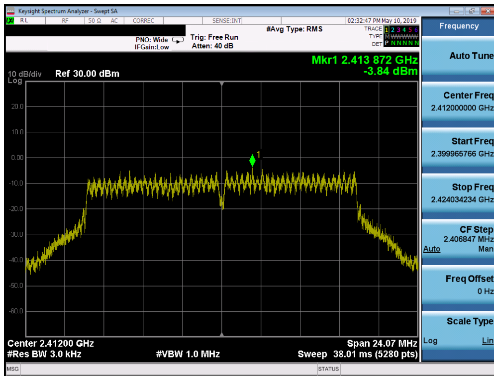
Plot 7-31. Power Spectral Density Plot SISO CORE 1 (802.11g – Ch. 1)
