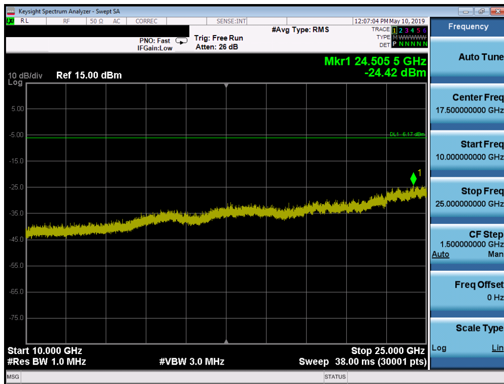
Plot 7-76. Conducted Spurious Plot SISO CORE 0 (802.11b – Ch. 6)
