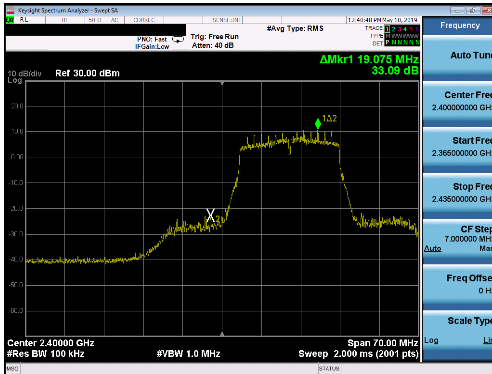
Plot 7-57. Band Edge Plot SISO CORE 0 (802.11n (2.4GHz) – Ch. 1)
