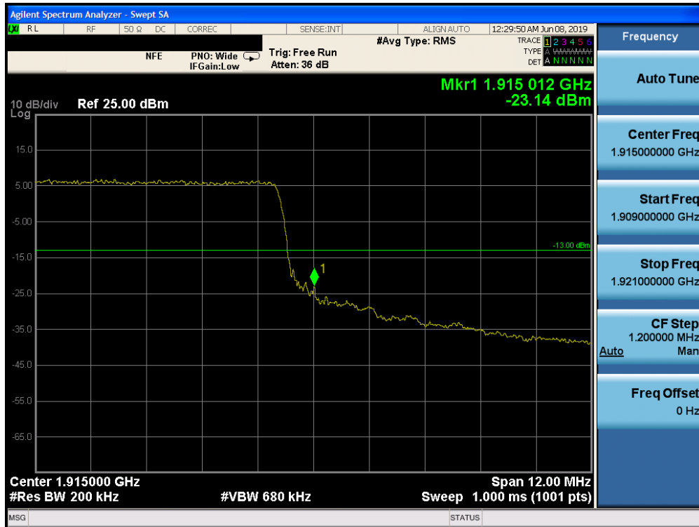
Plot 7-300. Upper Band Edge Plot (Band 25 - 15.0MHz QPSK - Full RB Configuration)
