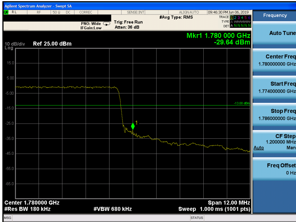
Plot 7-252. Upper Band Edge Plot (Band 66 - 15.0MHz QPSK - Full RB Configuration)
