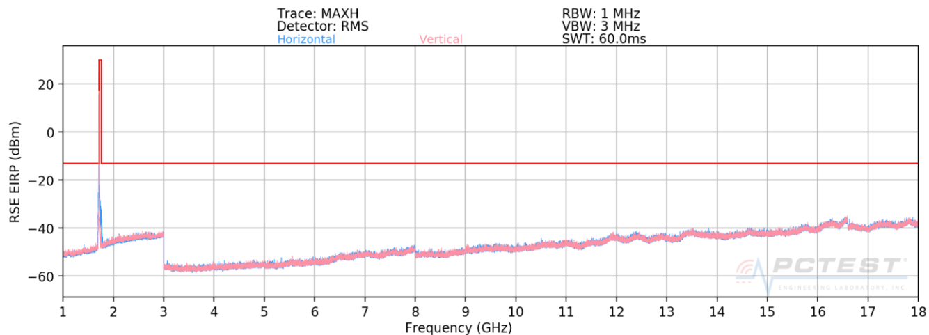
Plot 7-84. Radiated Spurious Plot above 1GHz (AWS WCDMA Mode)
