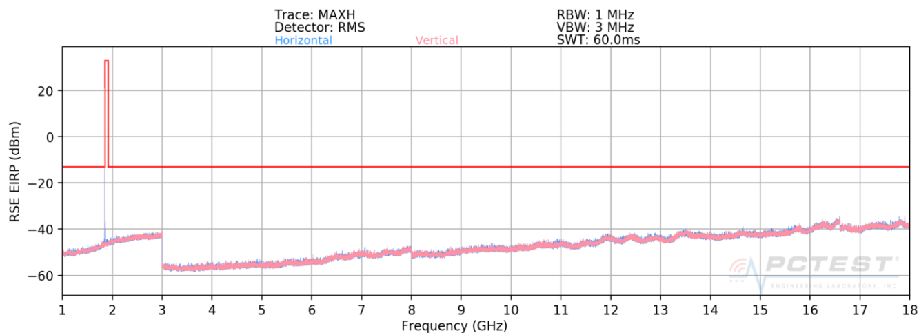
Plot 7-85. Radiated Spurious Plot above 1GHz (PCS GPRS Mode)
