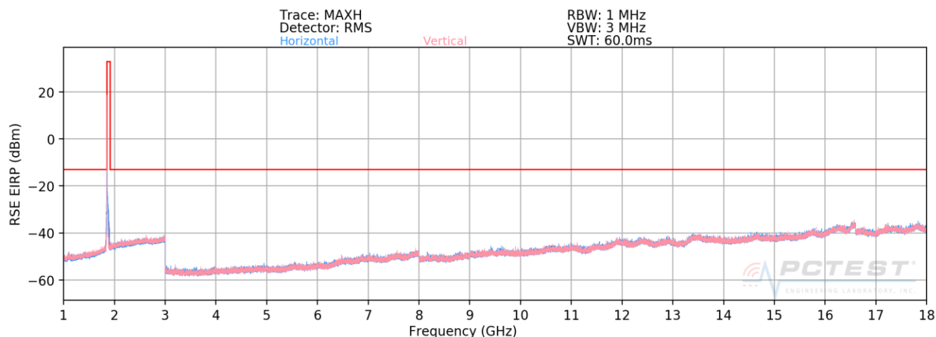
Plot 7-86. Radiated Spurious Plot above 1GHz (PCS WCDMA Mode)
