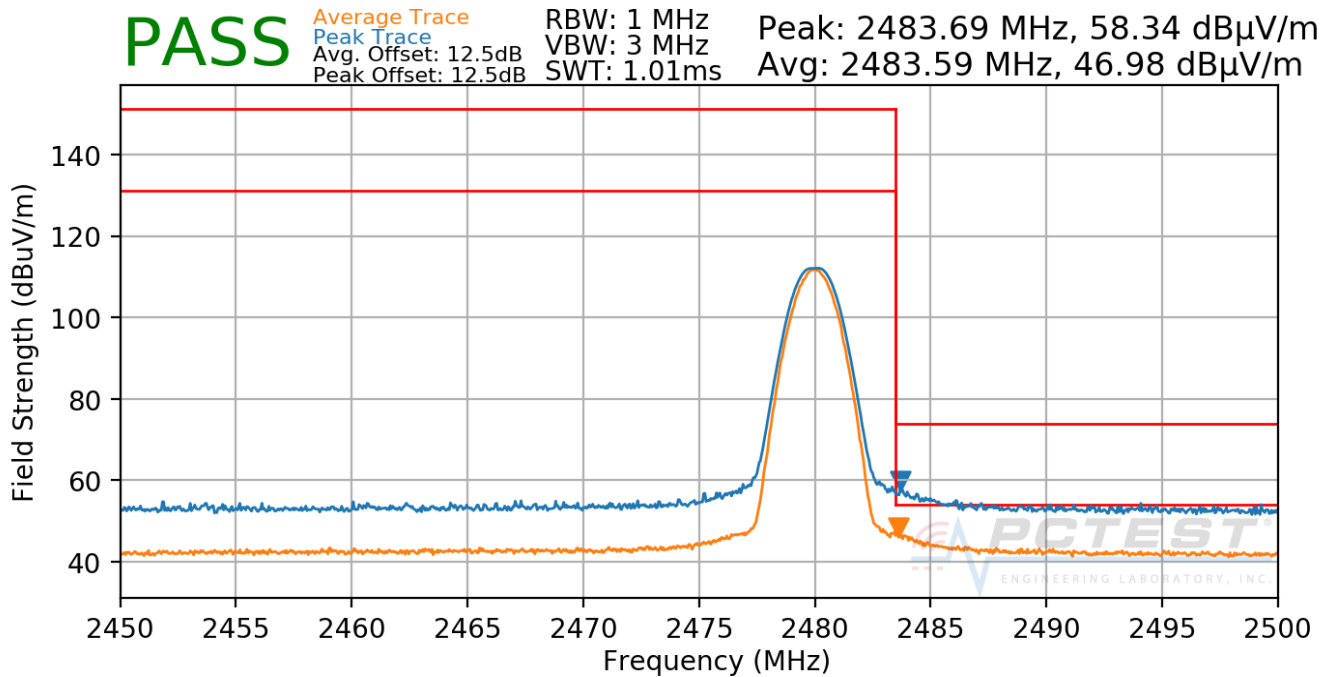
Plot 7-45. Radiated Restricted Upper Band Edge Measurement
