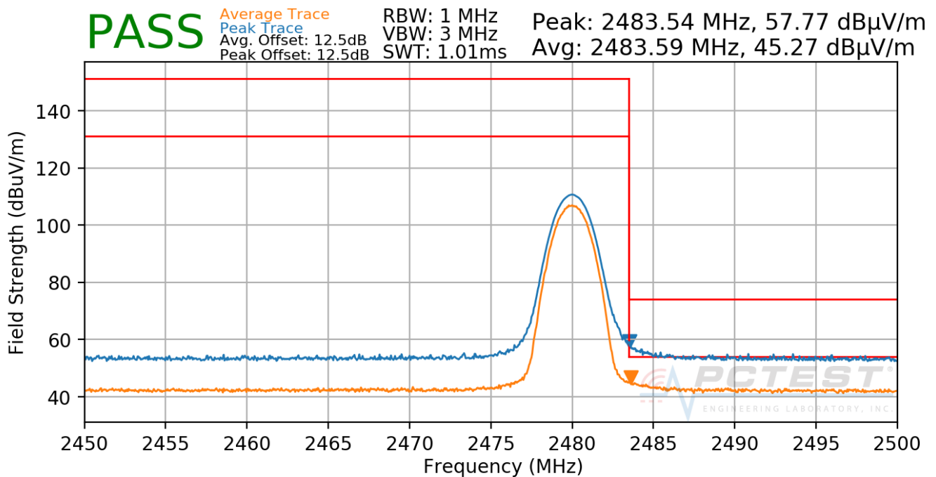
Plot 7-46. Radiated Restricted Upper Band Edge Measurement
