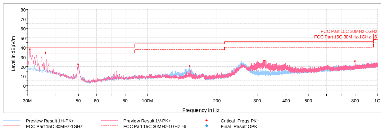
Plot 7-47. Radiated Spurious Plot below 1GHz GFSK ePA – Ch.39, with Laptop
