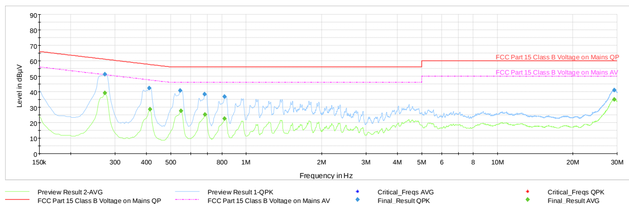
Plot 7-49. AC Line-Conducted Test Plot - Ch.39 (L1, with AC/DC Adapter)
