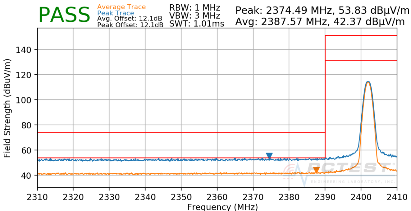
Plot 7-43. Radiated Restricted Lower Band Edge Measurement
