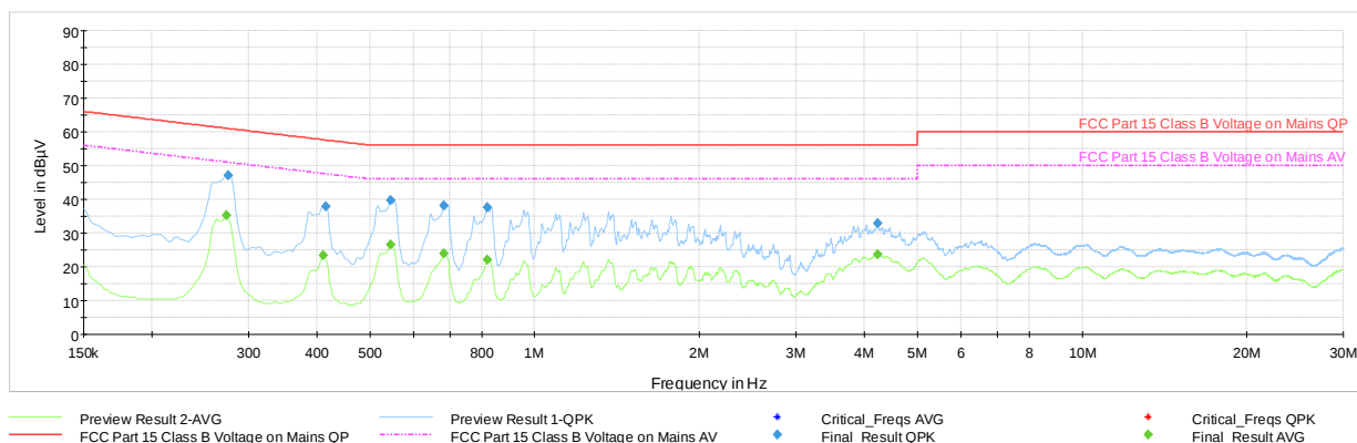
Plot 7-50. AC Line-Conducted Test Plot - Ch.39 (N, with AC/DC Adapter)
