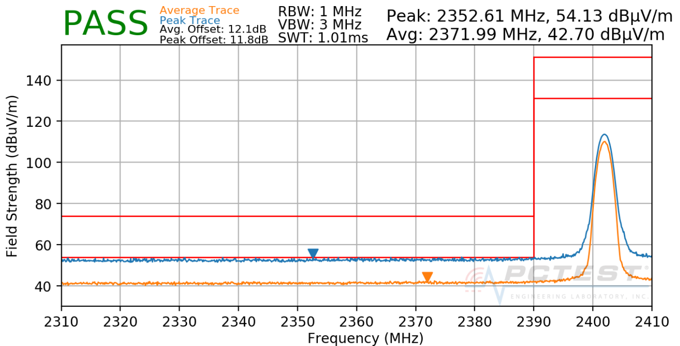
Plot 7-44. Radiated Restricted Lower Band Edge Measurement
