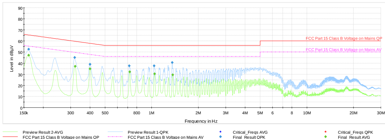
Plot 7-30. AC Line Conducted Plot with Bluetooth LE (N, with Laptop)
