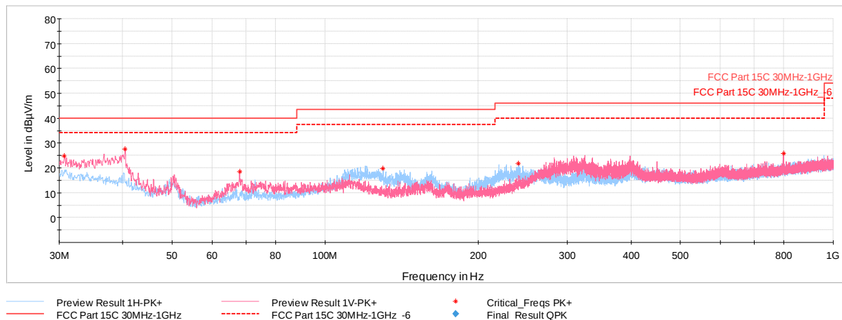
Plot 7-28. Radiated Spurious Plot below 1GHz (ePA – Ch.39, Pol. H & V, with Laptop)
