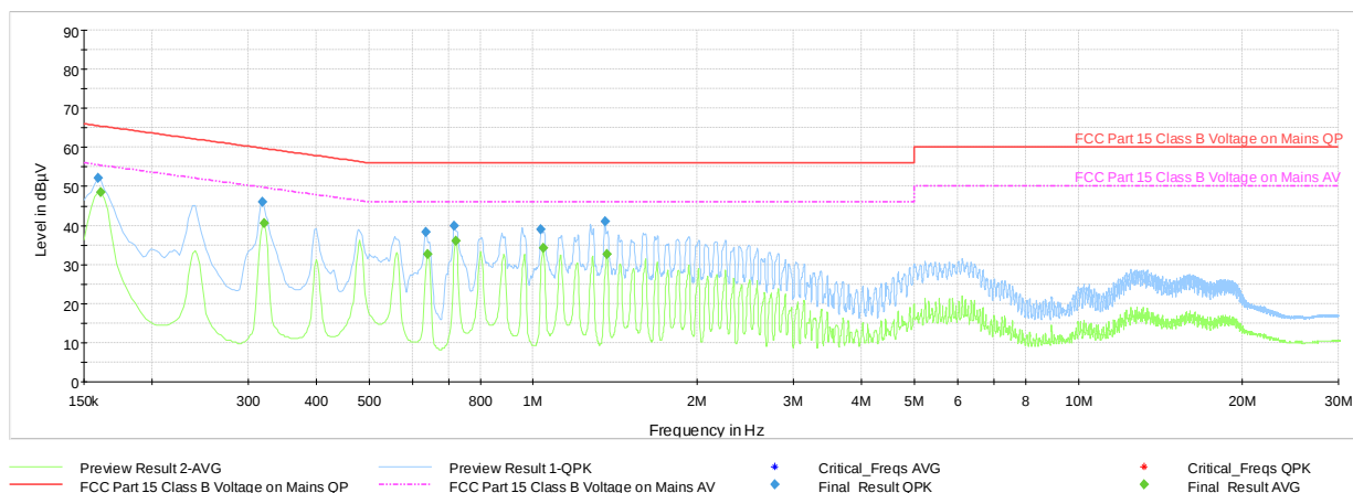
Plot 7-29. AC Line Conducted Plot with Bluetooth LE (L1, with Laptop)
