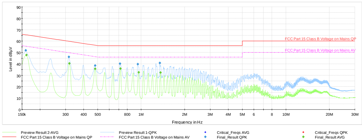
Plot 7-286. AC Line Conducted Plot with 802.11n UNII Band 1 – Ch.36 (L1), with Laptop
