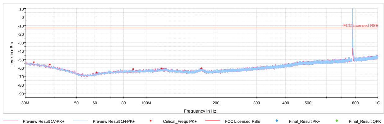
Plot 7-452. Radiated Spurious Plot below 1GHz with AC/DC Adapter (Band 13)
