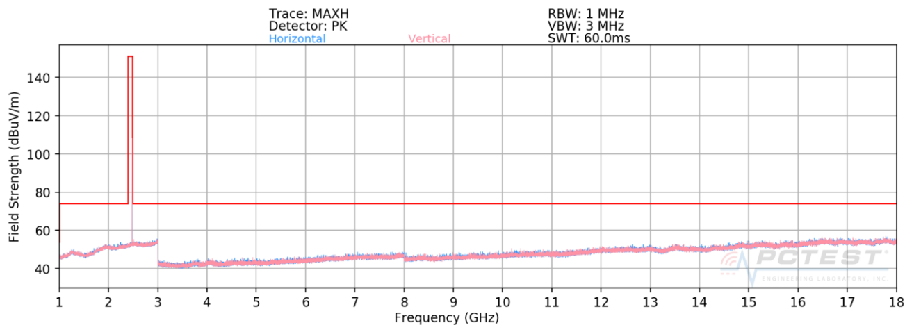
Plot 7-37. Radiated Spurious Plot above 1GHz (BT GFSK ePA – Ch. 78)
