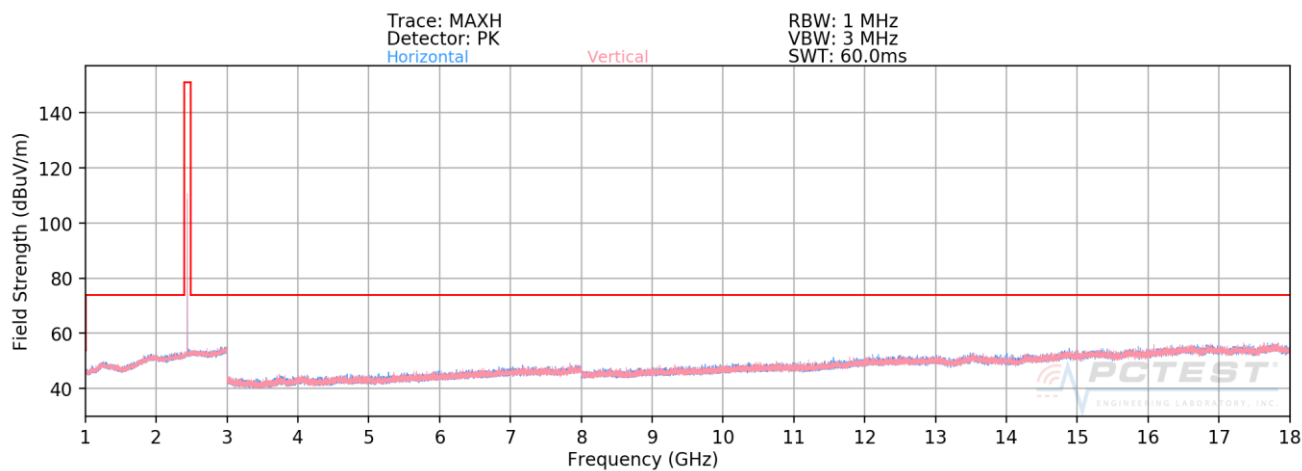
Plot 7-36. Radiated Spurious Plot above 1GHz (BT GFSK ePA – Ch. 39)
