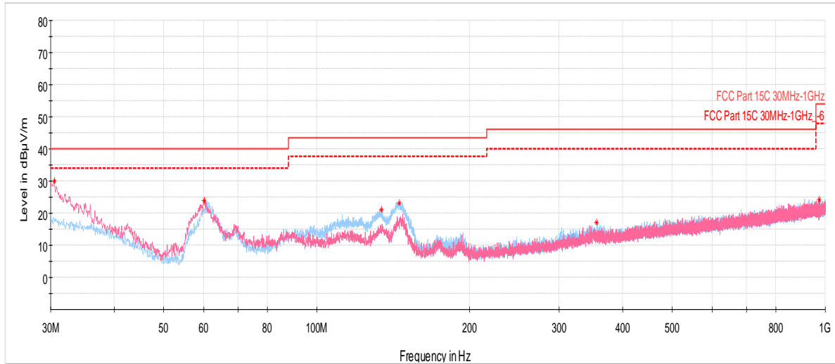
Plot 7-28. Radiated Spurious Plot below 1GHz (ePA – Ch.39, Pol. H & V, with AC/DC Adapter)
