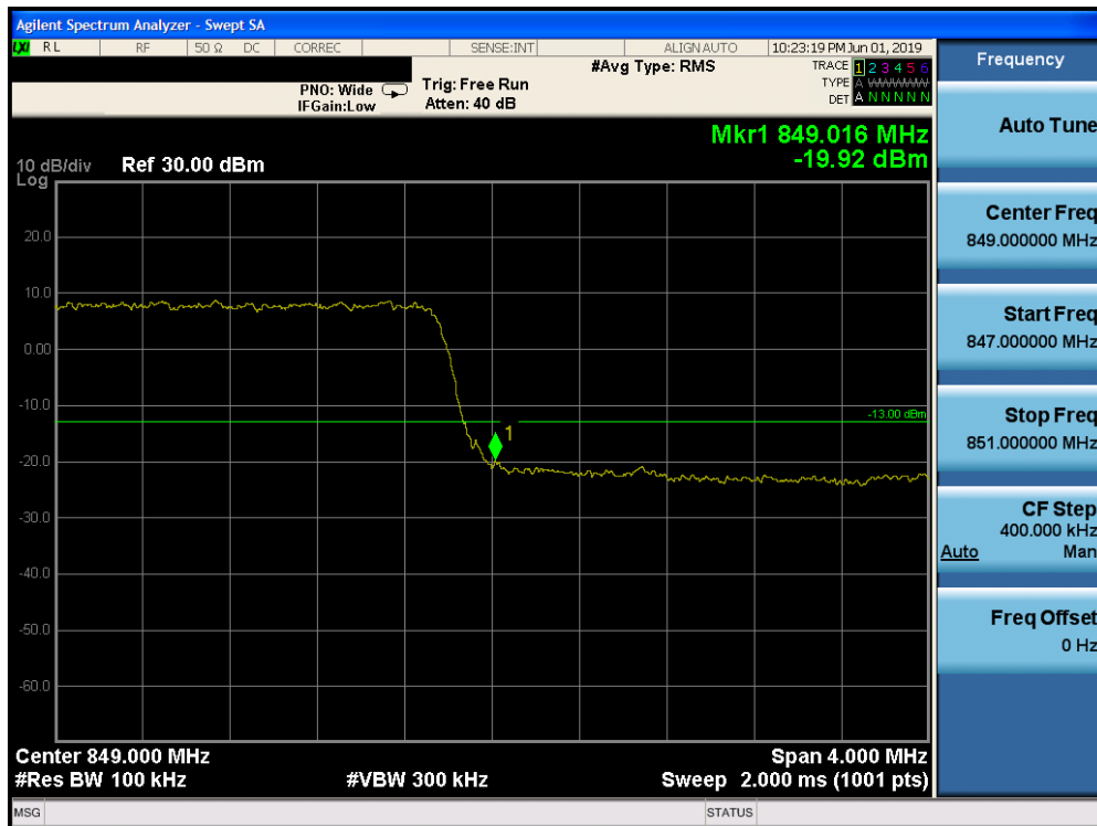
Plot 7-198. Upper Band Edge Plot (Band 5 - 5.0MHz QPSK - Full RB Configuration)
