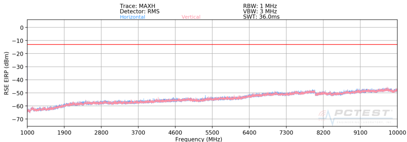
Plot 7-46. Radiated Spurious Plot above 1GHz (Band 26)
