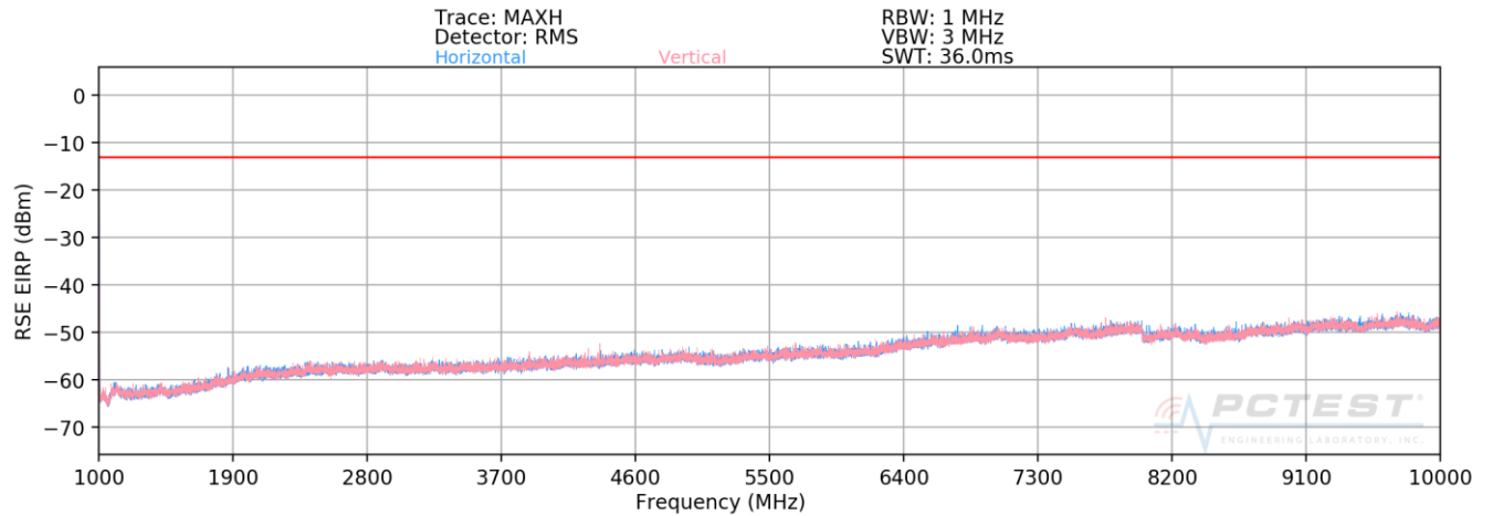
Plot 7-47. Radiated Spurious Plot above 1GHz (Band 14)
