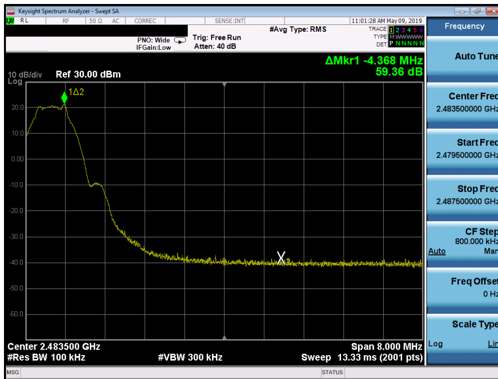
Plot 7-14. Band Edge Plot (Bluetooth (LE), ePA – Ch. 39)
