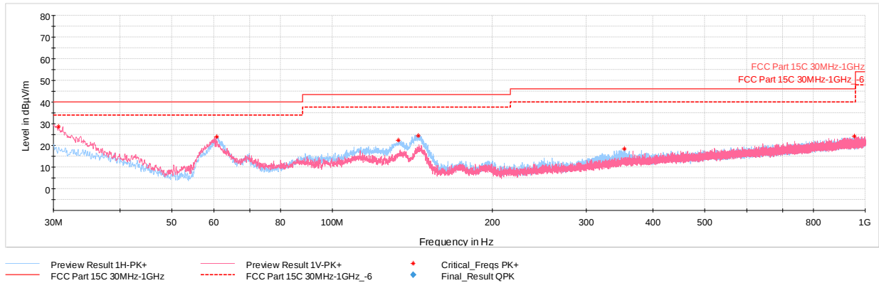
Plot 7-28. Radiated Spurious Plot below 1GHz (ePA – Ch.39, Pol. H & V, with AC/DC Adapter)
