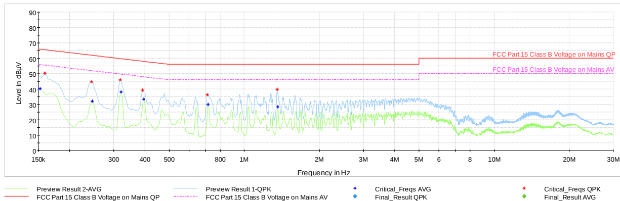
Plot 7-30. AC Line Conducted Plot with Bluetooth LE (N, with Laptop)
