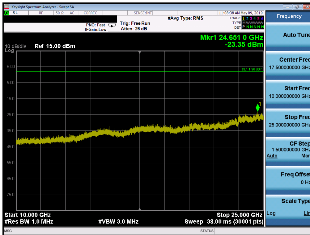
Plot 7-16. Conducted Spurious Plot (Bluetooth (LE), ePA – Ch. 0)
