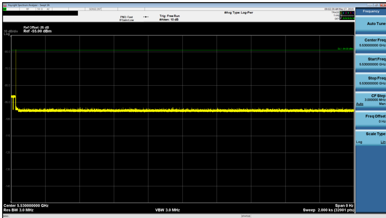
Figure 9-39. 5530MHz - Non-Occupancy Period (30 Minutes) - Mode 1 (80MHz)
