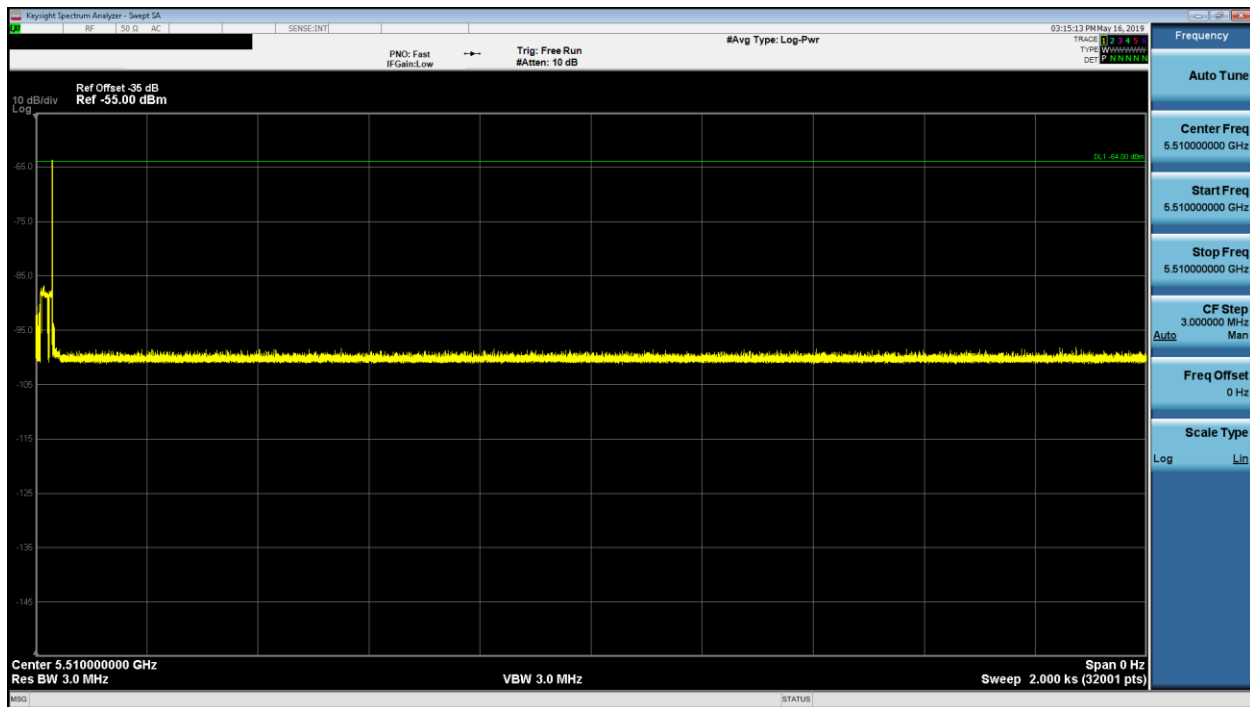
Figure 9-38. 5510MHz - Non-Occupancy Period (30 Minutes) - Mode 1 (40MHz)
