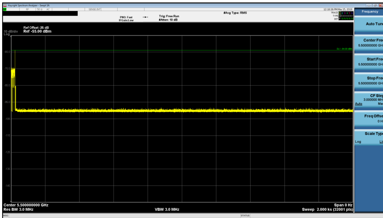
Figure 9-46. 5500MHz - Non-Occupancy Period (30 Minutes) - Mode 4 (20MHz)
