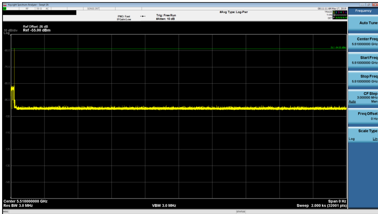
Figure 9-41. 5510MHz - Non-Occupancy Period (30 Minutes) - Mode 2 (40MHz)
