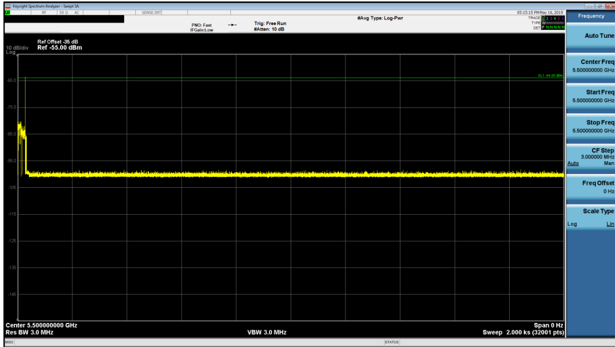
Figure 9-40. 5500MHz - Non-Occupancy Period (30 Minutes) - Mode 2 (20MHz)
