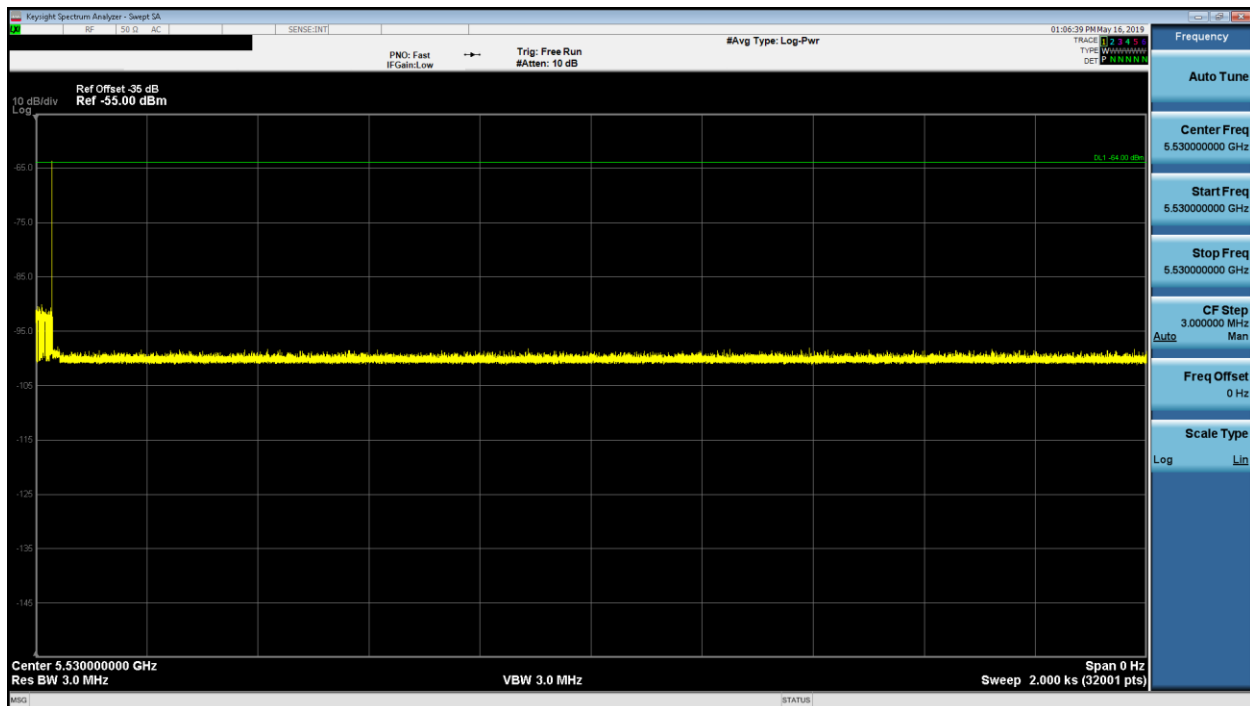
Figure 9-45. 5530MHz - Non-Occupancy Period (30 Minutes) - Mode 3 (80MHz)
