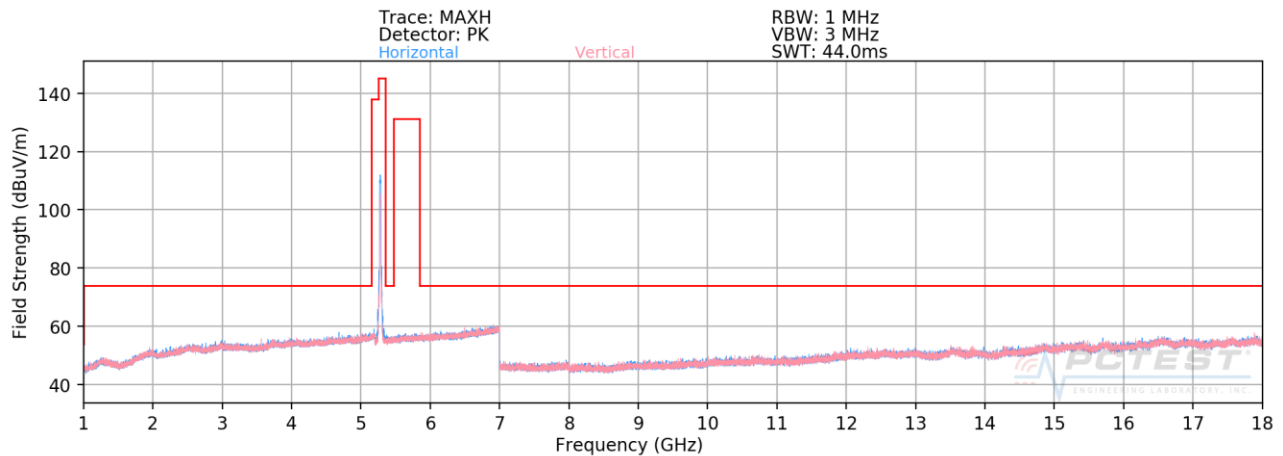
Plot 7-187. Radiated Spurious Plot above 1GHz SISO CORE 1 (802.11n – U2A Ch. 56)
