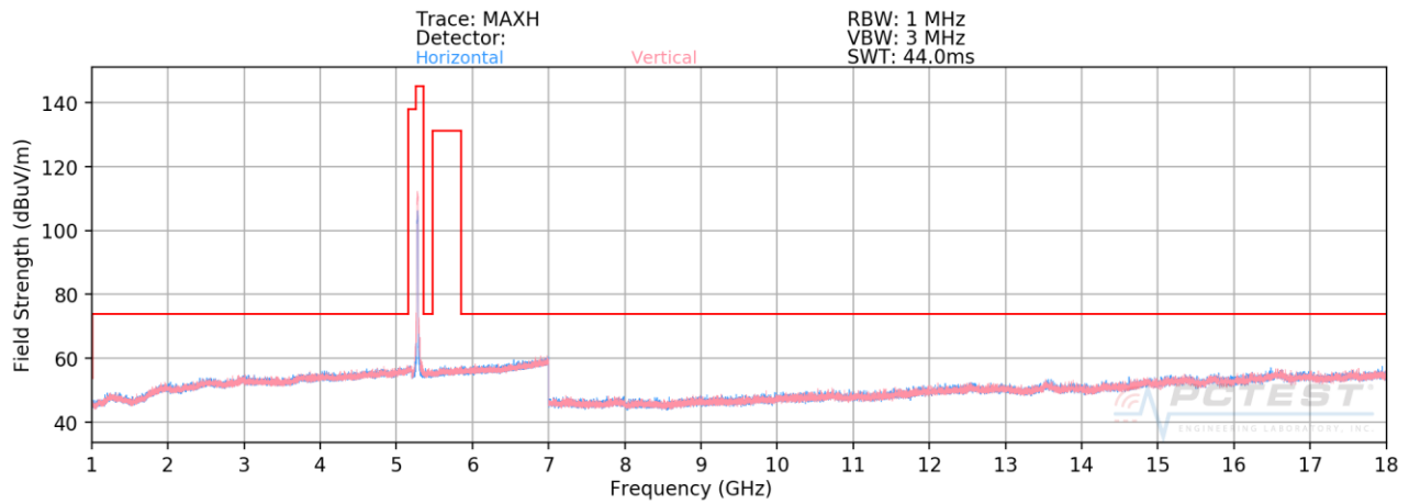
Plot 7-175. Radiated Spurious Plot above 1GHz SISO CORE0 (802.11n – U2A Ch. 56)
