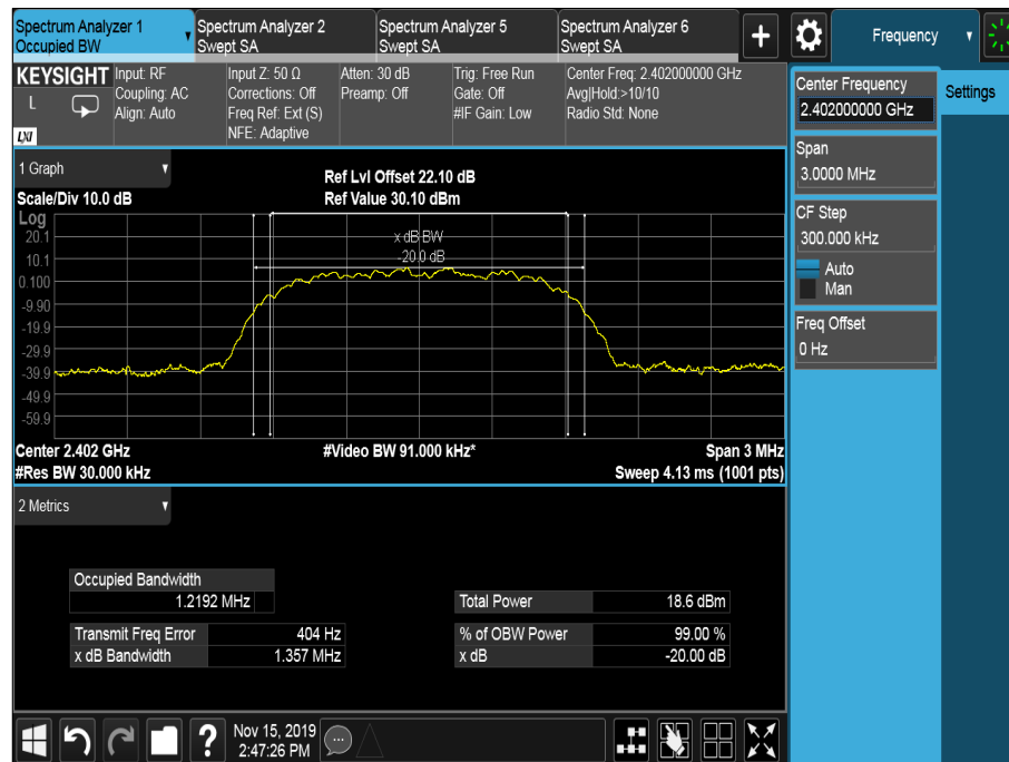
Figure 3 - 2402 MHz - 8-DPSK
