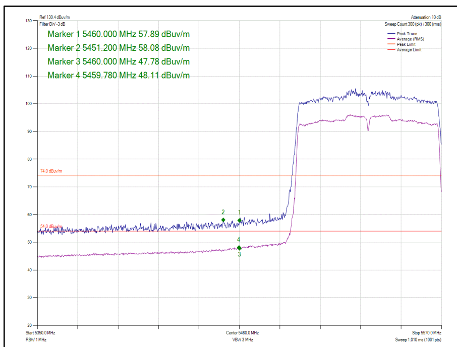
Figure 442 - 802.11ac VHT80 Core 1 - 5530 MHz Band Edge Frequency 5460 MHz
