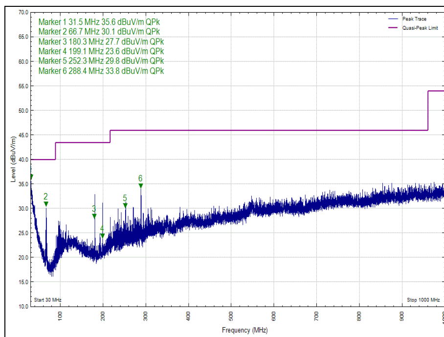
Figure 449 - U-NII 1 - 5180 MHz - 30 MHz to 1 GHz - Polarity: Horizontal (Peak)
