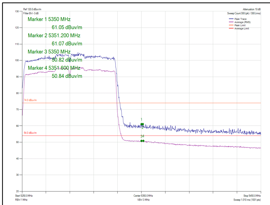
Figure 441 - 802.11ac VHT80 Core 1 - 5290 MHz Band Edge Frequency 5350 MHz
