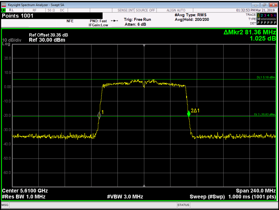
Figure 257 - 5610 MHz - 26 dB Emission Bandwidth
