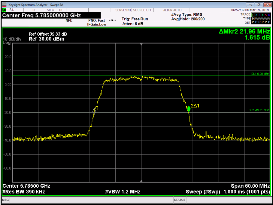
Figure 316 - 5785 MHz - 26 dB Emission Bandwidth
