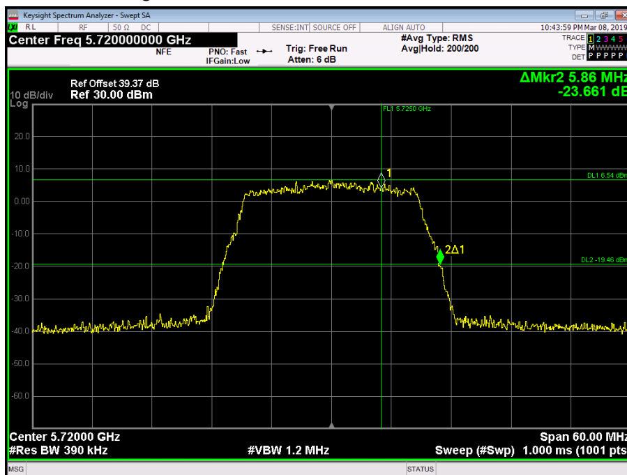
Figure 286 - 5720 MHz - 26 dB Emission Bandwidth
