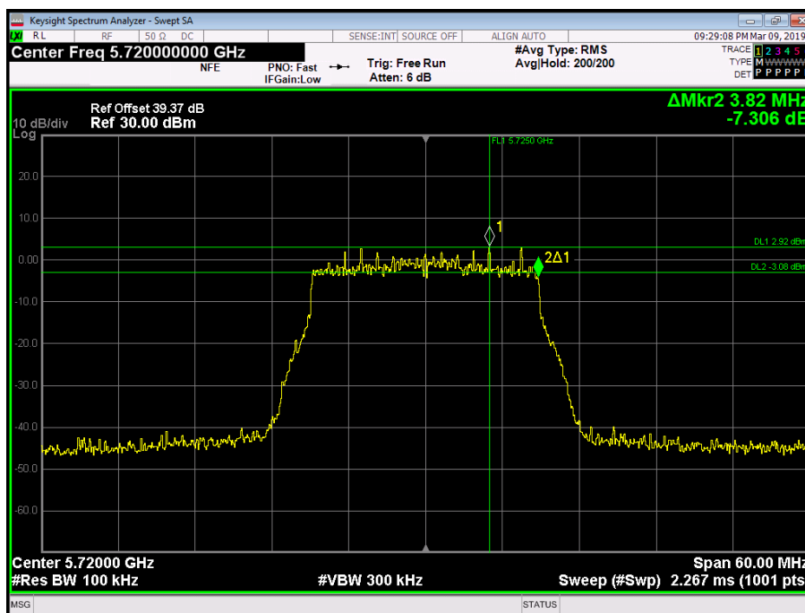
Figure 297 - 5720 MHz - 6 dB DTS Bandwidth
