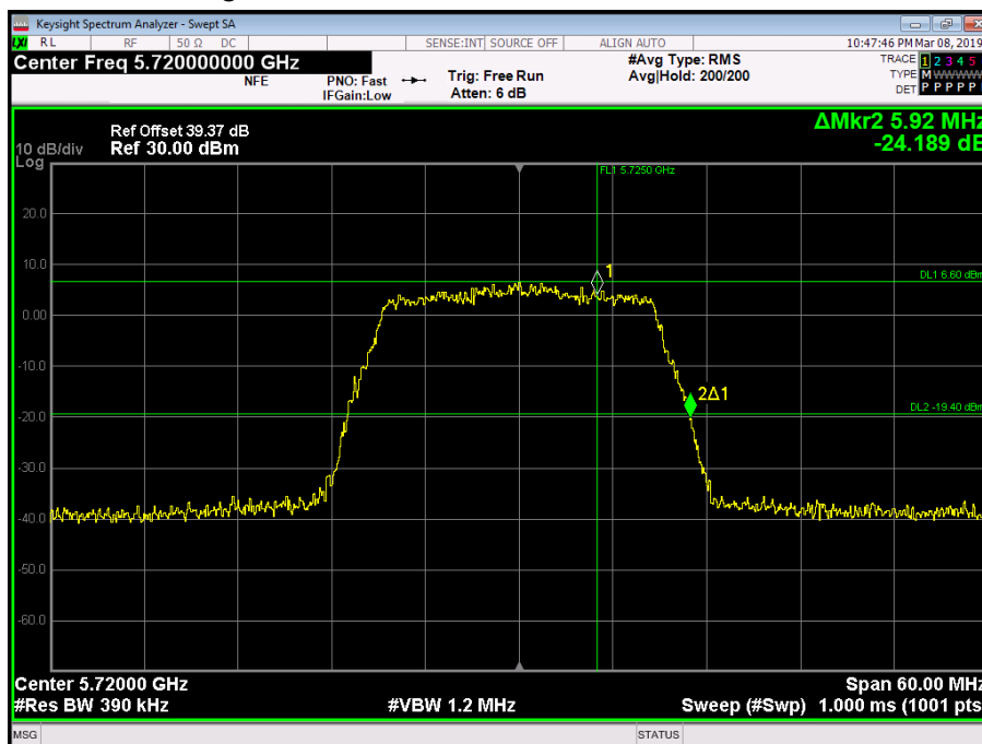
Figure 298 - 5720 MHz - 26 dB Emission Bandwidth
