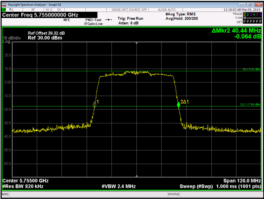
Figure 325 - 5755 MHz - 26 dB Emission Bandwidth
