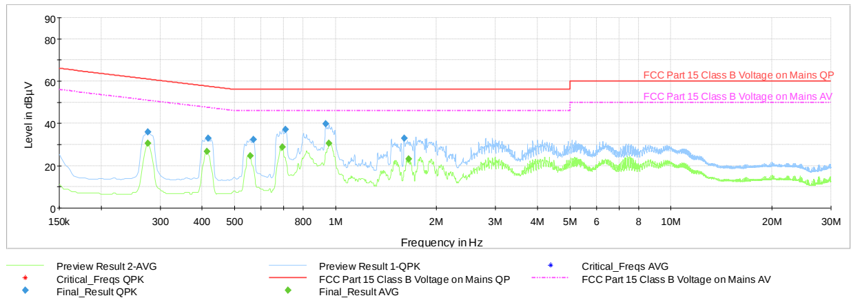
Plot 7-91. AC Line-Conducted Test Plot – Ch.39 (N, with AC/DC Adapter)
