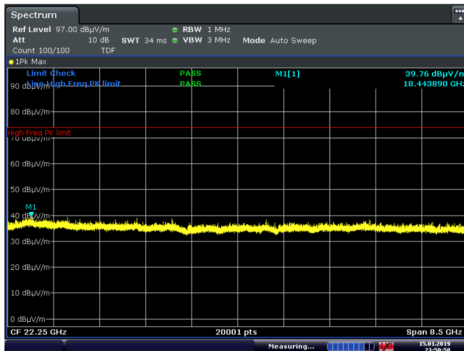
Plot 7-75. Radiated Spurious Plot above 18GHz (GFSK ePA – Ch. 78, Pol. H)
