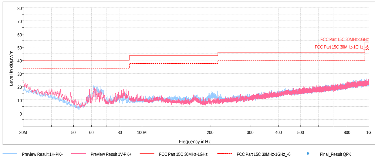
Plot 7-88. Radiated Spurious Plot below 1GHz GFSK ePA – Ch.39, with Laptop
