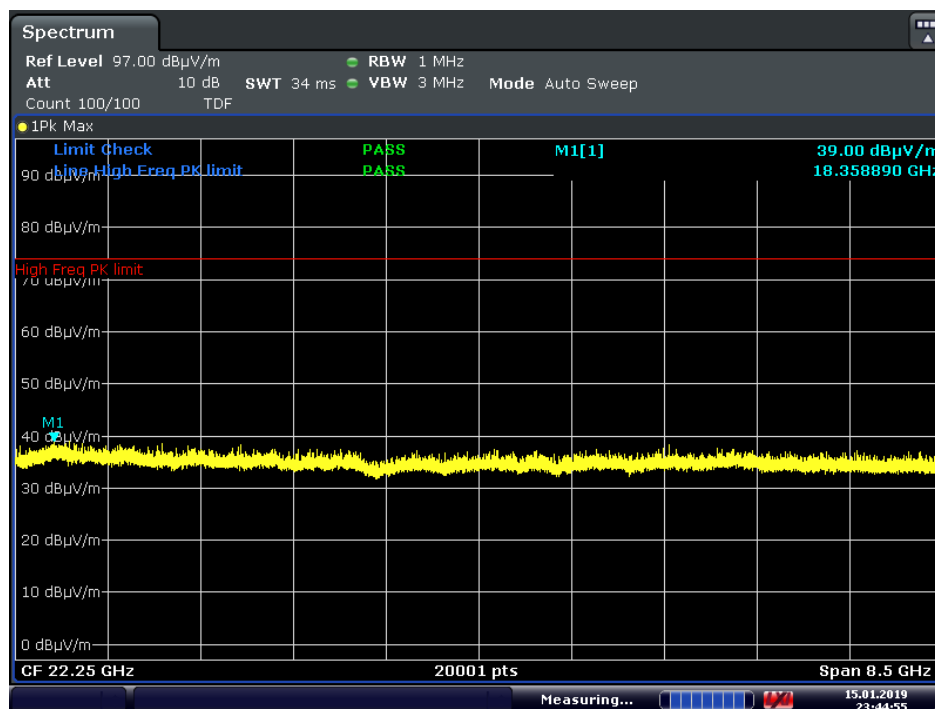
Plot 7-76. Radiated Spurious Plot above 18GHz (GFSK ePA – Ch. 78, Pol. V)
