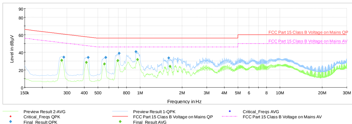
Plot 7-90. AC Line-Conducted Test Plot – Ch.39 (L1, with AC/DC Adapter)
