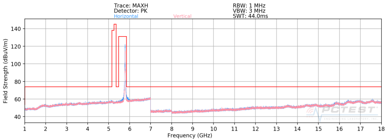
Plot 7-204. Radiated Spurious Plot above 1GHz MIMO/CDD (802.11n – U3 Ch. 157)
