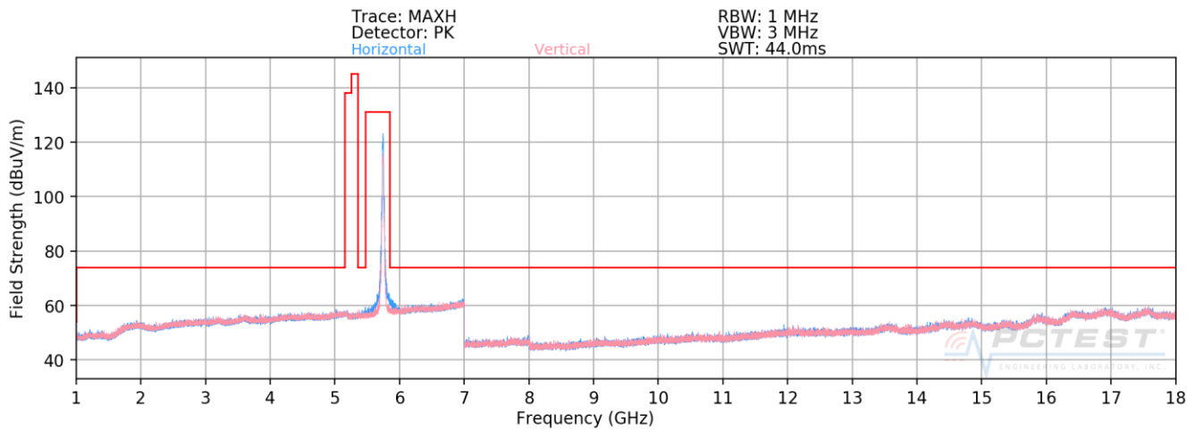
Plot 7-203. Radiated Spurious Plot above 1GHz MIMO/CDD (802.11n – U3 Ch. 149)
