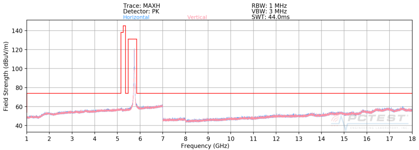
Plot 7-179. Radiated Spurious Plot above 1GHz SISO CORE0 (802.11n – U3 Ch. 149)
