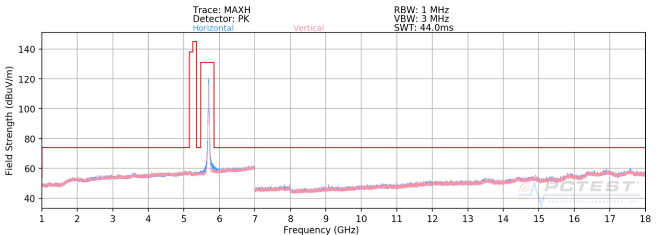
Plot 7-178. Radiated Spurious Plot above 1GHz SISO CORE0 (802.11n – U2C Ch. 144)
