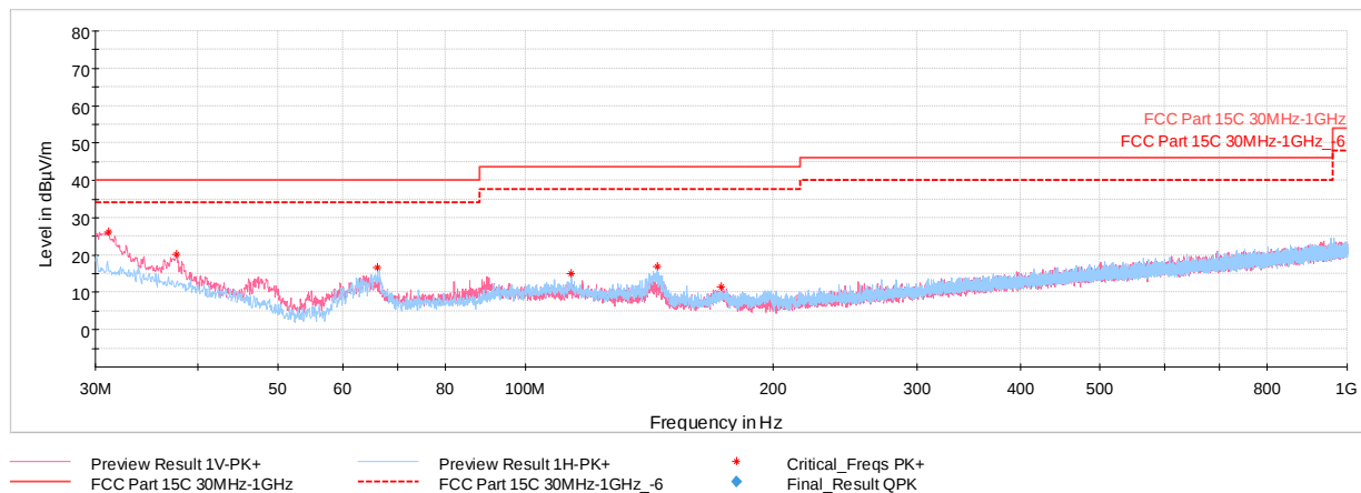
Plot 7-73. Radiated Spurious Plot below 1GHz (1Mbps, ePA – Ch.0, Pol. H & V, with AC/DC Adapter)
