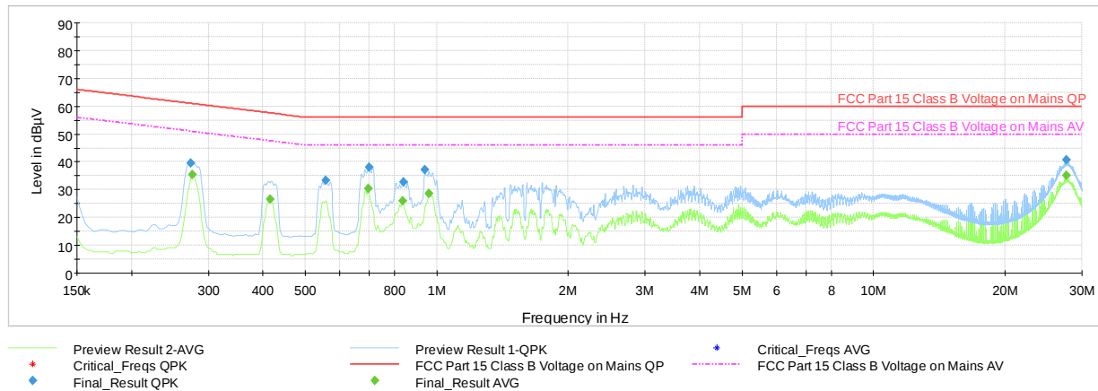
Plot 7-75. AC Line Conducted Plot with Bluetooth LE – 1Mbps ePA Ch.19 (N, with AC/DC Adapter)
