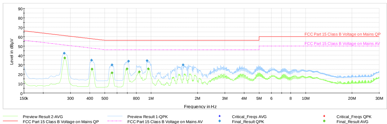
Plot 7-74. AC Line Conducted Plot with Bluetooth LE – 1Mbps ePA Ch.19 (L1, with AC/DC Adapter)
